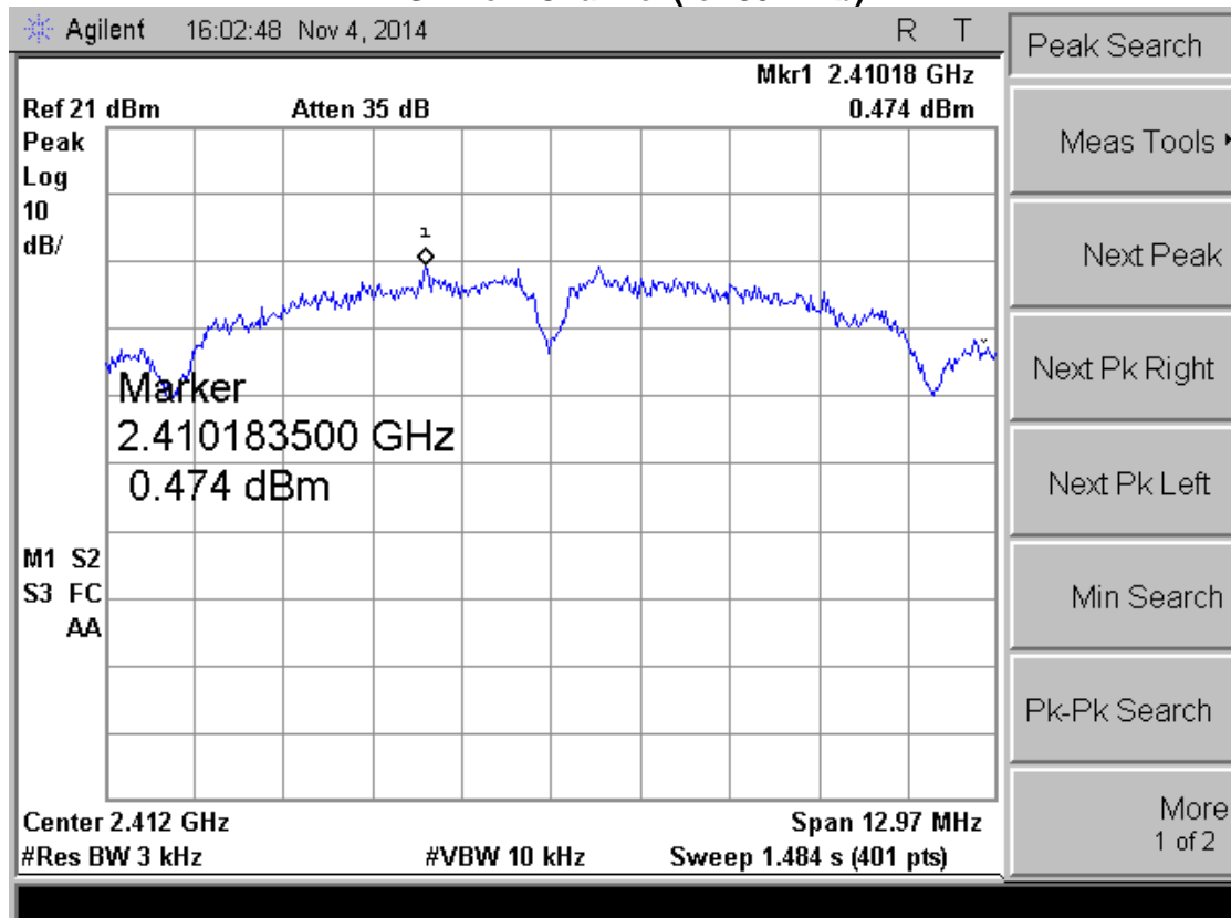
PSD-Low Channel (for 802.11b)
