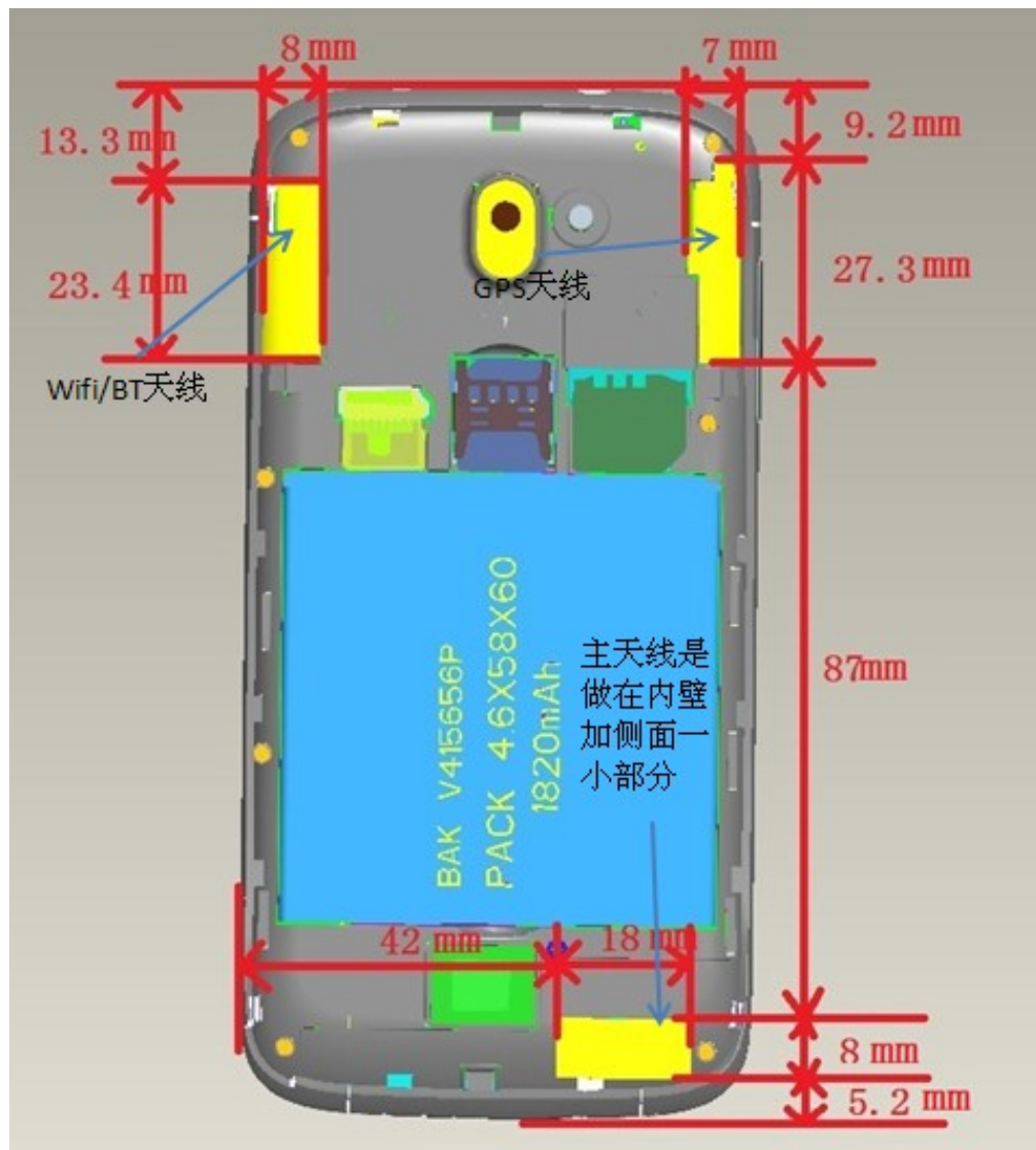
c: Antenna
