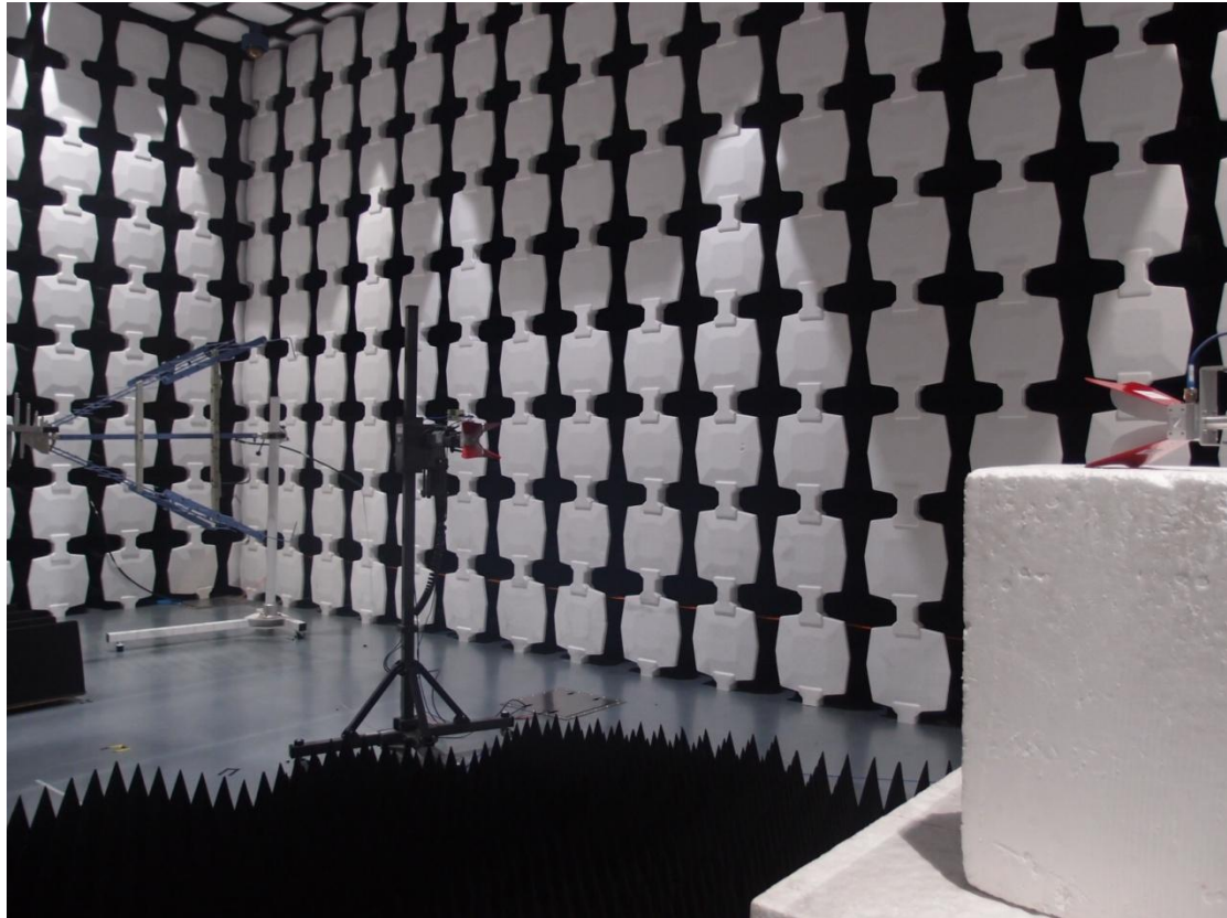
Description: Substitution Antenna for EIRP Test
