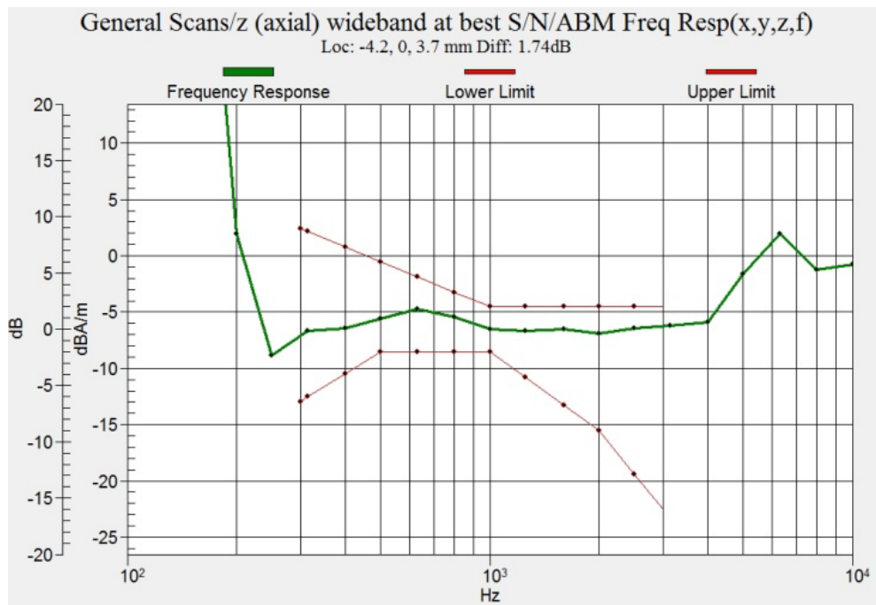
Figure C.5 Frequency Response of WCDMA 1900
