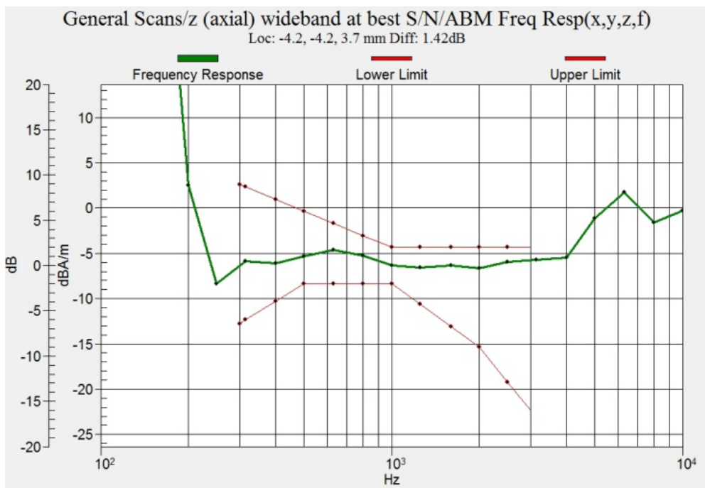
Figure C.4 Frequency Response of WCDMA 1700
