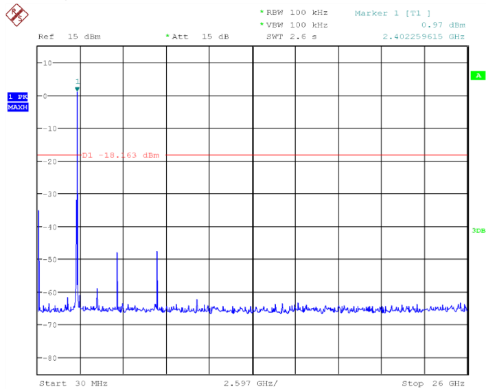
Fig.51 Conducted Spurious Emission (802.11b, Ch1)
