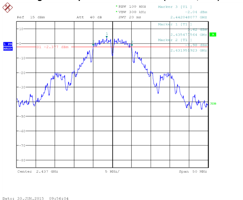
Fig.14 Occupied 6dB Bandwidth (802.11b, Ch6)
