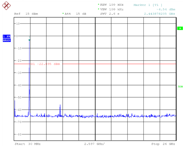
Fig.55 Conducted Spurious Emission (802.11b, Ch11)
