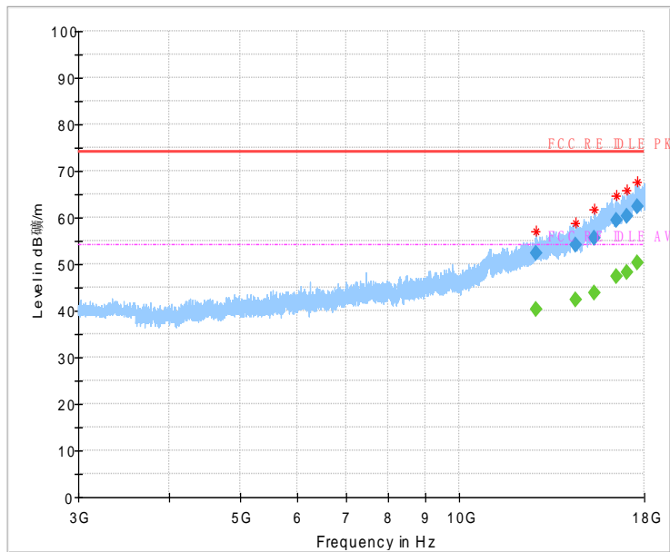
Fig.58 Radiated Spurious Emission (802.11 n-20MHz,Ch1,3GHz~18GHz)
