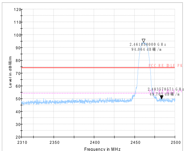
Fig.45 Radiated emission (Power): 802.11b, high channel
