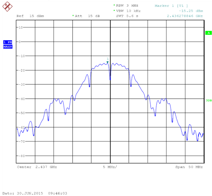
Fig.2 Power Spectral Density (802.1b,Ch6)
