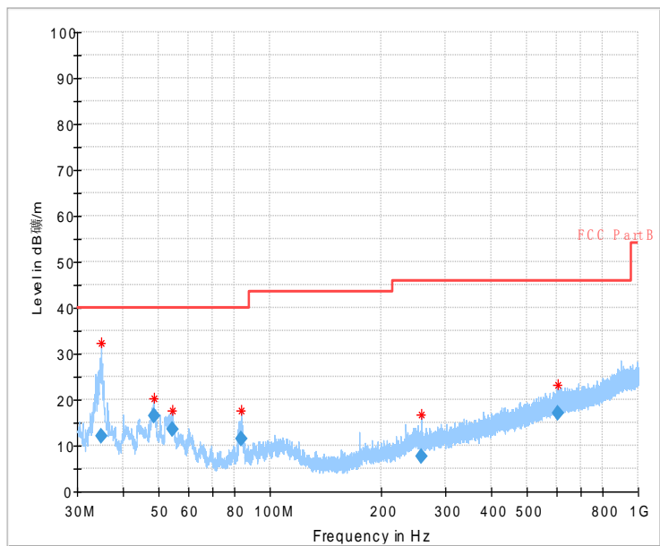
Fig.56 Radiated Spurious Emission (802.11 n-20MHz,Ch1,30MHz~1GHz)
