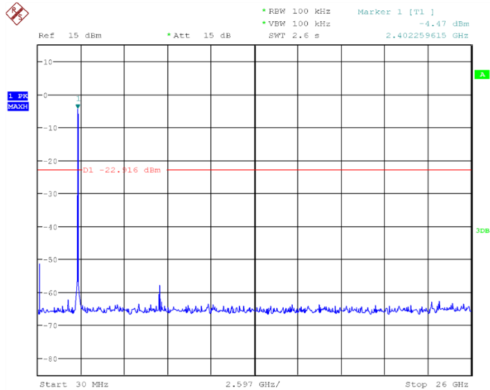
Fig.65 Conducted Spurious Emission (802.11n-20MHz, Ch6)
