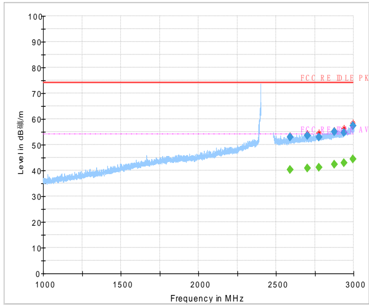
Fig.57 Radiated Spurious Emission (802.11 n-20MHz,Ch1,1GHz~3GHz)
