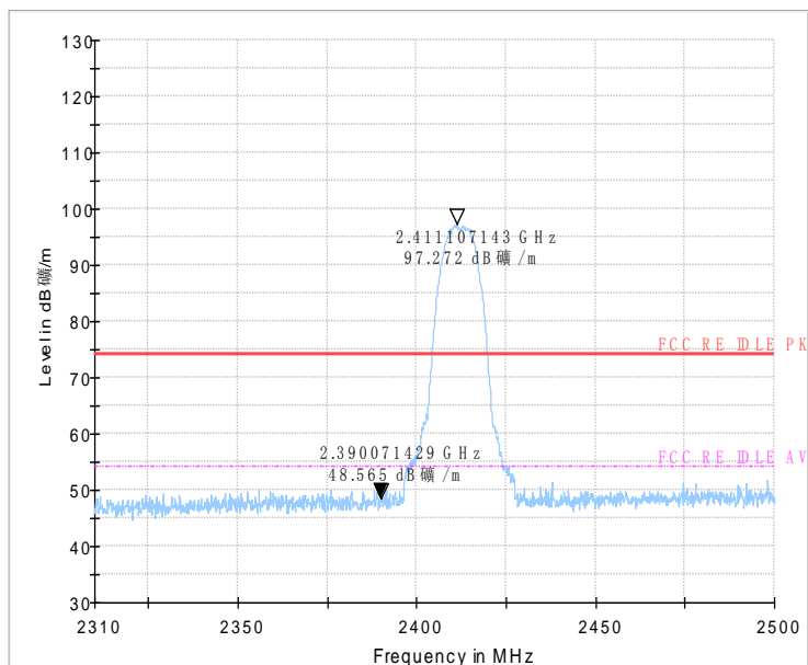
Fig.44 Radiated emission (Power): 802.11b, low channel
