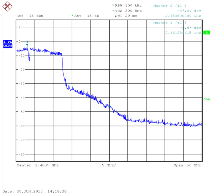
Fig.32 Band Edges (802.11n-40MHz, Ch11)
