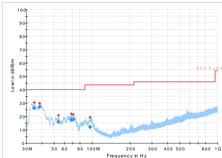
Fig.52 Radiated emission: 8DPSK, Ch0, 30MHz~1GHz
