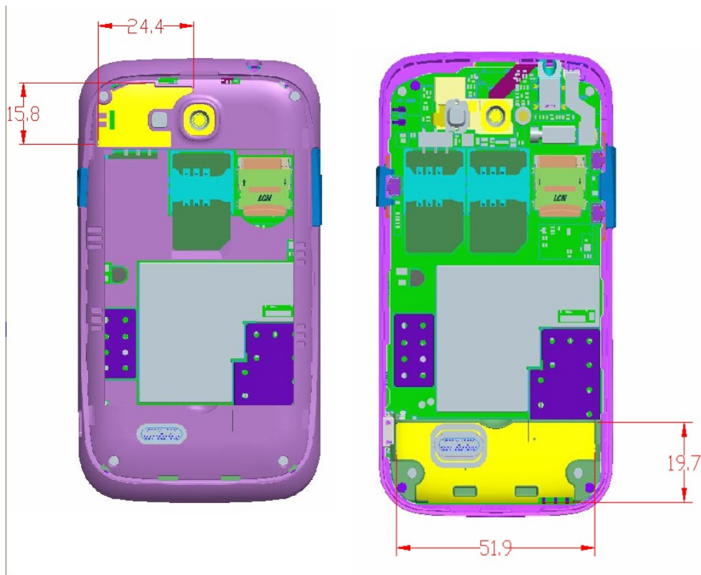
c: Antenna
