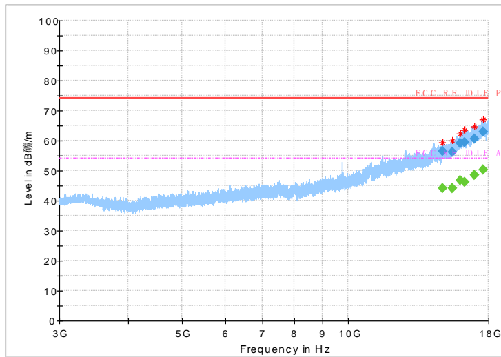
Fig.58 Radiated Spurious Emission (802.11 n-20MHz,Ch1,3GHz~18GHz)
