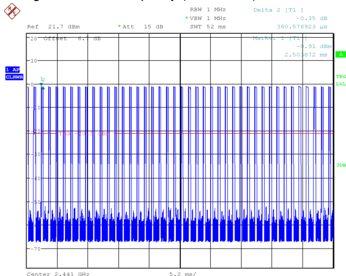
Fig.58 Time of occupancy (Dwell Time): Ch39, Packet DH1
