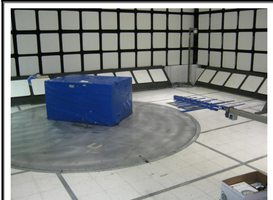
RADIATED FRONT PHOTO (BELOW 1 GHz)
