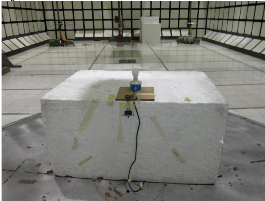
RADIATED PHOTO (30MHz to 1 GHz) 10m – Dimmer2 and Bypass2 Digital
