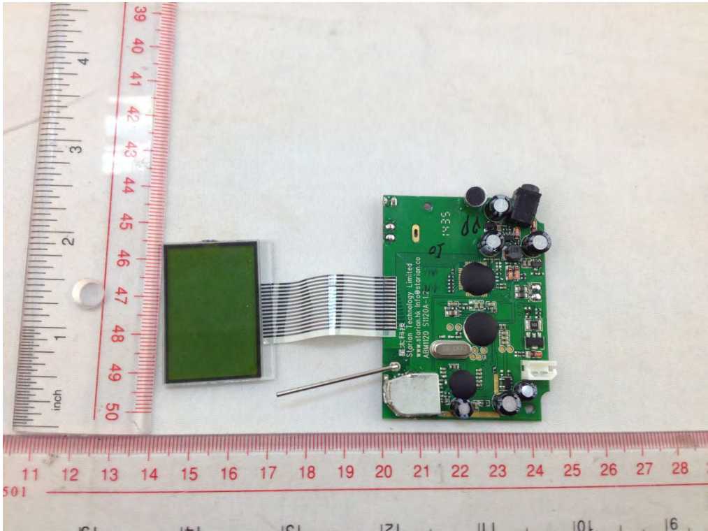
PARENT BOARD TOP VIEW 1
