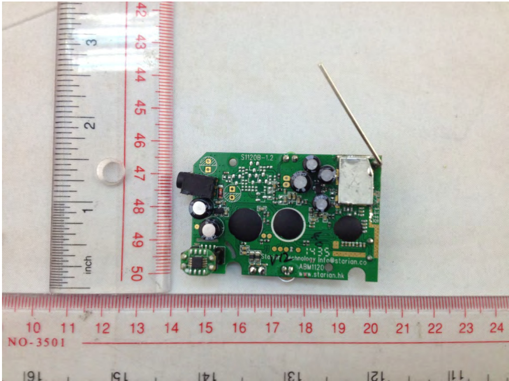
BABY BOARD TOP VIEW 1
