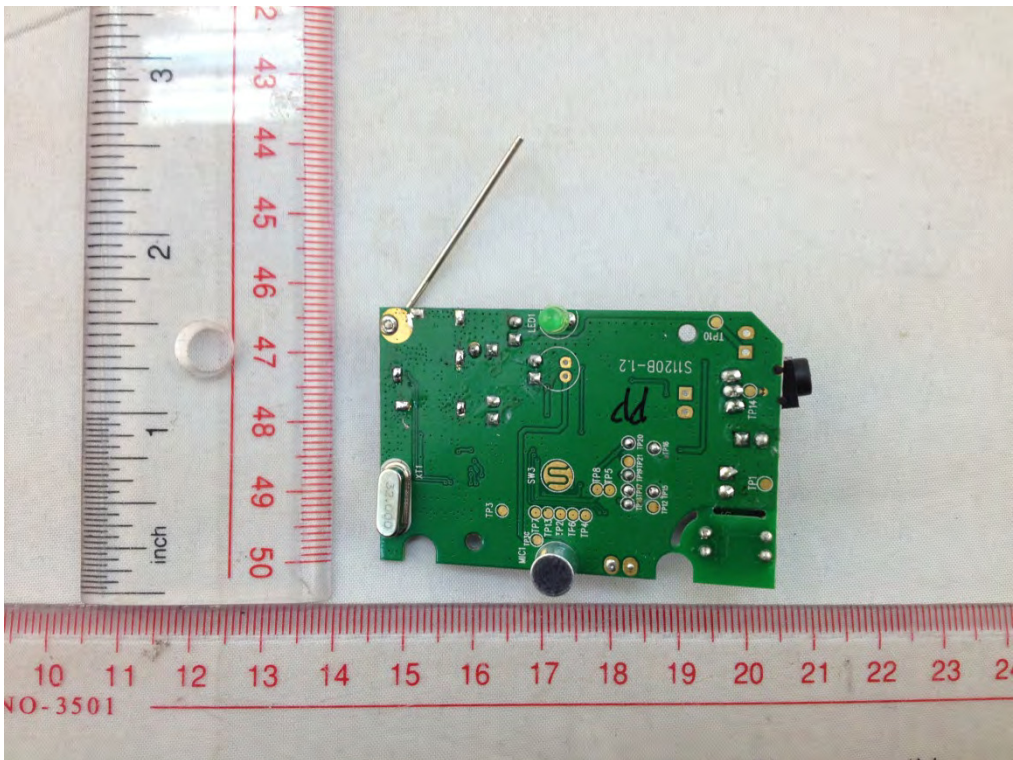
BABY BOARD BACK VIEW 1
