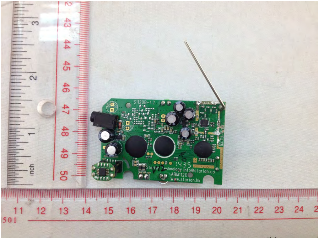
BABY BOARD TOP VIEW 2
