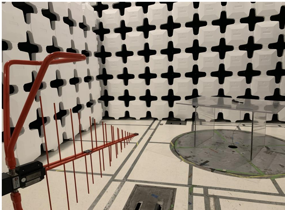
Figure 2: Radiated Spurious Emissions, 30 MHz - 1 GHz, Test Setup
