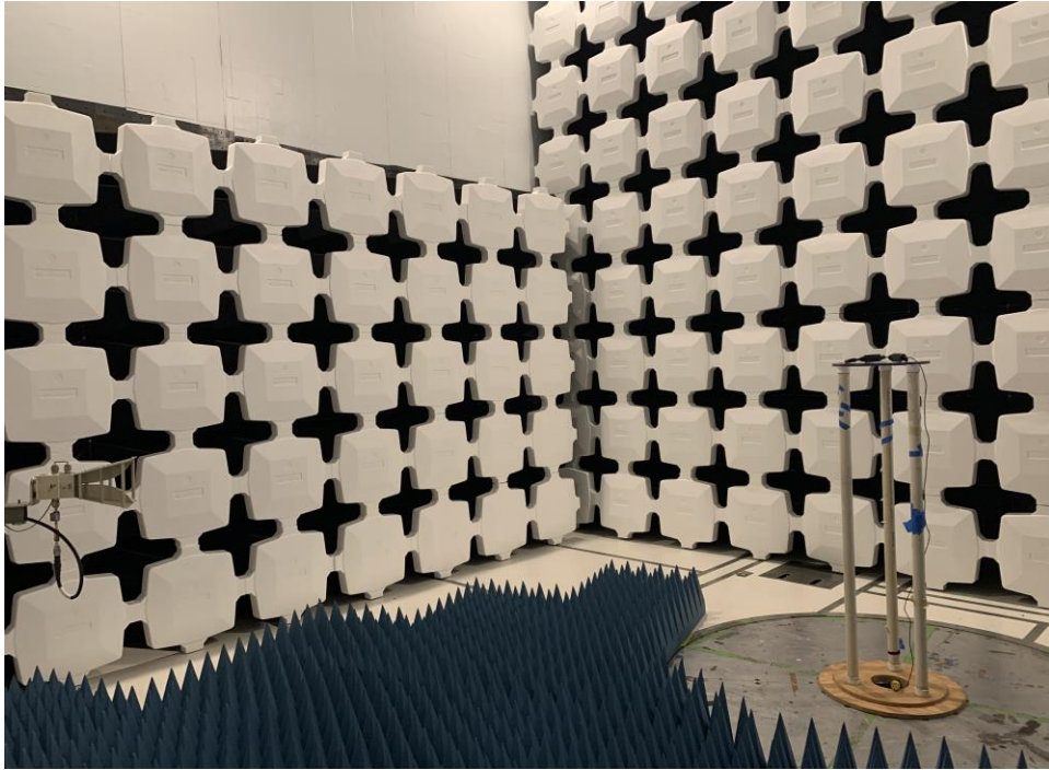
Figure 3: Radiated Spurious Emissions, 1 GHz -18 GHz, Test Setup
