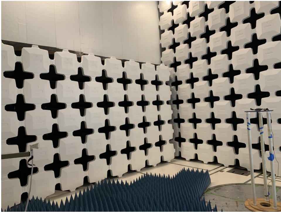
Figure 4: Radiated Spurious Emissions, 18 GHz - 25 GHz, Test Setup
