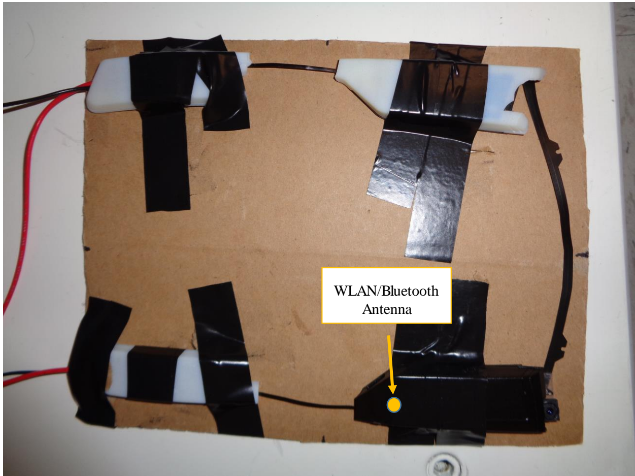
Photo 2: Antenna Location – SAR sample Outside of glasses arms shown
