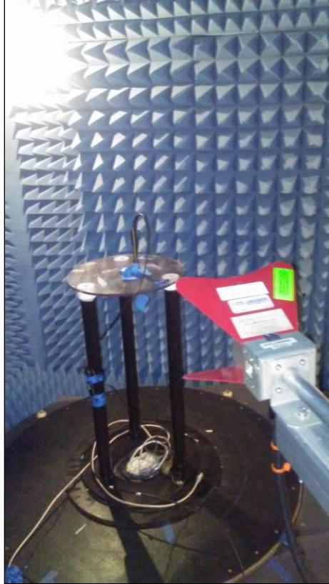
Photograph 2. Radiated Spurious Emissions, Above 1 GHz, Test Setup
