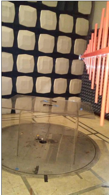
Photograph 3. Radiated Spurious Emissions, Below 1 GHz, Test Setup
