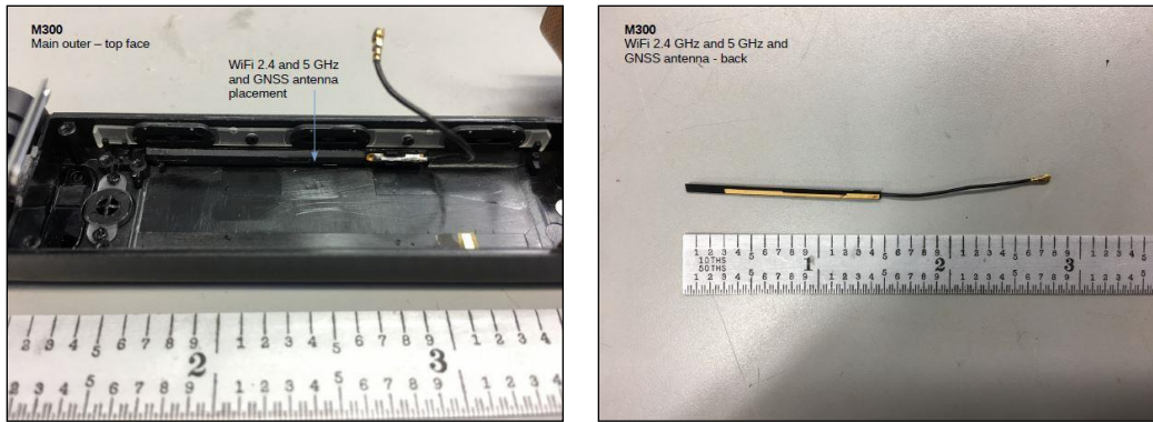
Figure 3: Antenna A.
