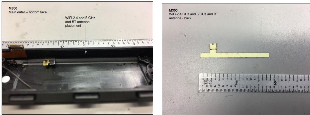
Figure 4: Antenna B.
