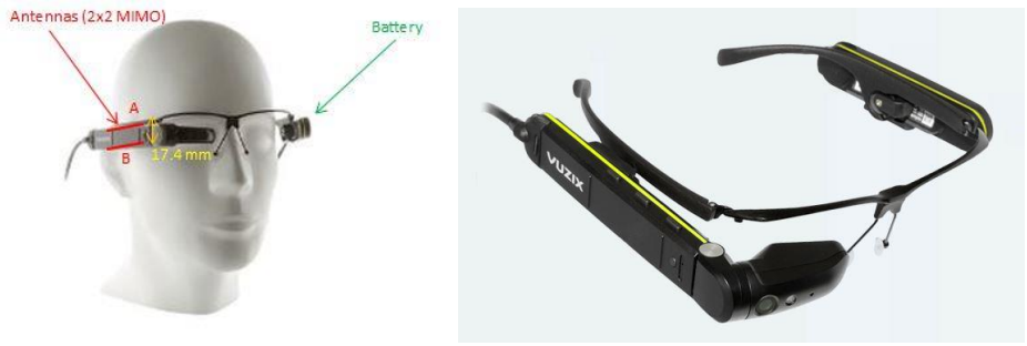
Figure 2: Vuzix M300 antenna placement.
