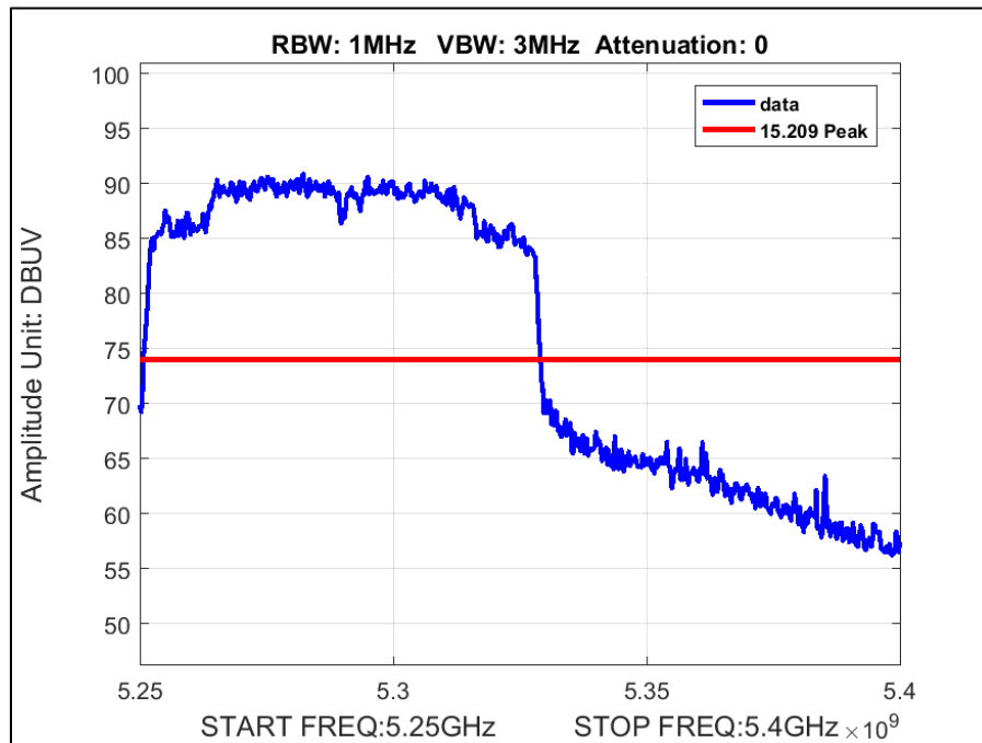
Plot 303. Undesirable Emissions, Peak Band Edge BW 80M – CH 5290M AC Mode
