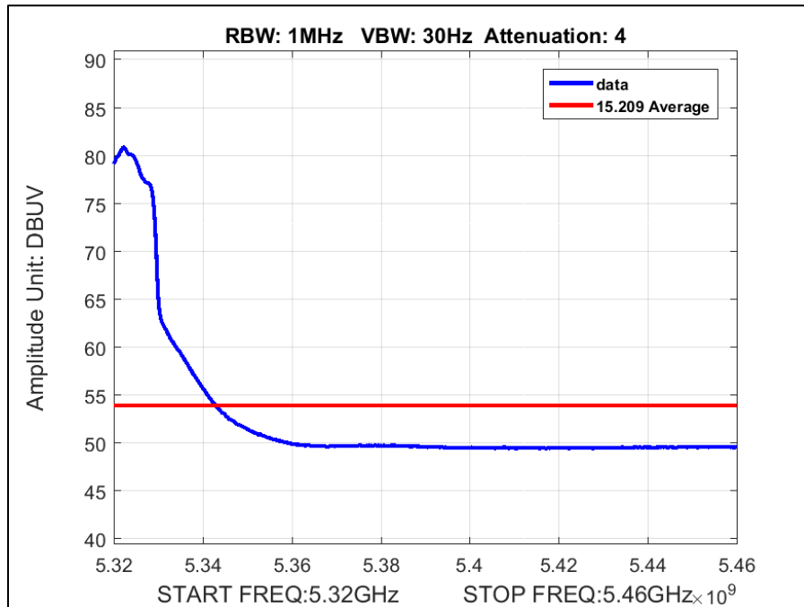
Plot 282. Undesirable Emissions, Average Band Edge BW 20M – CH 5320M AC Mode
