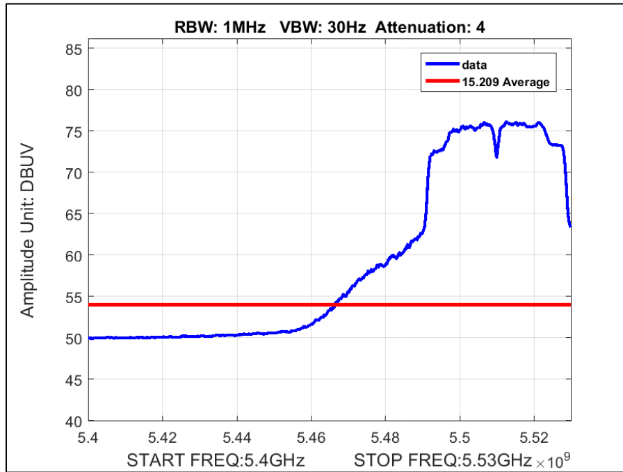
Plot 289. Undesirable Emissions, Average Band Edge BW 40M – CH 5510M AC Mode
