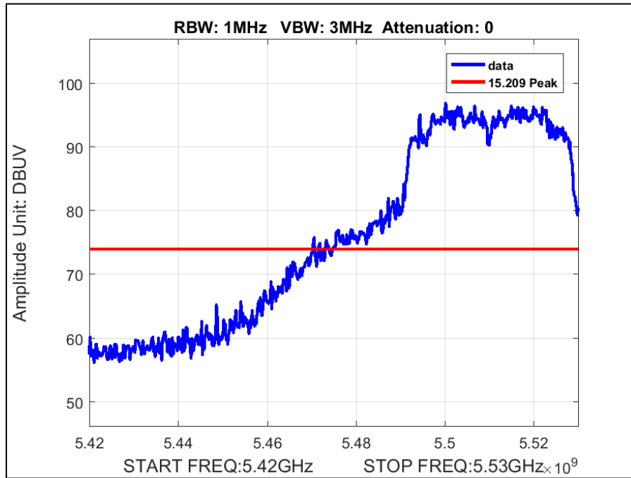
Plot 301. Undesirable Emissions, Peak Band Edge BW 40M – CH 5510M AC Mode
