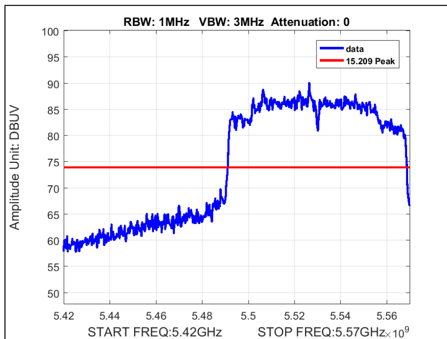
Plot 304. Undesirable Emissions, Peak Band Edge BW 80M – CH 5530M AC Mode
