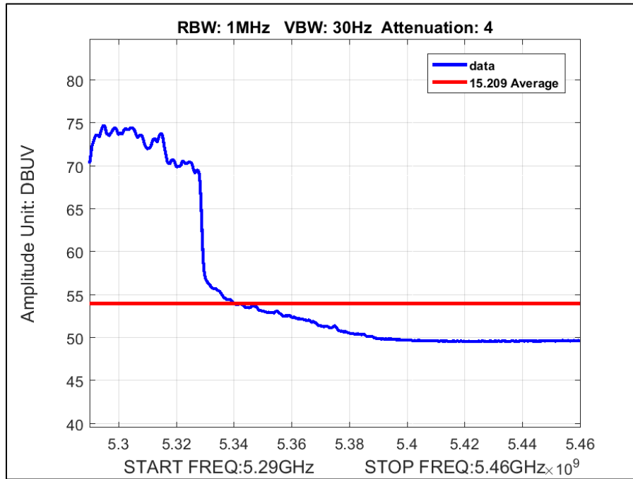
Plot 291. Undesirable Emissions, Average Band Edge BW 80M – CH 5290M AC Mode
