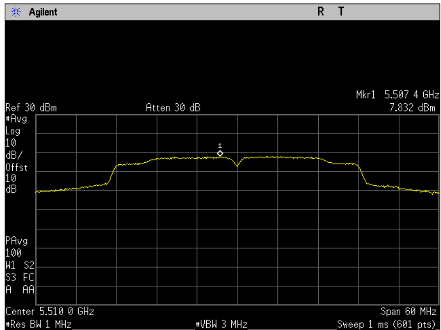
Plot 264. Power Spectral, BW 40M, Ch 5510M, N Mode, Port B
