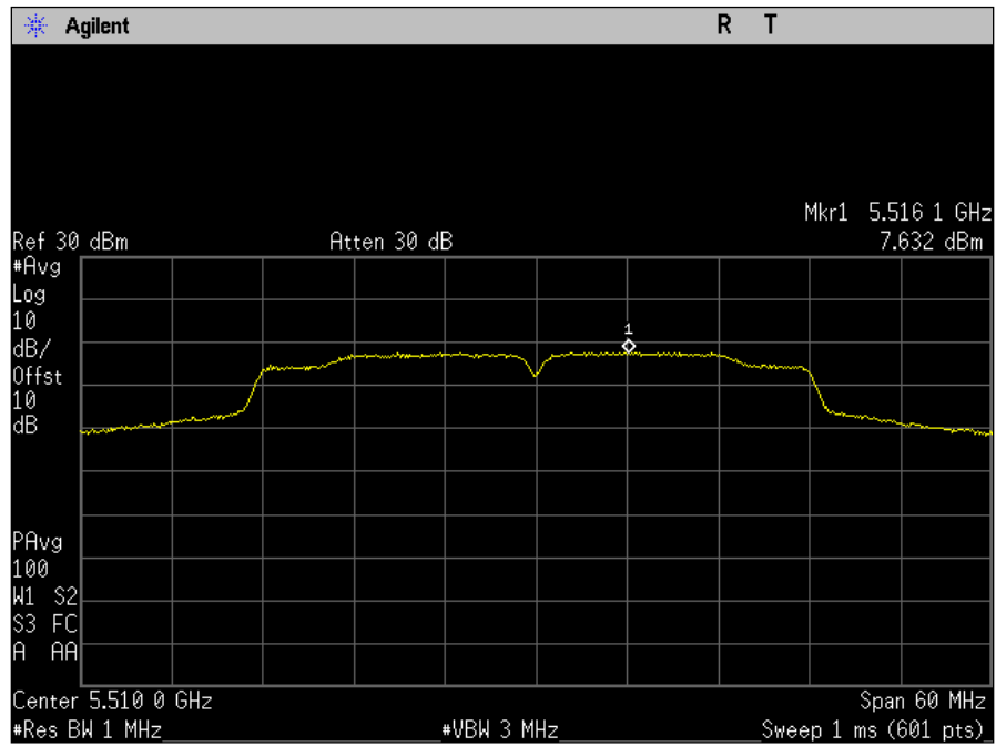
Plot 263. Power Spectral, BW 40M, Ch 5510M, AC Mode, Port B
