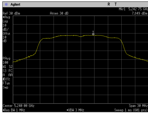
Plot 112. Power Spectral Density, MIMO, Bandwidth 20M, Ch. 5240M, ac mode, port b
