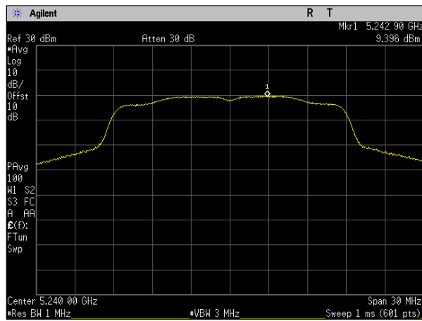
Plot 85. Power Spectral Density, SISO, Bandwidth 20M, Ch. 5240M, n mode, port b
