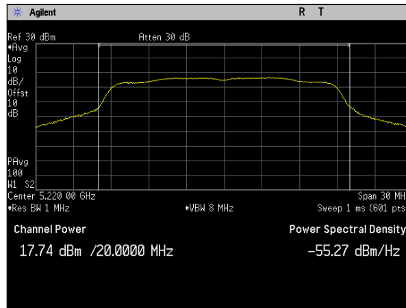
Plot 50. Conducted Transmitter Output Power, MIMO, Bandwidth 20M, Ch. 5220M, ac mode, Port b
