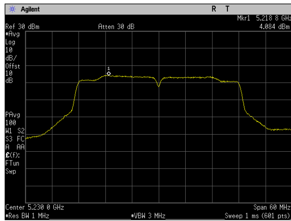
Plot 119. Power Spectral Density, MIMO, Bandwidth 40M, Ch. 5230M, ac mode, port a
