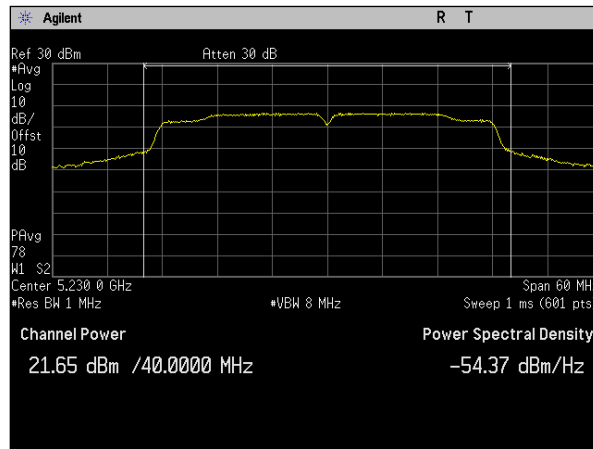
Plot 37. Conducted Transmitter Output Power, SISO, Bandwidth 40M, Ch. 5230M, n mode, Port b
