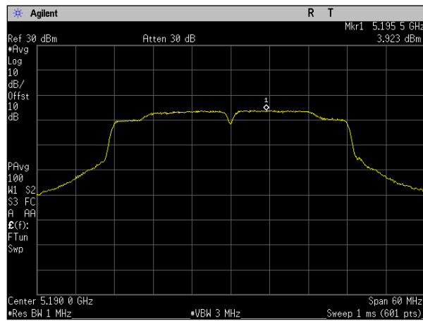
Plot 116. Power Spectral Density, MIMO, Bandwidth 40M, Ch. 5190M, ac mode, port b
