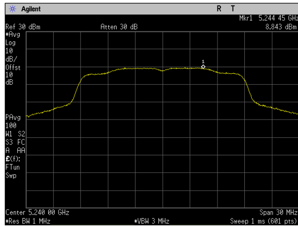
Plot 81. Power Spectral Density, SISO, Bandwidth 20M, Ch. 5240M, a mode, port b
