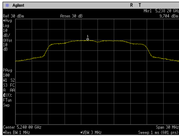
Plot 84. Power Spectral Density, SISO, Bandwidth 20M, Ch. 5240M, ac mode, port a
