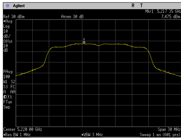
Plot 104. Power Spectral Density, MIMO, Bandwidth 20M, Ch. 5220M, a mode, port b
