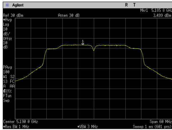
Plot 118. Power Spectral Density, MIMO, Bandwidth 40M, Ch. 5190M, n mode, port b
