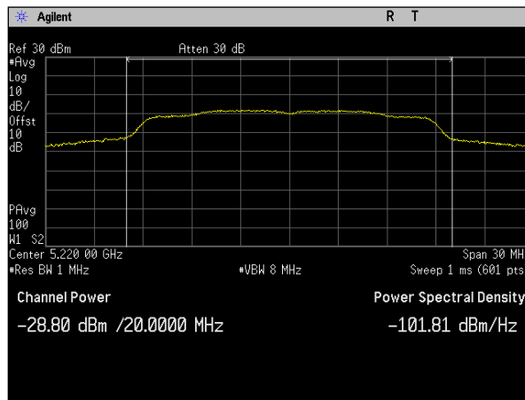
Plot 20. Conducted Transmitter Output Power, SISO, Bandwidth 20M, Ch. 5220M, a mode, Port a
