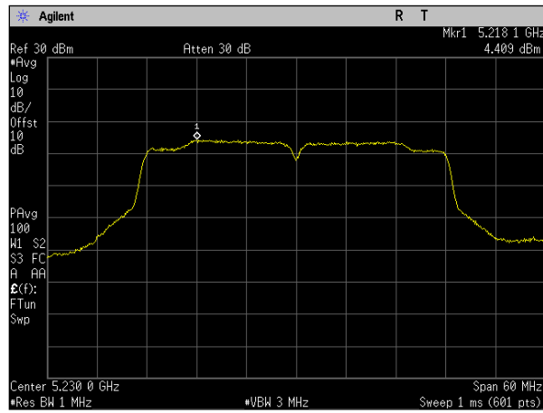
Plot 121. Power Spectral Density, MIMO, Bandwidth 40M, Ch. 5230M, n mode, port a
