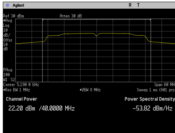
Plot 34. Conducted Transmitter Output Power, SISO, Bandwidth 40M, Ch. 5190M, n mode, Port a
