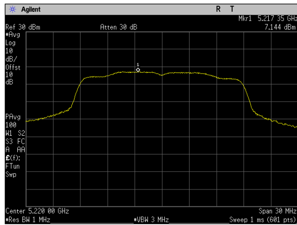
Plot 107. Power Spectral Density, MIMO, Bandwidth 20M, Ch. 5220M, n mode, port a
