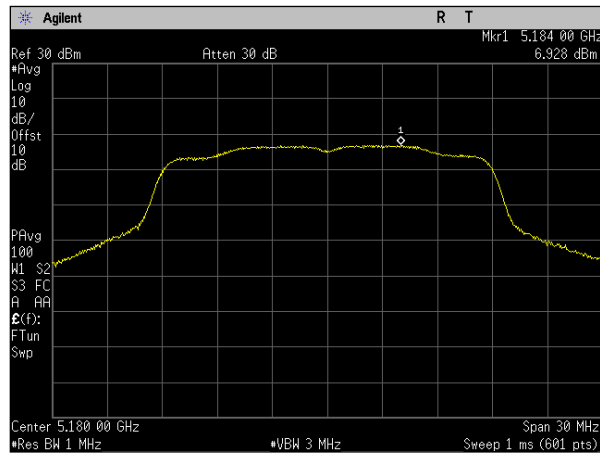
Plot 100. Power Spectral Density, MIMO, Bandwidth 20M, Ch. 5180M, ac mode, port b
