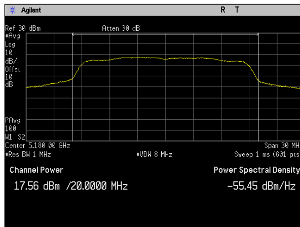
Plot 43. Conducted Transmitter Output Power, MIMO, Bandwidth 20M, Ch. 5180M, ac mode, Port a
