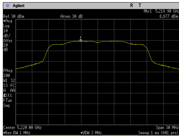
Plot 79. Power Spectral Density, SISO, Bandwidth 20M, Ch. 5220M, n mode, port b
