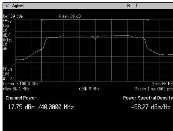
Plot 61. Conducted Transmitter Output Power, MIMO, Bandwidth 40M, Ch. 5190M, n mode, Port a
