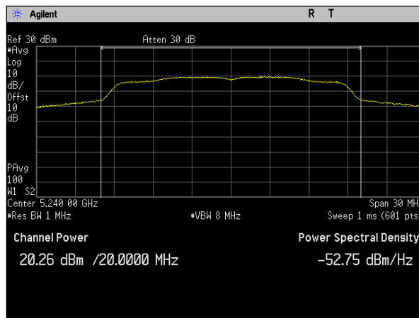
Plot 30. Conducted Transmitter Output Power, SISO, Bandwidth 20M, Ch. 5240M, n mode, Port a
