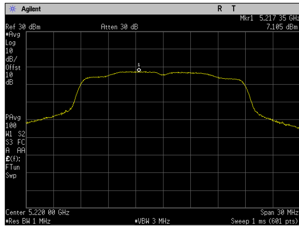
Plot 103. Power Spectral Density, MIMO, Bandwidth 20M, Ch. 5220M, a mode, port a
