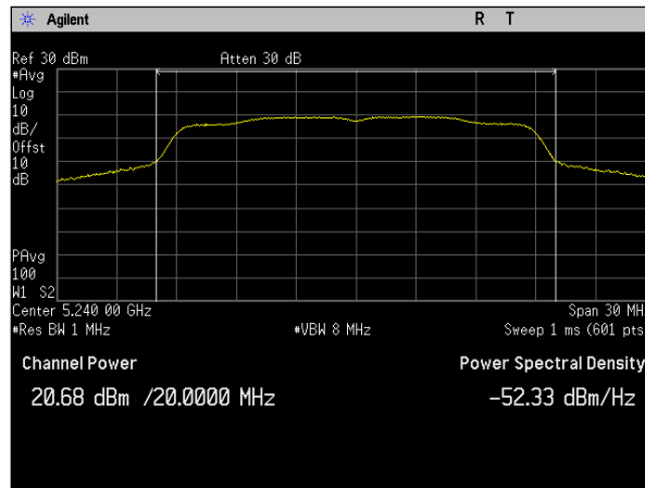
Plot 25. Conducted Transmitter Output Power, SISO, Bandwidth 20M, Ch. 5240M, a mode, Port b
