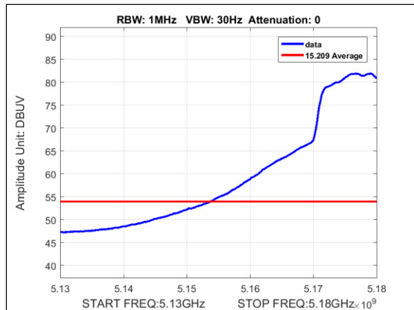
Plot 126. Undesirable Emissions, Average Band Edge Spurious, MIMO, Bandwidth 20M, Ch. 5180M, ac mode
