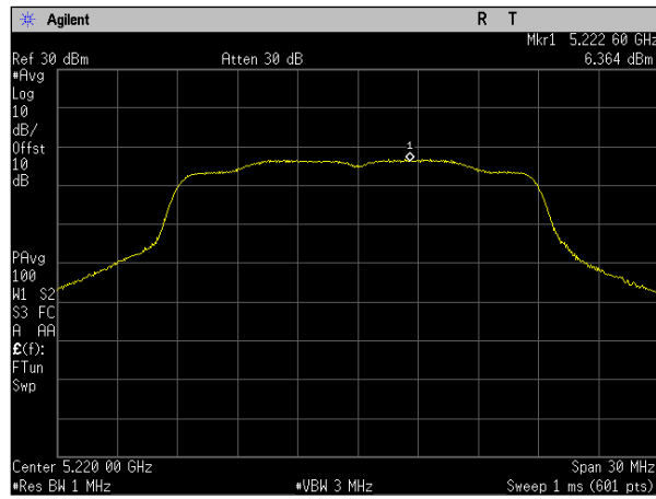
Plot 106. Power Spectral Density, MIMO, Bandwidth 20M, Ch. 5220M, ac mode, port b
