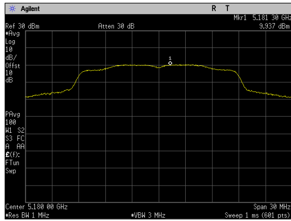
Plot 72. Power Spectral Density, SISO, Bandwidth 20M, Ch. 5180M, ac mode, port a
