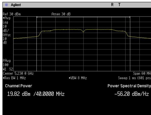
Plot 38. Conducted Transmitter Output Power, SISO, Bandwidth 40M, Ch. 5230M, n mode, Port a
