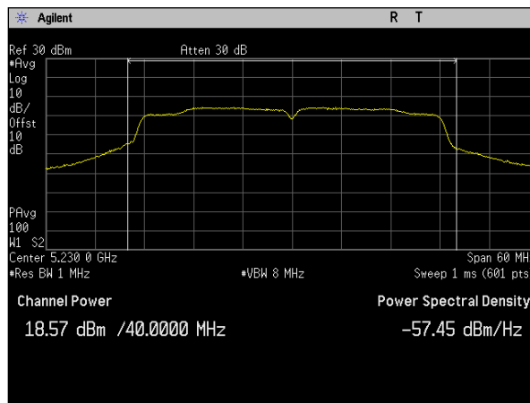
Plot 64. Conducted Transmitter Output Power, MIMO, Bandwidth 40M, Ch. 5230M, ac mode, Port b
