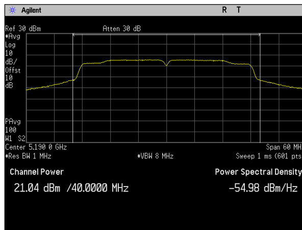
Plot 33. Conducted Transmitter Output Power, SISO, Bandwidth 40M, Ch. 5190M, n mode, Port b
