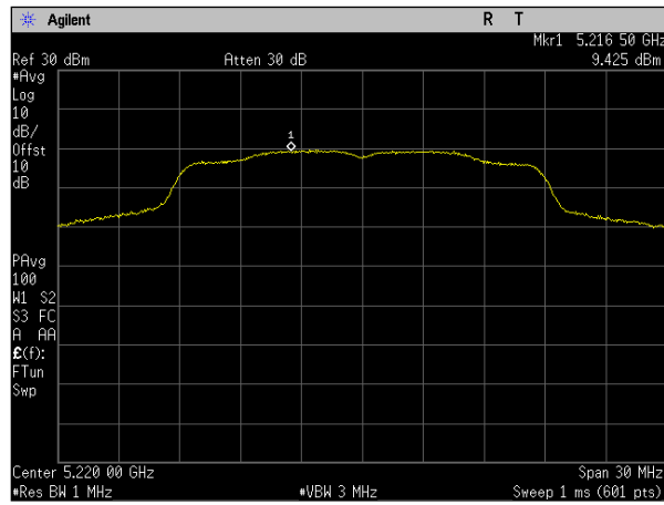
Plot 78. Power Spectral Density, SISO, Bandwidth 20M, Ch. 5220M, ac mode, port a
