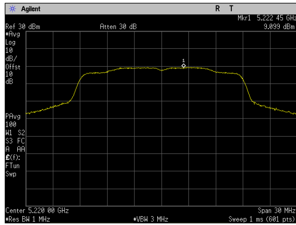
Plot 75. Power Spectral Density, SISO, Bandwidth 20M, Ch. 5220M, a mode, port b
