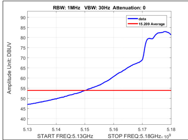
Plot 125. Undesirable Emissions, Average Band Edge Spurious, MIMO, Bandwidth 20M, Ch. 5180M, a mode setting 21
