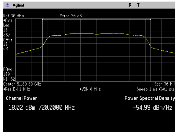
Plot 44. Conducted Transmitter Output Power, MIMO, Bandwidth 20M, Ch. 5180M, ac mode, Port b
