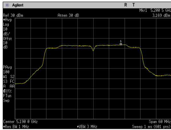
Plot 115. Power Spectral Density, MIMO, Bandwidth 40M, Ch. 5190M, ac mode, port a
