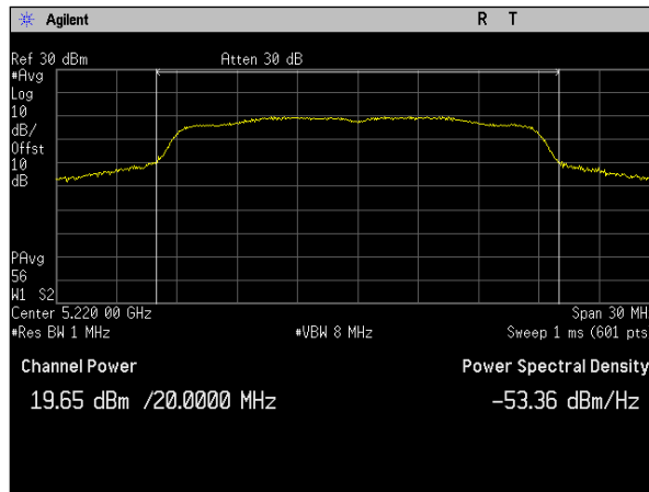
Plot 19. Conducted Transmitter Output Power, SISO, Bandwidth 20M, Ch. 5220M, a mode, Port b
