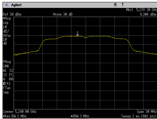
Plot 82. Power Spectral Density, SISO, Bandwidth 20M, Ch. 5240M, a mode, port a
