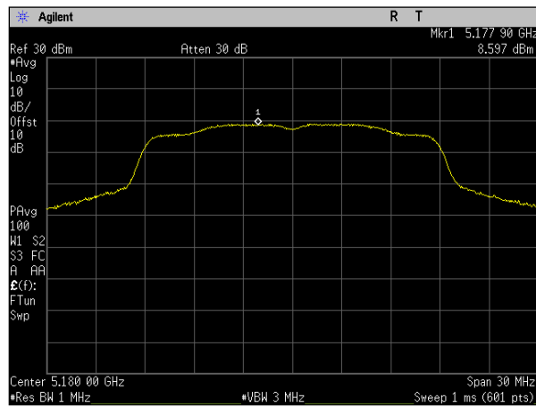
Plot 73. Power Spectral Density, SISO, Bandwidth 20M, Ch. 5180M, n mode, port b
