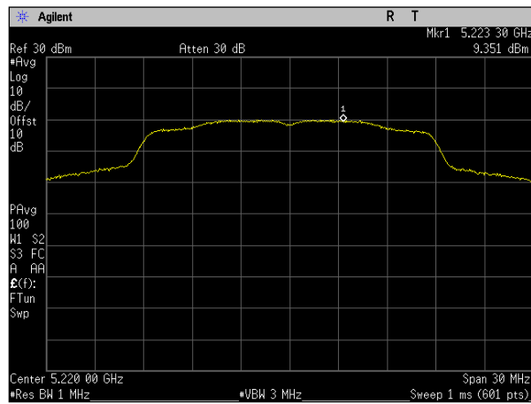
Plot 76. Power Spectral Density, SISO, Bandwidth 20M, Ch. 5220M, a mode, port a
