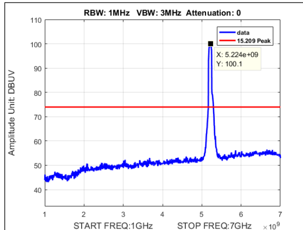
Plot 161. Undesirable Emissions, Peak Spurious Radiated Emissions, MIMO, Bandwidth 80M, Ch. 5210M, 1-7 GHz, ac mode
