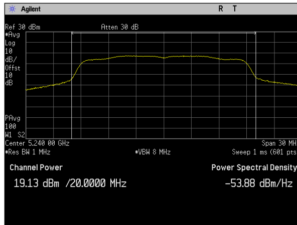
Plot 53. Conducted Transmitter Output Power, MIMO, Bandwidth 20M, Ch. 5240M, a mode, Port a
