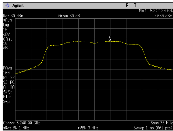
Plot 113. Power Spectral Density, MIMO, Bandwidth 20M, Ch. 5240M, n mode, port a
