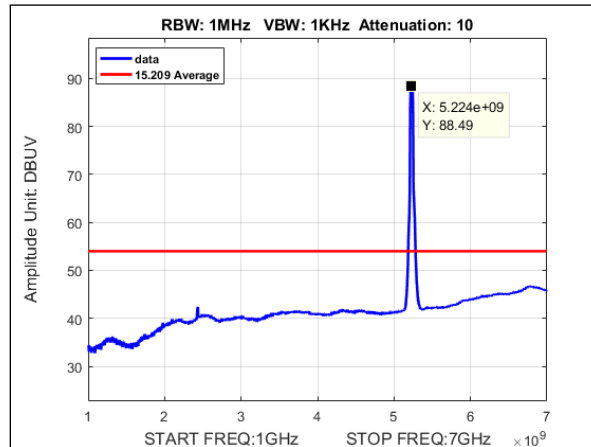
Plot 152. Undesirable Emissions, Average Spurious Radiated Emissions, MIMO, Bandwidth 40M, Ch. 5190M, 1-7 GHz, n mode
