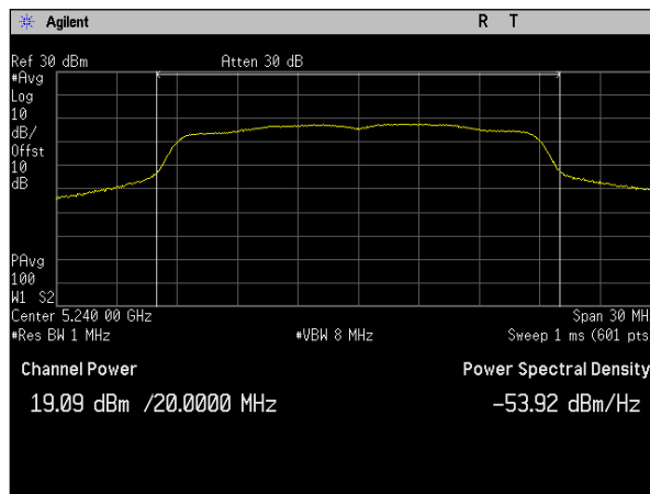
Plot 58. Conducted Transmitter Output Power, MIMO, Bandwidth 20M, Ch. 5240M, n mode, Port b
