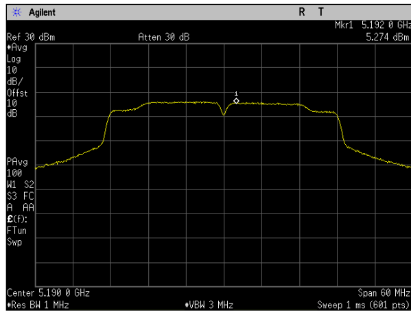
Plot 87. Power Spectral Density, SISO, Bandwidth 40M, Ch. 5190M, ac mode, port b
