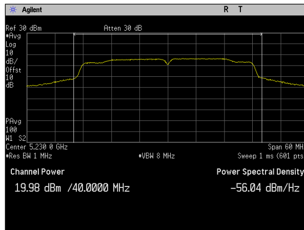
Plot 35. Conducted Transmitter Output Power, SISO, Bandwidth 40M, Ch. 5230M, ac mode, Port b
