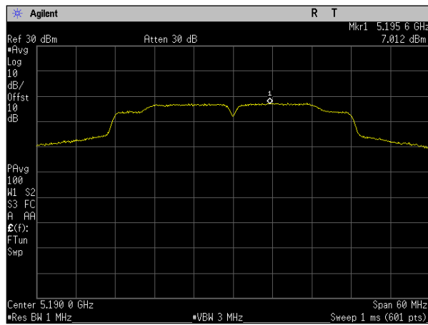
Plot 88. Power Spectral Density, SISO, Bandwidth 40M, Ch. 5190M, ac mode, port a
