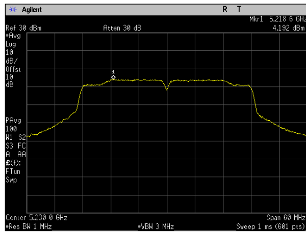
Plot 122. Power Spectral Density, MIMO, Bandwidth 40M, Ch. 5230M, n mode, port b
