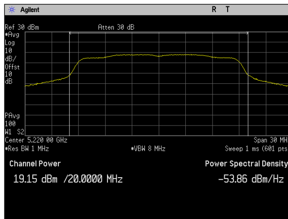
Plot 21. Conducted Transmitter Output Power, SISO, Bandwidth 20M, Ch. 5220M, ac mode, Port b
