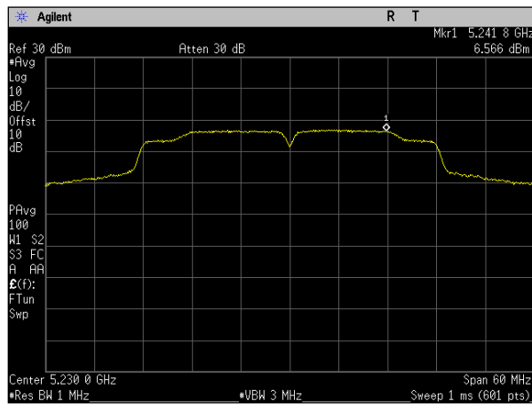
Plot 94. Power Spectral Density, SISO, Bandwidth 40M, Ch. 5230M, n mode, port a
