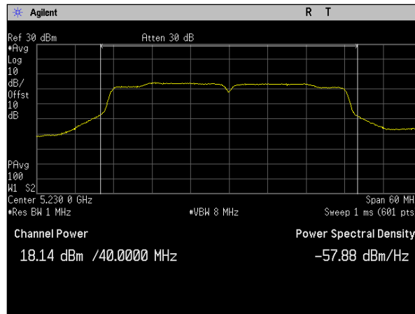
Plot 65. Conducted Transmitter Output Power, MIMO, Bandwidth 40M, Ch. 5230M, n mode, Port a
