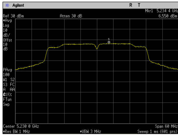
Plot 93. Power Spectral Density, SISO, Bandwidth 40M, Ch. 5230M, n mode, port b
