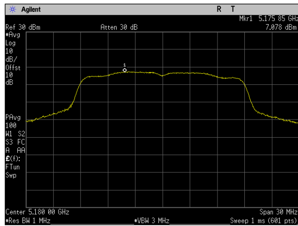
Plot 101. Power Spectral Density, MIMO, Bandwidth 20M, Ch. 5180M, n mode, port a
