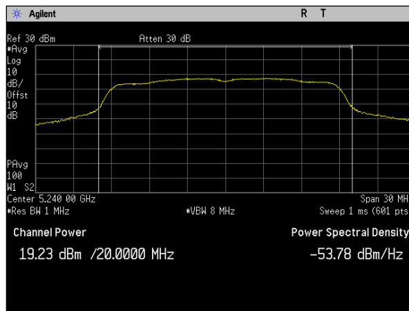
Plot 55. Conducted Transmitter Output Power, MIMO, Bandwidth 20M, Ch. 5240M, ac mode, Port a
