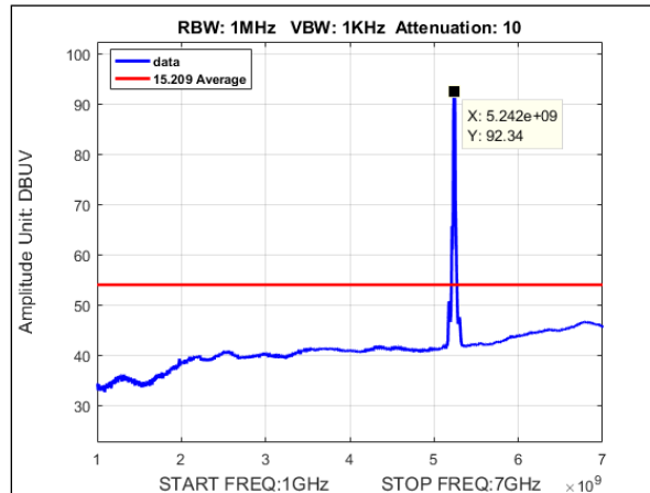
Plot 143. Undesirable Emissions, Average Spurious Radiated Emissions, MIMO, Bandwidth 20M, Ch. 5240M, 1-7 GHz, ac mode
