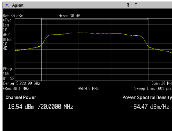
Plot 47. Conducted Transmitter Output Power, MIMO, Bandwidth 20M, Ch. 5220M, a mode, Port a
