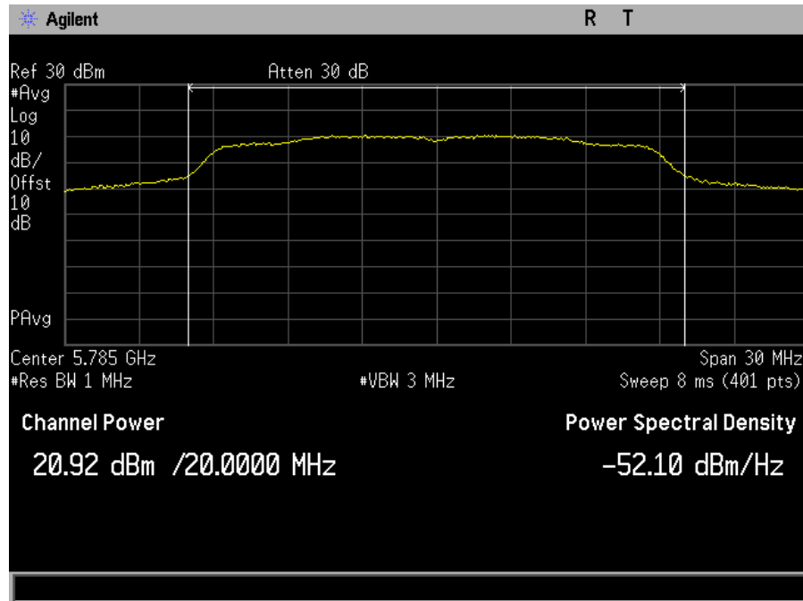
Plot 51. Maximum Conducted Output Power, MIMO, Bandwidth 20M, Ch. 5785M, ac mode, port a
