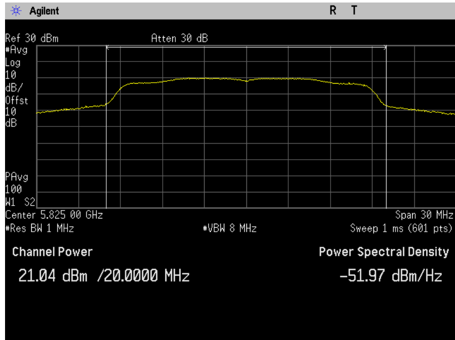
Plot 27. Maximum Conducted Output Power, SISO, Bandwidth 20M, Ch. 5825M, a mode, port b
