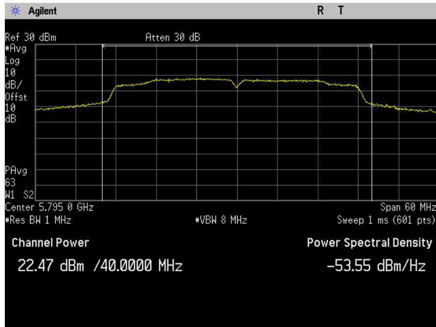
Plot 40. Maximum Conducted Output Power, SISO, Bandwidth 40M, Ch. 5795M, n mode, port b
