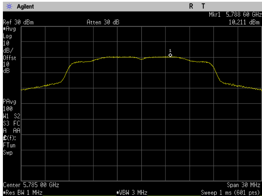
Plot 82. Power Spectral Density, SISO, Bandwidth 20M, Ch. 5785M, n mode, port b
