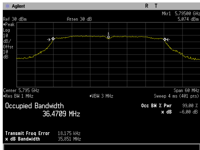
Plot 12. Occupied Bandwidth, 6dB, Bandwidth 40M, Ch. 5795M, ac mode
