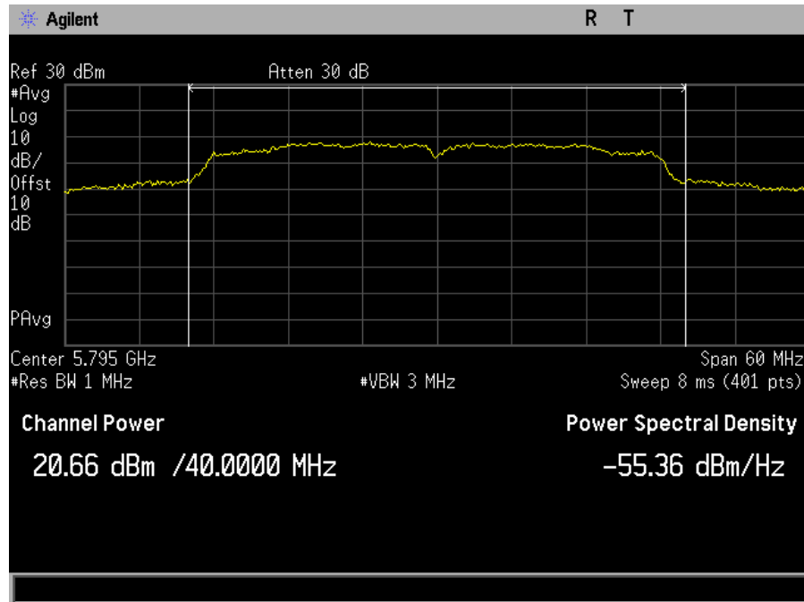
Plot 67. Maximum Conducted Output Power, MIMO, Bandwidth 40M, Ch. 5795M, n mode, port a
