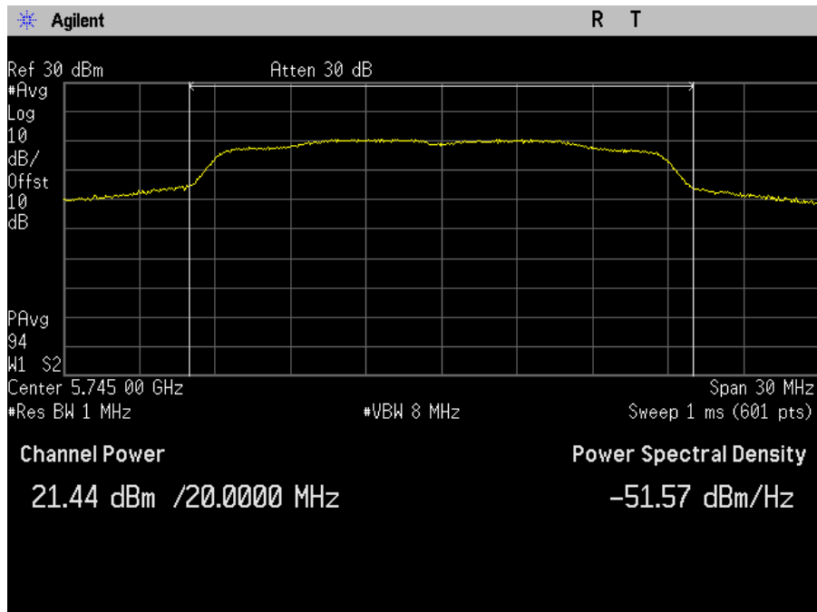
Plot 44. Maximum Conducted Output Power, MIMO, Bandwidth 20M, Ch. 5745M, a mode, port b
