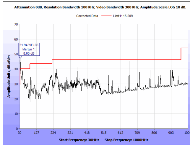
Plot 127. Undesirable Emissions, Below 1GHz
