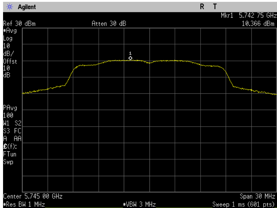
Plot 76. Power Spectral Density, SISO, Bandwidth 20M, Ch. 5745M, n mode, port b
