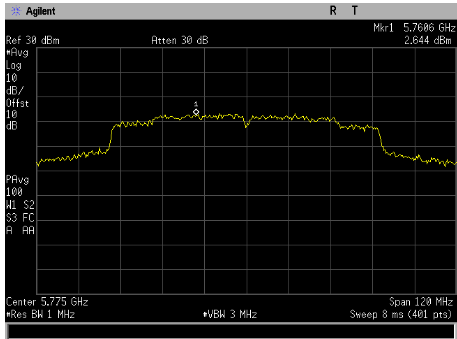
Plot 125. Power Spectral Density, MIMO, Bandwidth 80M, Ch. 5775M, ac mode, port a
