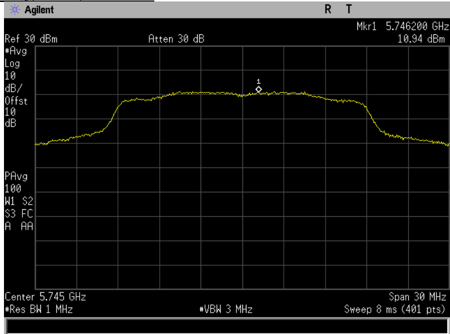
Plot 99. Power Spectral Density, MIMO, Bandwidth 20M, Ch. 5745M, a mode, port a
