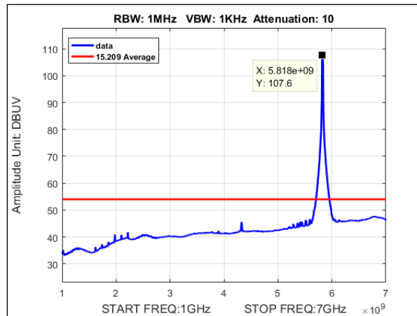
Plot 148. Undesirable Emissions, Average Radiated Spurious Emissions, MIMO, Bandwidth 20MHz, Ch. 5825, a mode, 1-7GHz
