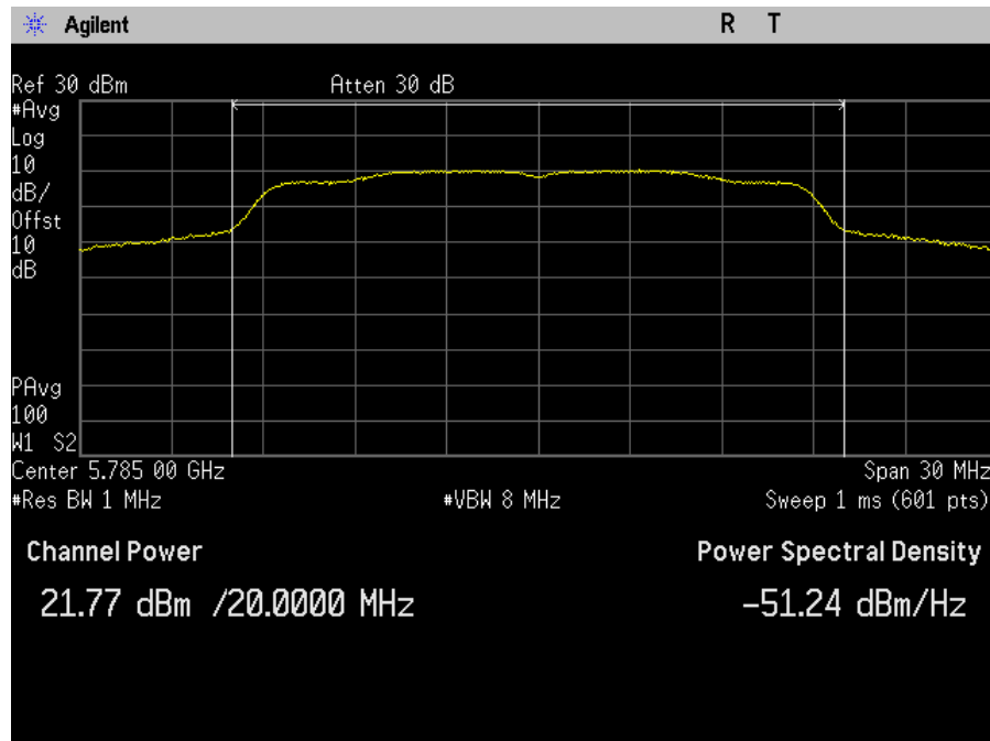
Plot 50. Maximum Conducted Output Power, MIMO, Bandwidth 20M, Ch. 5785M, a mode, port b
