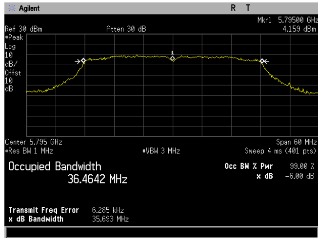
Plot 13. Occupied Bandwidth, 6dB, Bandwidth 40M, Ch. 5795M, n mode
