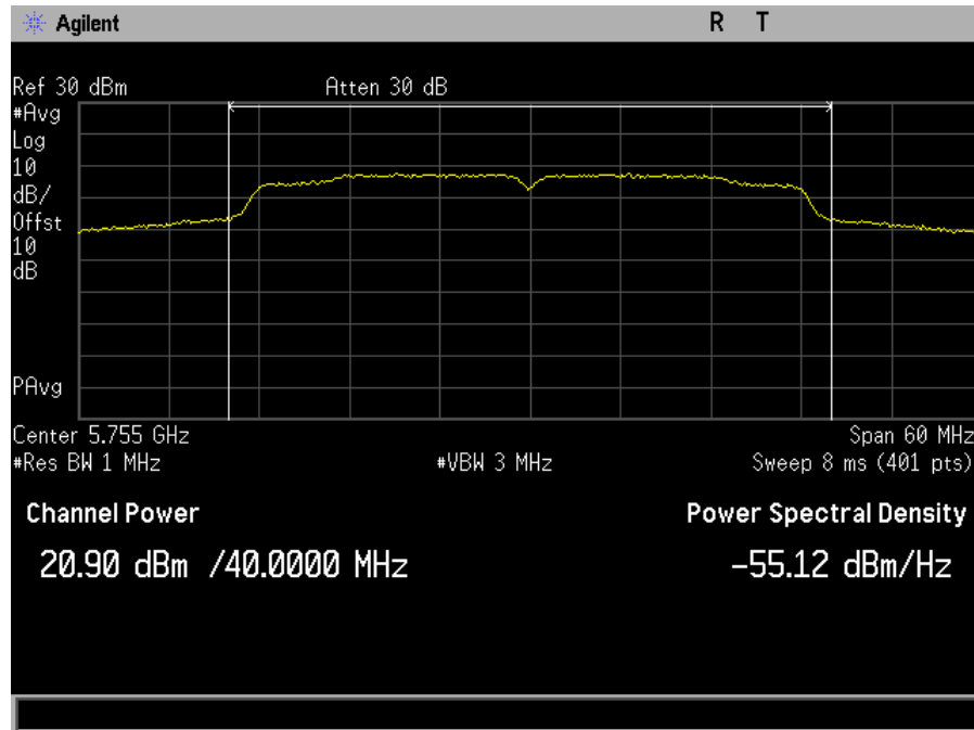
Plot 35. Maximum Conducted Output Power, SISO, Bandwidth 40M, Ch. 5755M, n mode, port a
