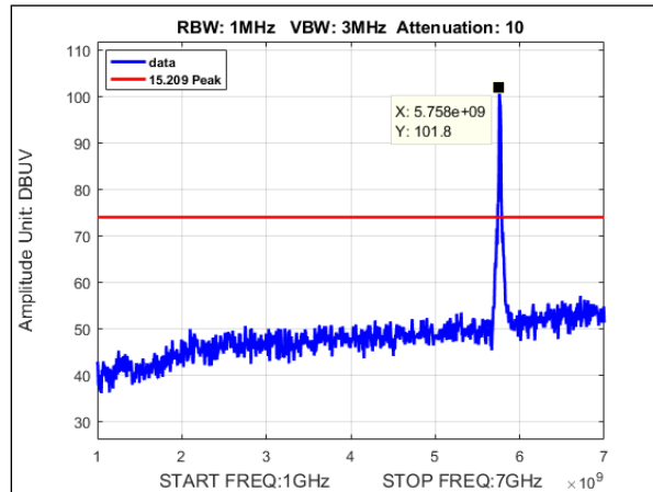
Plot 165. Undesirable Emissions, Peak Radiated Spurious Emissions, MIMO, Bandwidth 20M, Ch. 5765, n mode, 1-7GHz
