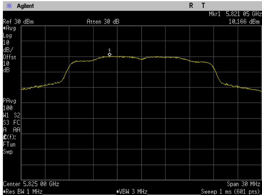
Plot 114. Power Spectral Density, MIMO, Bandwidth 20M, Ch. 5825M, ac mode, port b
