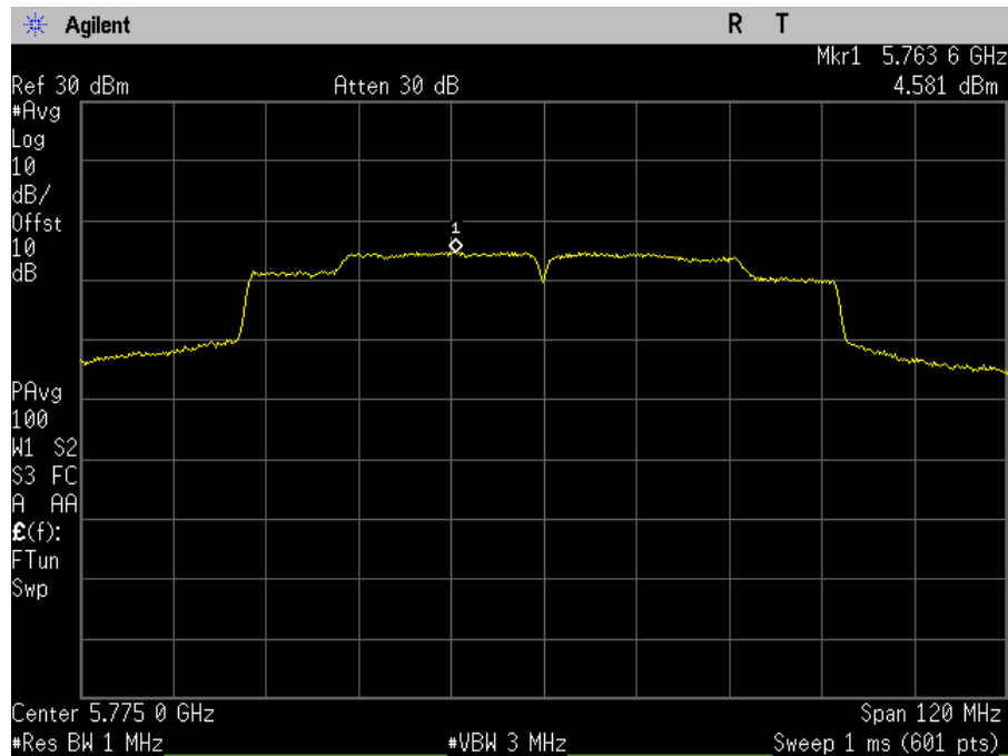
Plot 98. Power Spectral Density, SISO, Bandwidth 80M, Ch. 5775M, ac mode, port b
