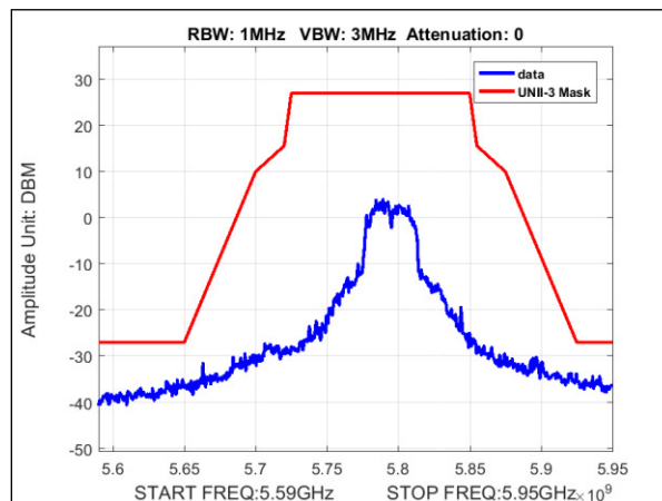
Plot 133. Undesirable Emissions, MIMO, Emissions Mask, Bandwidth 40M, Ch. 5795, ac mode
