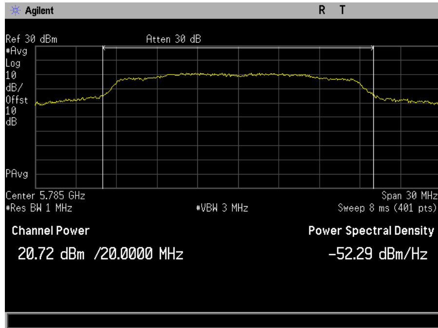
Plot 49. Maximum Conducted Output Power, MIMO, Bandwidth 20M, Ch. 5785M, a mode, port a
