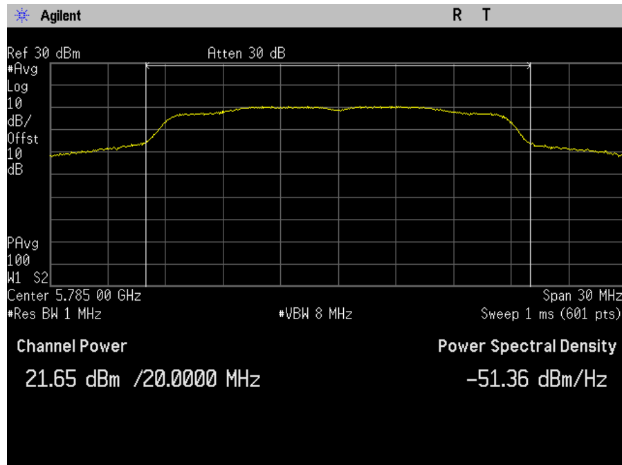
Plot 26. Maximum Conducted Output Power, SISO, Bandwidth 20M, Ch. 5785M, n mode, port b
