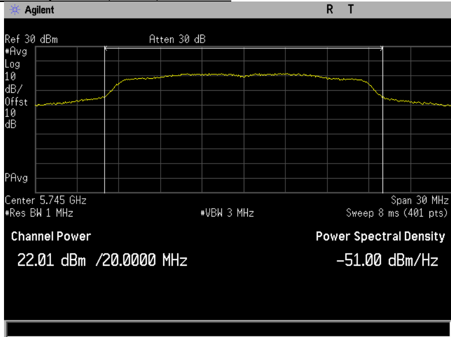
Plot 43. Maximum Conducted Output Power, MIMO, Bandwidth 20M, Ch. 5745M, a mode, port a
