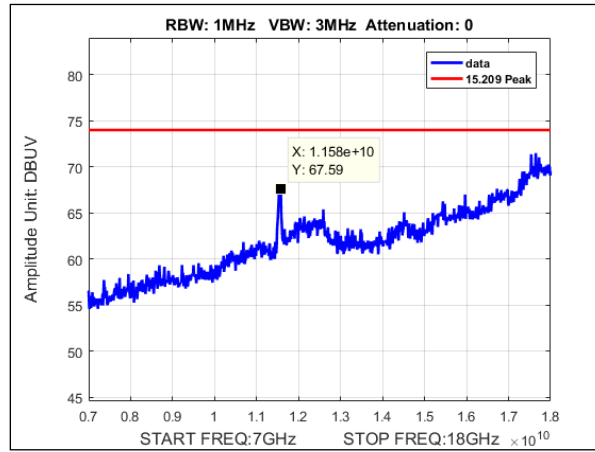
Plot 163. Undesirable Emissions, Peak Radiated Spurious Emissions, MIMO, Bandwidth 80M, Ch. 5775, ac mode, 7-18GHz
