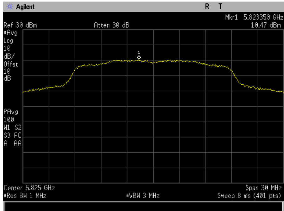
Plot 87. Power Spectral Density, SISO, Bandwidth 20M, Ch. 5825M, n mode, port a
