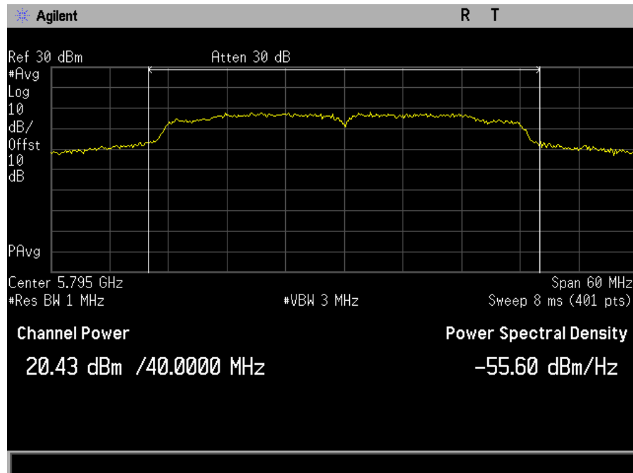
Plot 38. Maximum Conducted Output Power, SISO, Bandwidth 40M, Ch. 5795M, ac mode, port a
