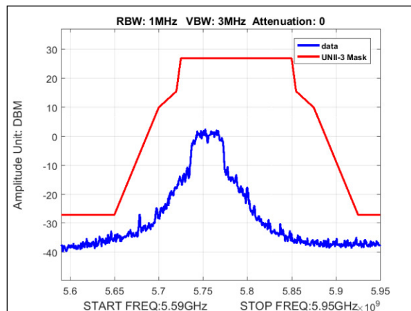
Plot 136. Undesirable Emissions, MIMO, Emissions Mask, Bandwidth 40M, Ch. 5755, n mode
