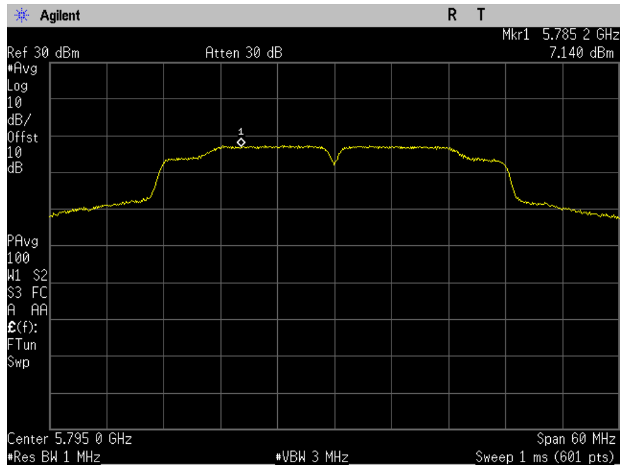
Plot 124. Power Spectral Density, MIMO, Bandwidth 40M, Ch. 5795M, n mode, port b
