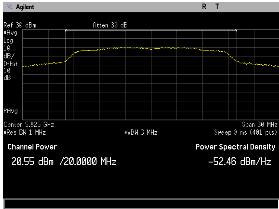
Plot 28. Maximum Conducted Output Power, SISO, Bandwidth 20M, Ch. 5825M, a mode, port a
