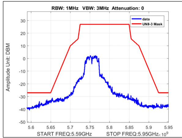
Plot 131. Undesirable Emissions, MIMO, Emissions Mask, Bandwidth 40M, Ch. 5755, ac mode
