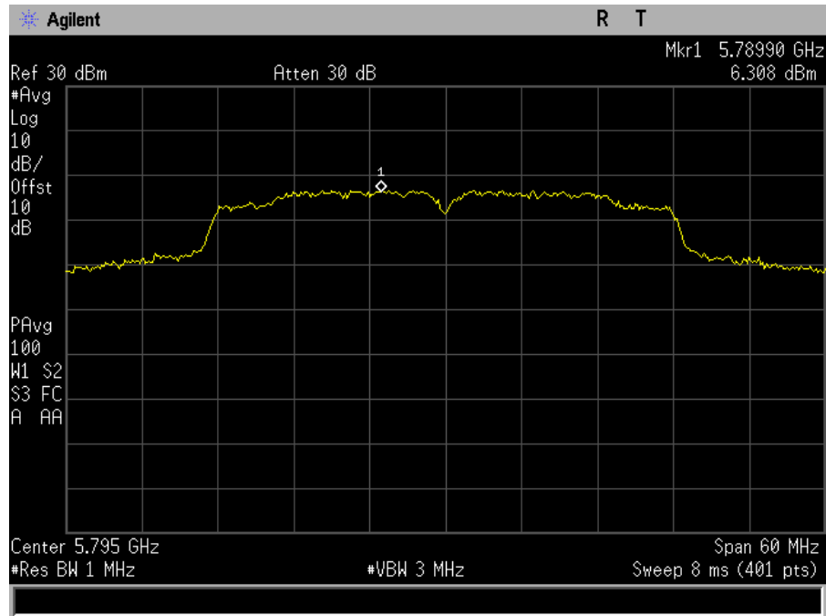
Plot 123. Power Spectral Density, MIMO, Bandwidth 40M, Ch. 5795M, n mode, port a
