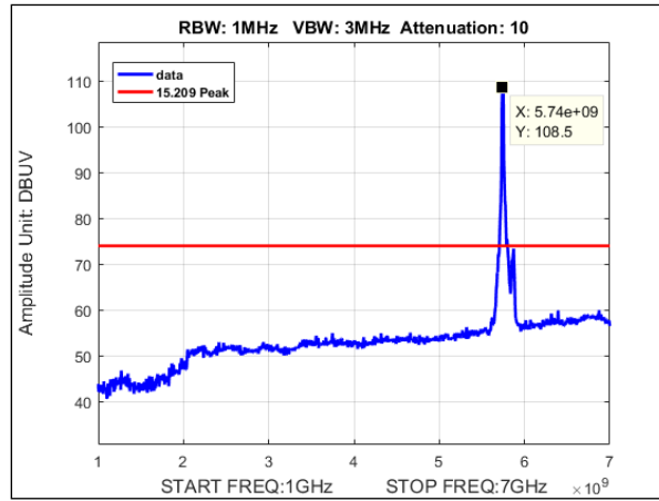
Plot 157. Undesirable Emissions, Peak Radiated Spurious Emissions, MIMO, Bandwidth 20M, Ch. 5745, ac mode, 1-7GHz
