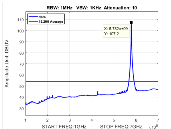
Plot 147. Undesirable Emissions, Average Radiated Spurious Emissions, MIMO, Bandwidth 20MHz, Ch. 5785, a mode, 1-7GHz
