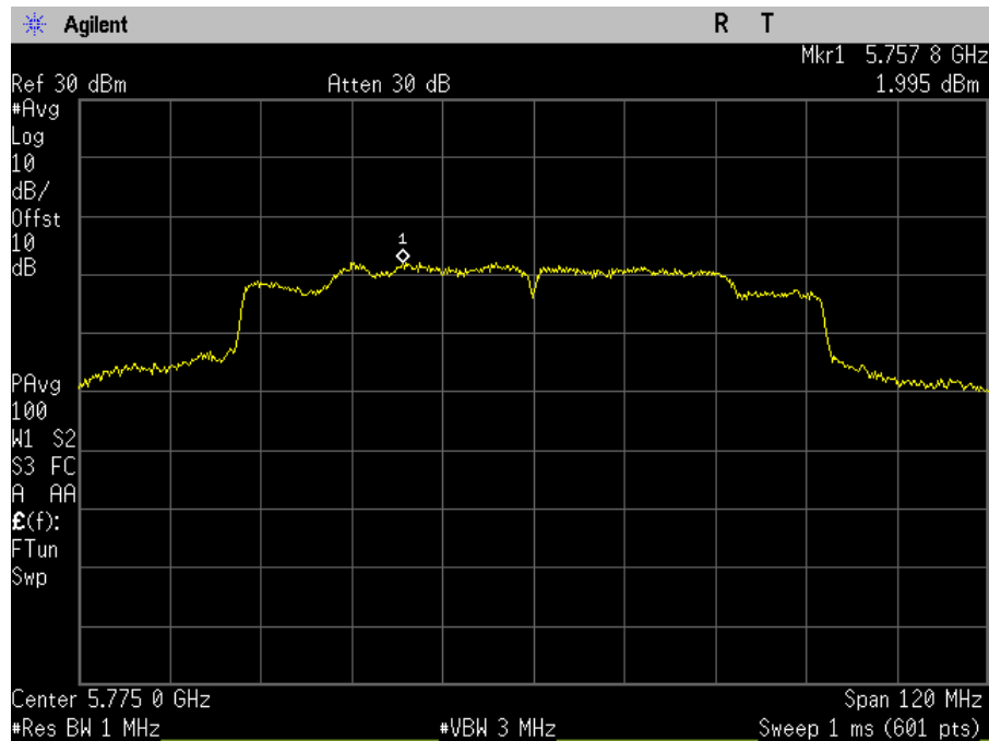
Plot 126. Power Spectral Density, MIMO, Bandwidth 80M, Ch. 5775M, ac mode, port b
