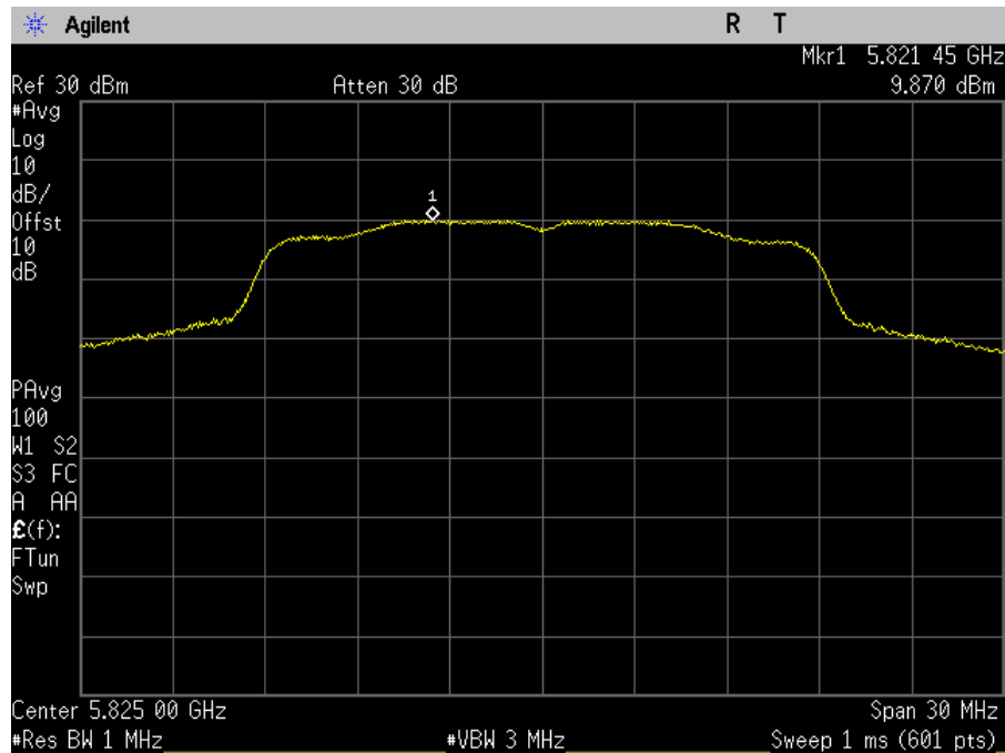
Plot 88. Power Spectral Density, SISO, Bandwidth 20M, Ch. 5825M, n mode, port b
