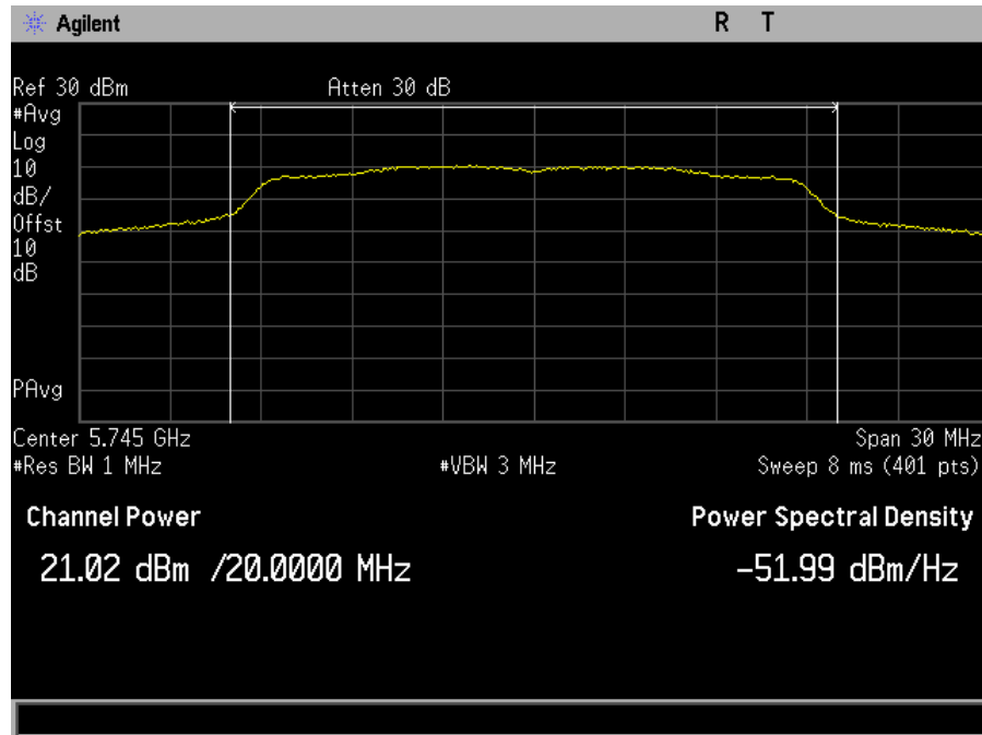
Plot 17. Maximum Conducted Output Power, SISO, Bandwidth 20M, Ch. 5745M, ac mode, port a
