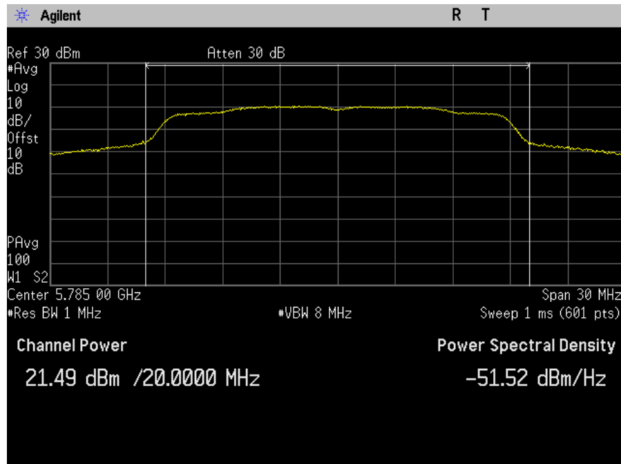
Plot 52. Maximum Conducted Output Power, MIMO, Bandwidth 20M, Ch. 5785M, ac mode, port b
