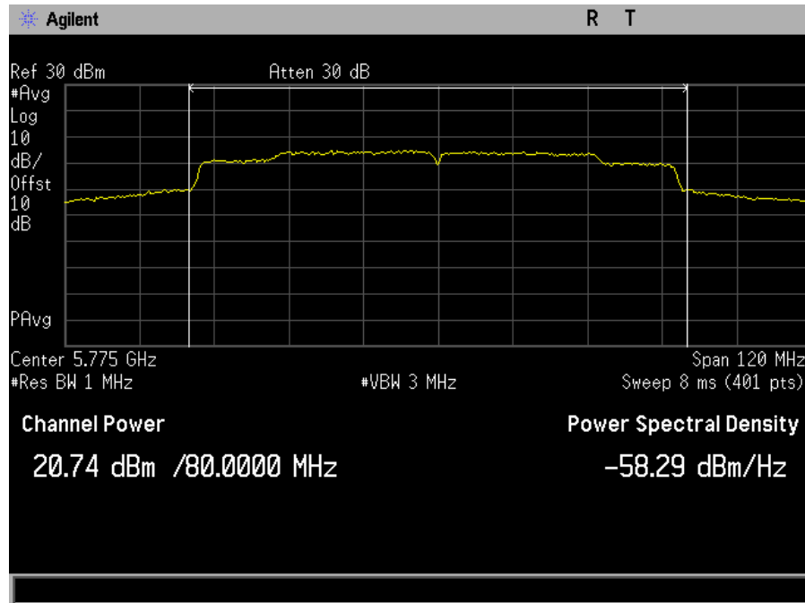
Plot 41. Maximum Conducted Output Power, SISO, Bandwidth 80M, Ch. 5775M, ac mode, port a
