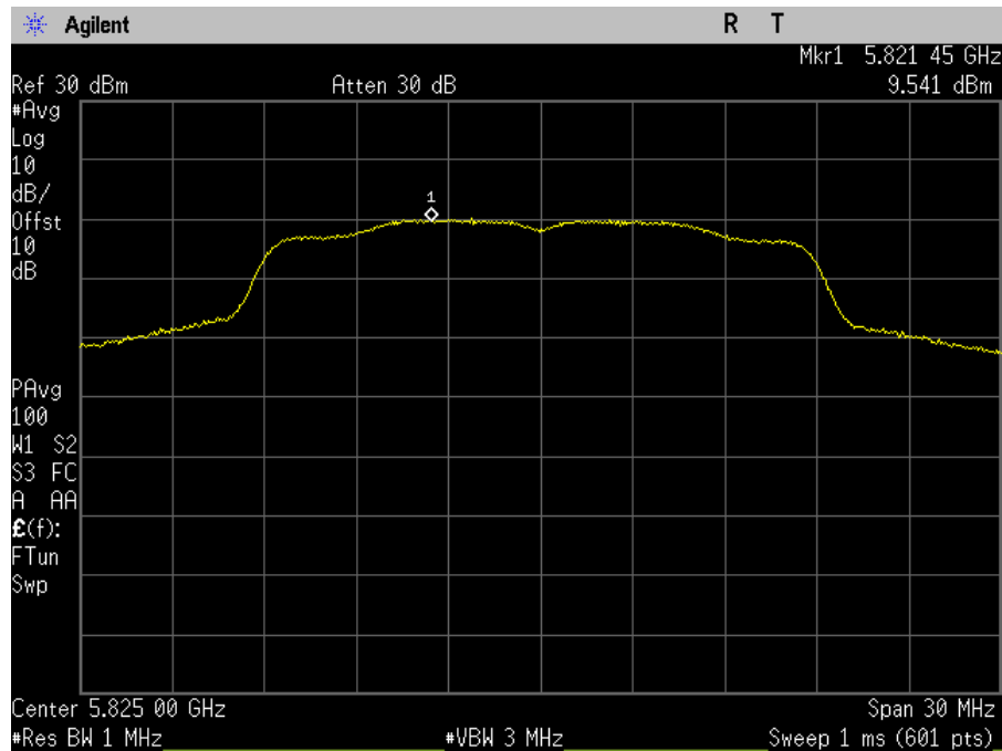
Plot 84. Power Spectral Density, SISO, Bandwidth 20M, Ch. 5825M, a mode, port b
