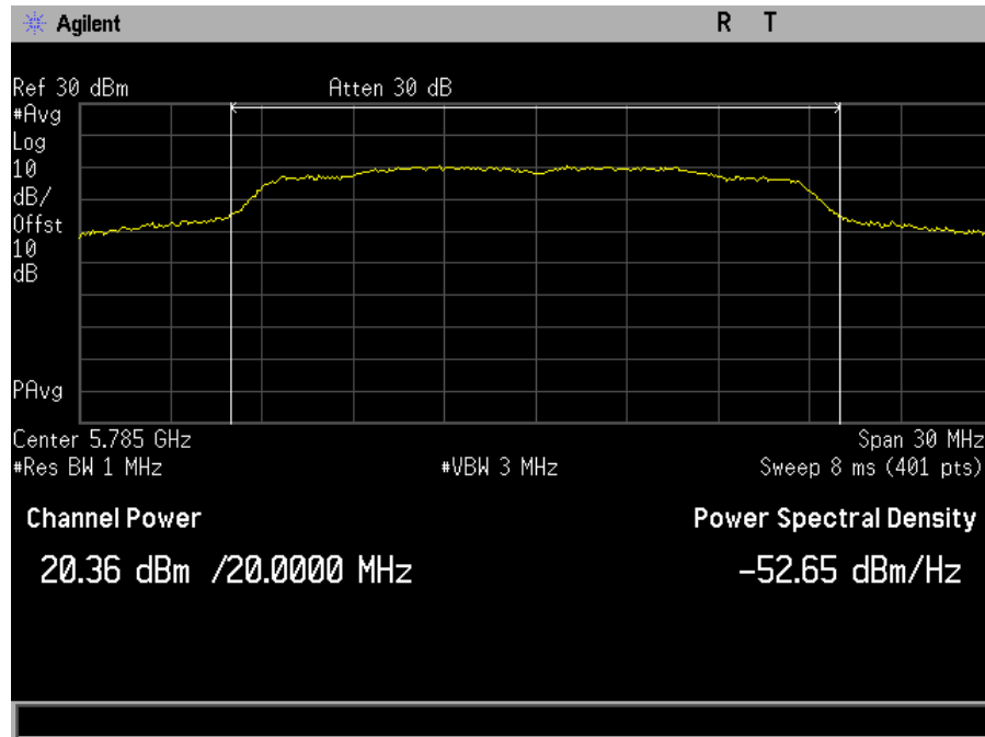
Plot 21. Maximum Conducted Output Power, SISO, Bandwidth 20M, Ch. 5785M, a mode, port a
