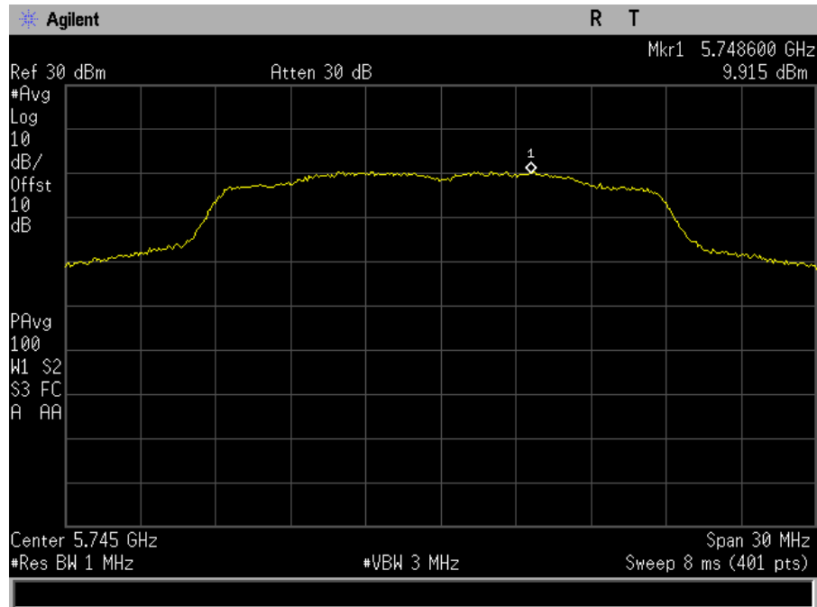
Plot 75. Power Spectral Density, SISO, Bandwidth 20M, Ch. 5745M, n mode, port a
