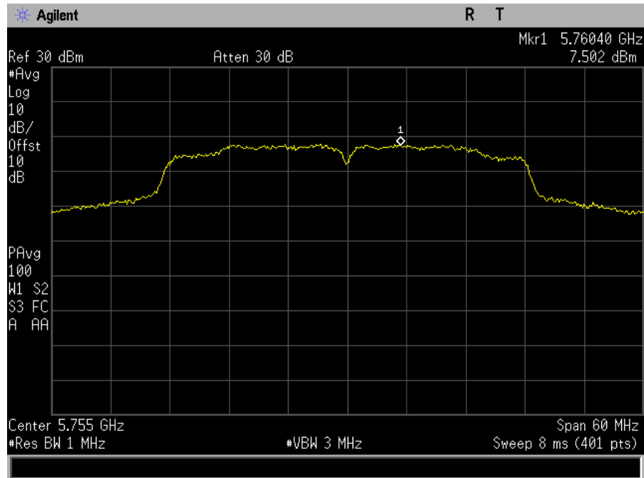
Plot 117. Power Spectral Density, MIMO, Bandwidth 40M, Ch. 5755M, ac mode, port a
