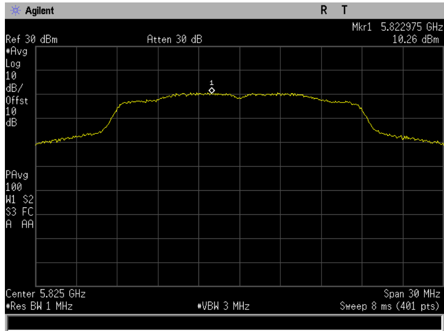
Plot 115. Power Spectral Density, MIMO, Bandwidth 20M, Ch. 5825M, n mode, port a
