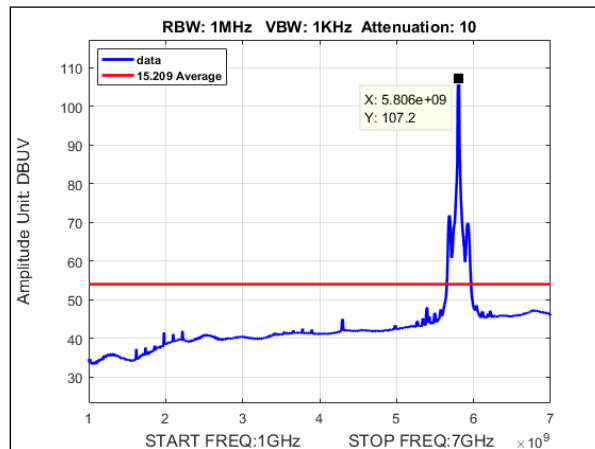
Plot 141. Undesirable Emissions, Average Radiated Spurious Emissions, MIMO, Bandwidth 20MHz, Ch. 5805, ac mode, 1-7GHz
