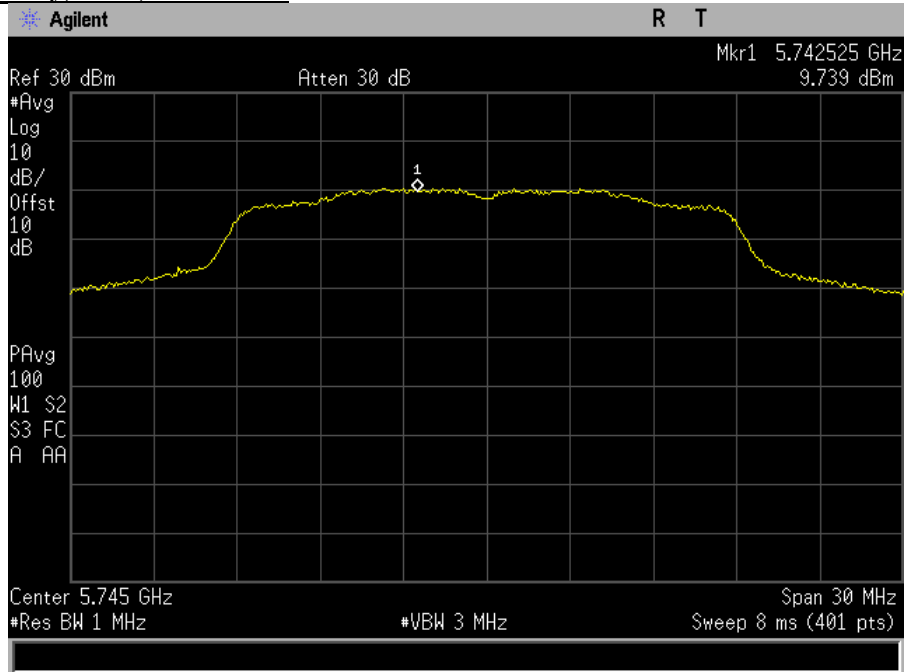
Plot 71. Power Spectral Density, SISO, Bandwidth 20M, Ch. 5745M, a mode, port a
