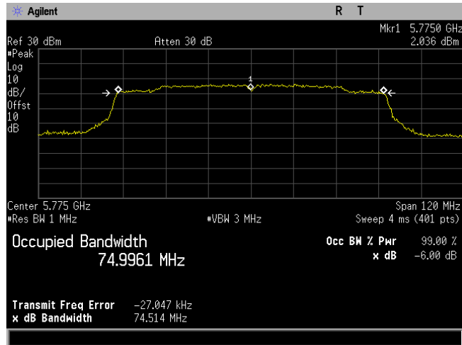
Plot 14. Occupied Bandwidth, 6dB, Bandwidth 80M, Ch. 5775M, ac mode
