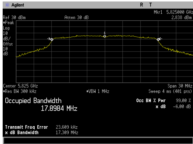
Plot 7. Occupied Bandwidth, 6dB, Bandwidth 20M, Ch. 5825M, a mode
