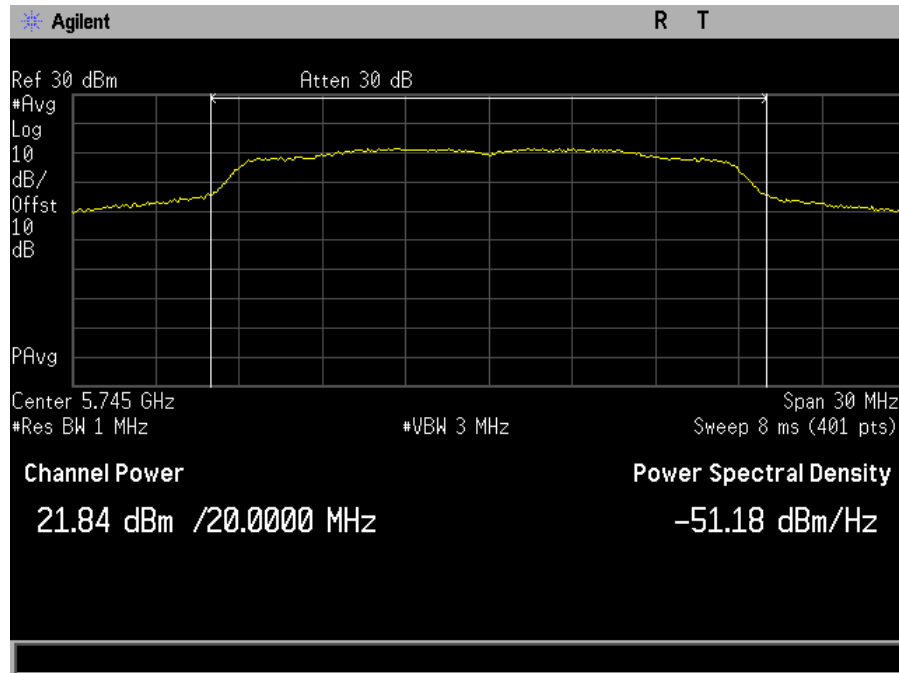
Plot 47. Maximum Conducted Output Power, MIMO, Bandwidth 20M, Ch. 5745M, n mode, port a
