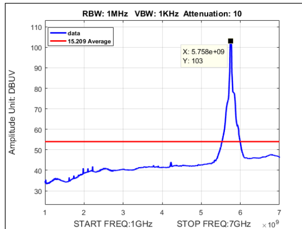
Plot 142. Undesirable Emissions, Average Radiated Spurious Emissions, MIMO, Bandwidth 40MHz, Ch. 5755, ac mode, 1-7GHz
