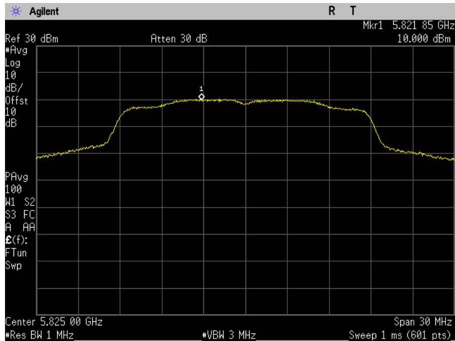
Plot 112. Power Spectral Density, MIMO, Bandwidth 20M, Ch. 5825M, a mode, port b
