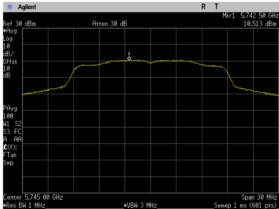
Plot 104. Power Spectral Density, MIMO, Bandwidth 20M, Ch. 5745M, n mode, port b
