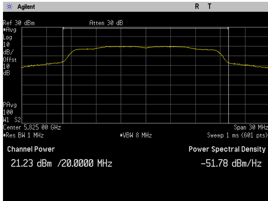
Plot 59. Maximum Conducted Output Power, MIMO, Bandwidth 20M, Ch. 5825M, n mode, port a
