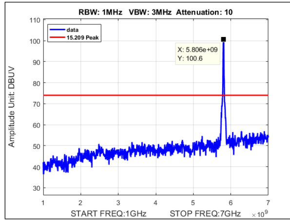
Plot 166. Undesirable Emissions, Peak Radiated Spurious Emissions, MIMO, Bandwidth 20M, Ch. 5805, n mode, 1-7GHz
