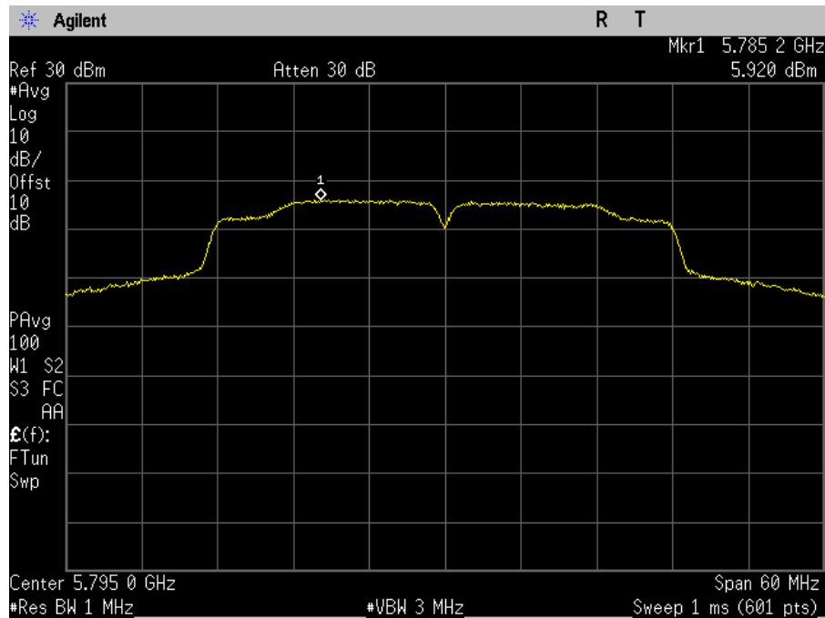
Plot 122. Power Spectral Density, MIMO, Bandwidth 40M, Ch. 5795M, ac mode, port b
