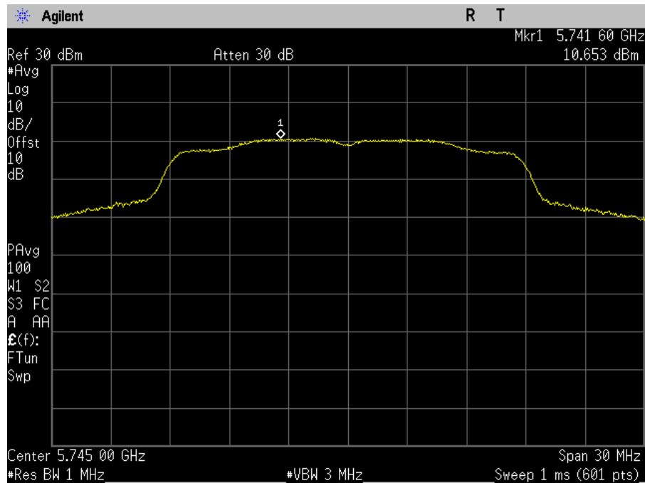
Plot 102. Power Spectral Density, MIMO, Bandwidth 20M, Ch. 5745M, ac mode, port b
