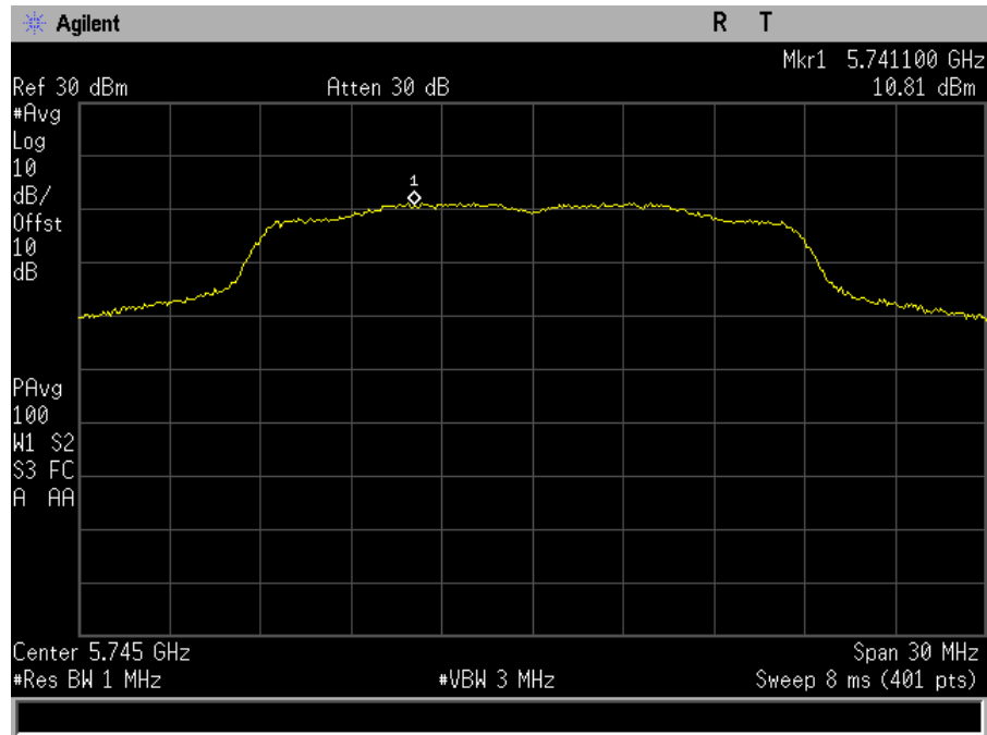
Plot 101. Power Spectral Density, MIMO, Bandwidth 20M, Ch. 5745M, ac mode, port a
