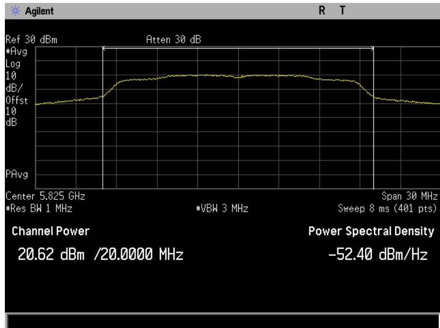
Plot 30. Maximum Conducted Output Power, SISO, Bandwidth 20M, Ch. 5825M, n mode, port a
