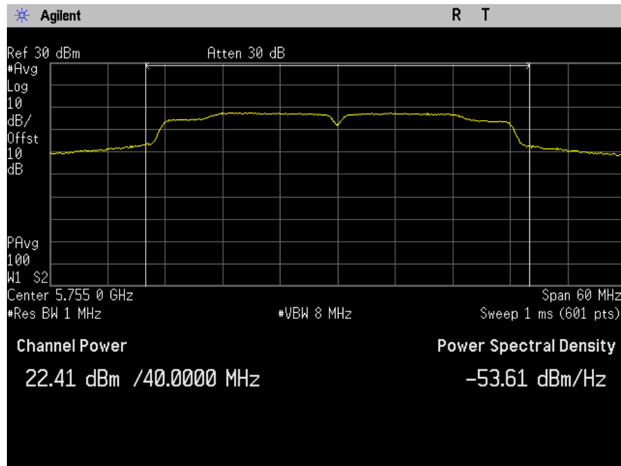
Plot 62. Maximum Conducted Output Power, MIMO, Bandwidth 40M, Ch. 5755M, ac mode, port b
