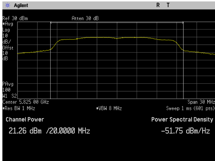
Plot 56. Maximum Conducted Output Power, MIMO, Bandwidth 20M, Ch. 5825M, a mode, port b
