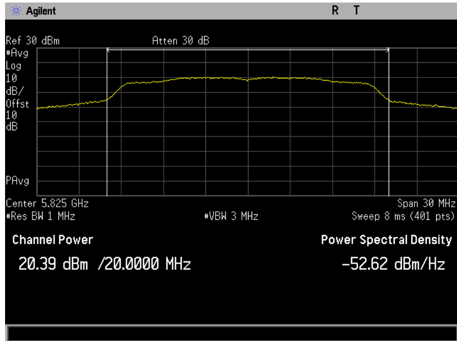
Plot 31. Maximum Conducted Output Power, SISO, Bandwidth 20M, Ch. 5825M, ac mode, port a
