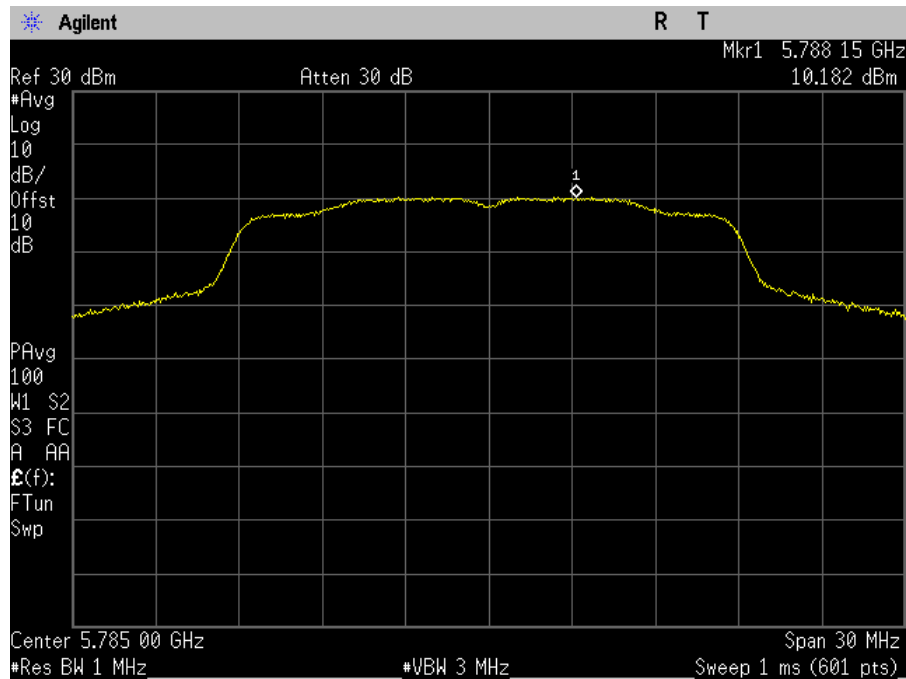
Plot 110. Power Spectral Density, MIMO, Bandwidth 20M, Ch. 5785M, n mode, port b
