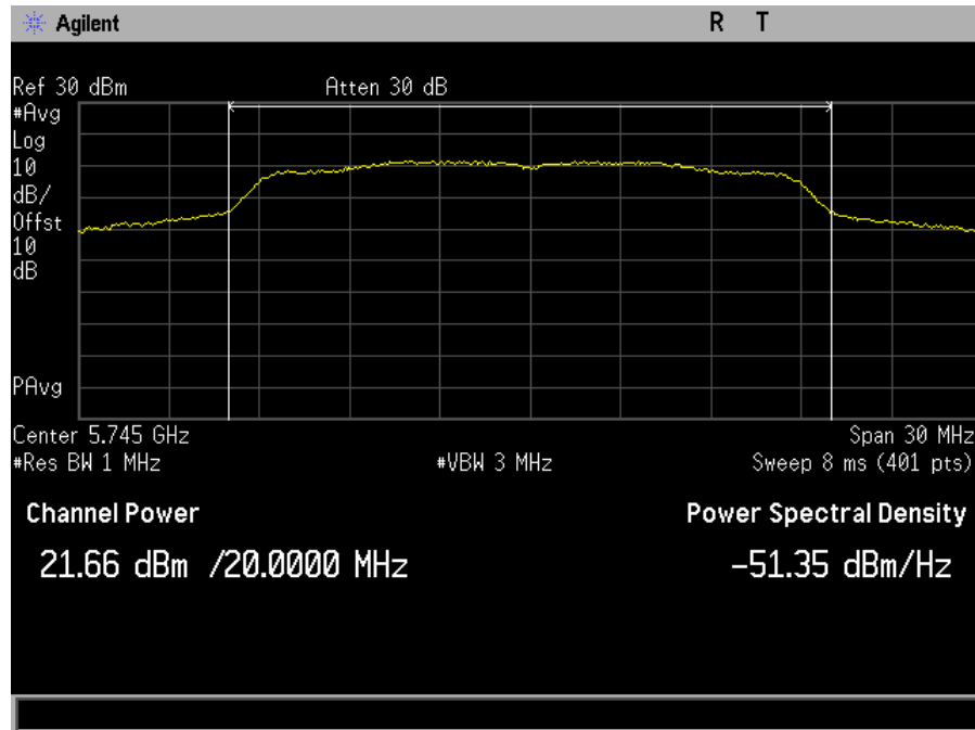
Plot 45. Maximum Conducted Output Power, MIMO, Bandwidth 20M, Ch. 5745M, ac mode, port a
