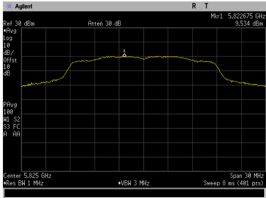
Plot 83. Power Spectral Density, SISO, Bandwidth 20M, Ch. 5825M, a mode, port a
