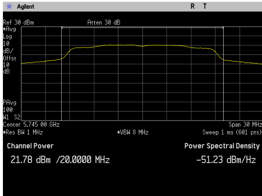
Plot 20. Maximum Conducted Output Power, SISO, Bandwidth 20M, Ch. 5745M, n mode, port b
