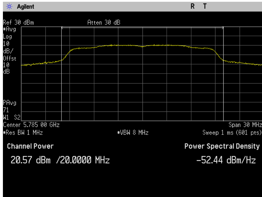
Plot 22. Maximum Conducted Output Power, SISO, Bandwidth 20M, Ch. 5785M, a mode, port b
