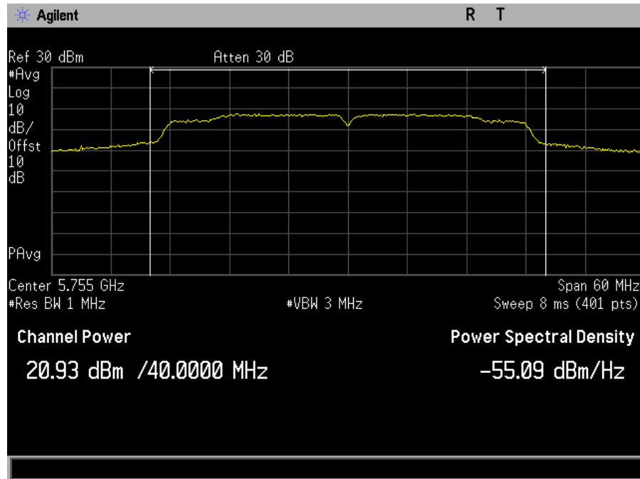
Plot 33. Maximum Conducted Output Power, SISO, Bandwidth 40M, Ch. 5755M, ac mode, port a
