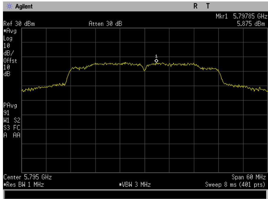
Plot 95. Power Spectral Density, SISO, Bandwidth 40M, Ch. 5795M, n mode, port a
