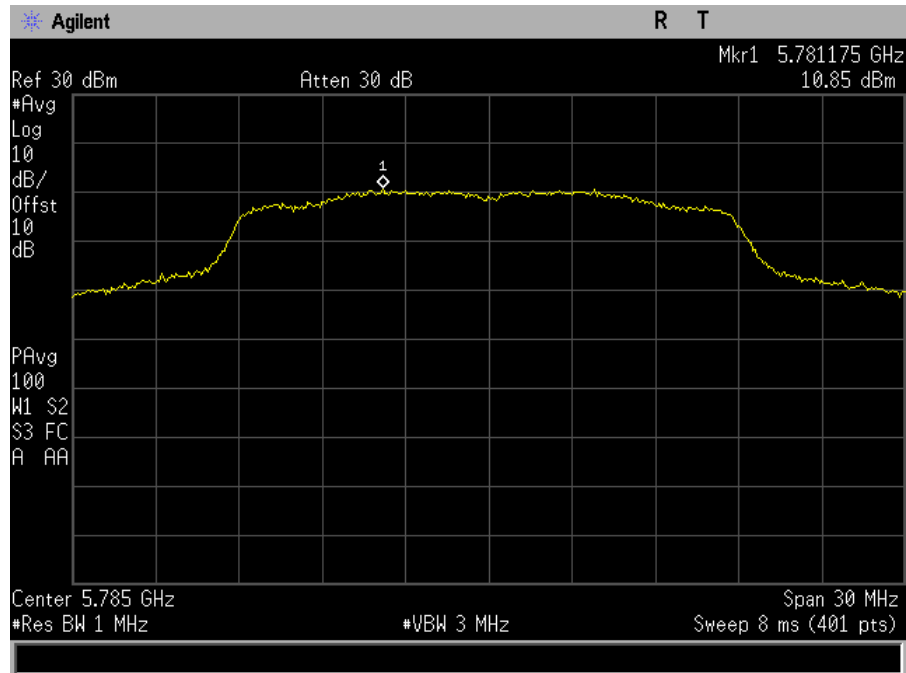
Plot 107. Power Spectral Density, MIMO, Bandwidth 20M, Ch. 5785M, ac mode, port a
