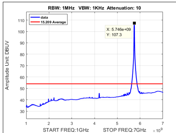
Plot 146. Undesirable Emissions, Average Radiated Spurious Emissions, MIMO, Bandwidth 20MHz, Ch. 5745, a mode, 1-7GHz
