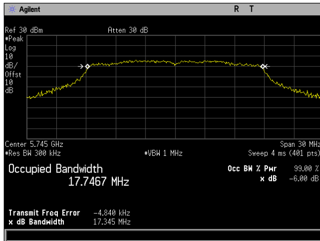
Plot 1. Occupied Bandwidth, 6dB, Bandwidth 20M, Ch. 5745M, a mode
