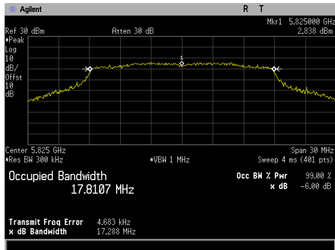
Plot 8. Occupied Bandwidth, 6dB, Bandwidth 20M, Ch. 5825M, ac mode
