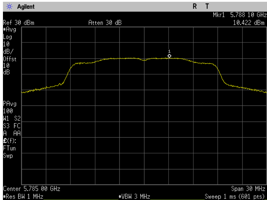
Plot 80. Power Spectral Density, SISO, Bandwidth 20M, Ch. 5785M, ac mode, port b
