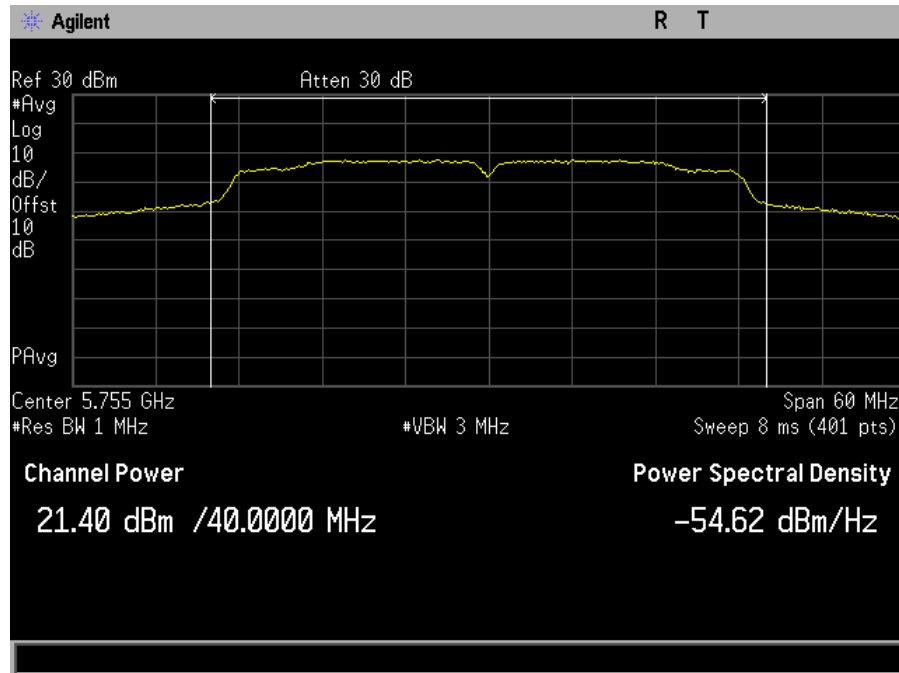
Plot 63. Maximum Conducted Output Power, MIMO, Bandwidth 40M, Ch. 5755M, n mode, port a
