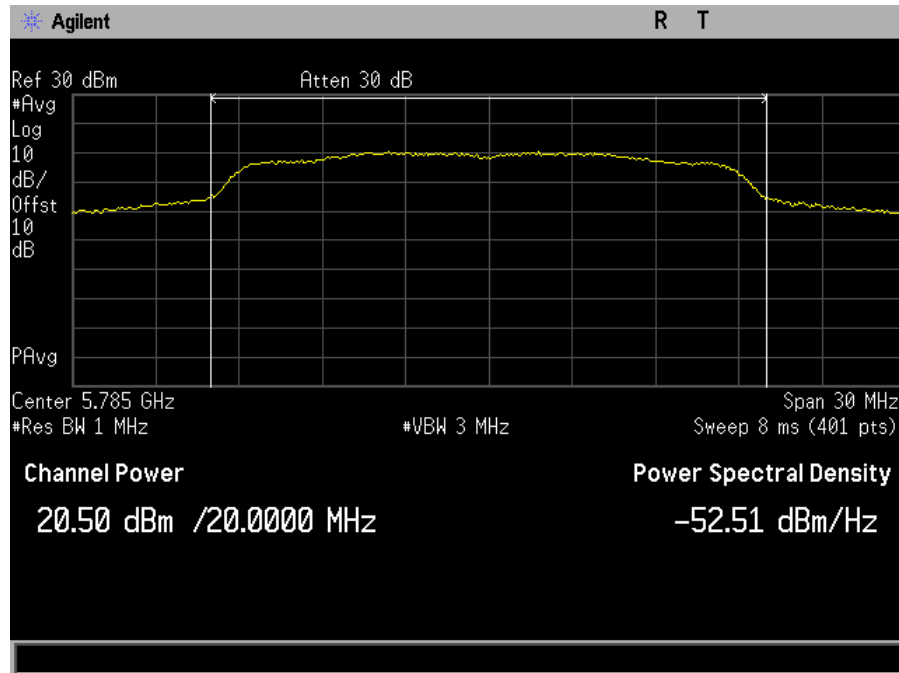
Plot 25. Maximum Conducted Output Power, SISO, Bandwidth 20M, Ch. 5785M, n mode, port a
