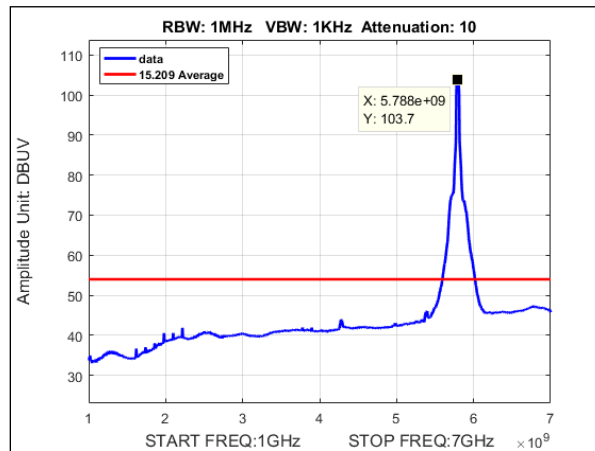
Plot 143. Undesirable Emissions, Average Radiated Spurious Emissions, MIMO, Bandwidth 40MHz, Ch. 5795, ac mode, 1-7GHz
