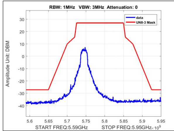
Plot 128. Undesirable Emissions, MIMO, Emissions Mask, Bandwidth 20M, Ch. 5745, a mode
