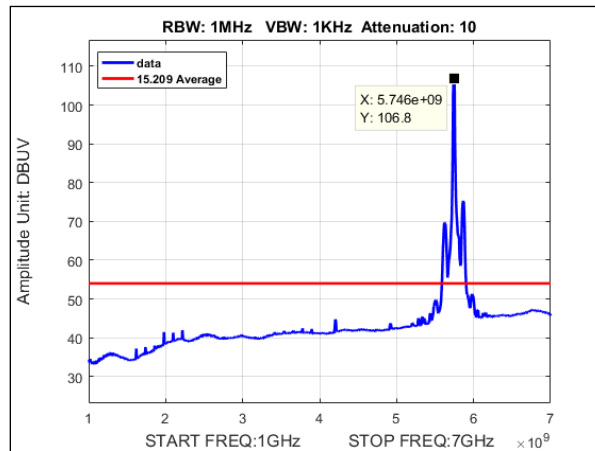
Plot 139. Undesirable Emissions, Average Radiated Spurious Emissions, MIMO, Bandwidth 20MHz, Ch. 5745, ac mode, 1-7GHz
