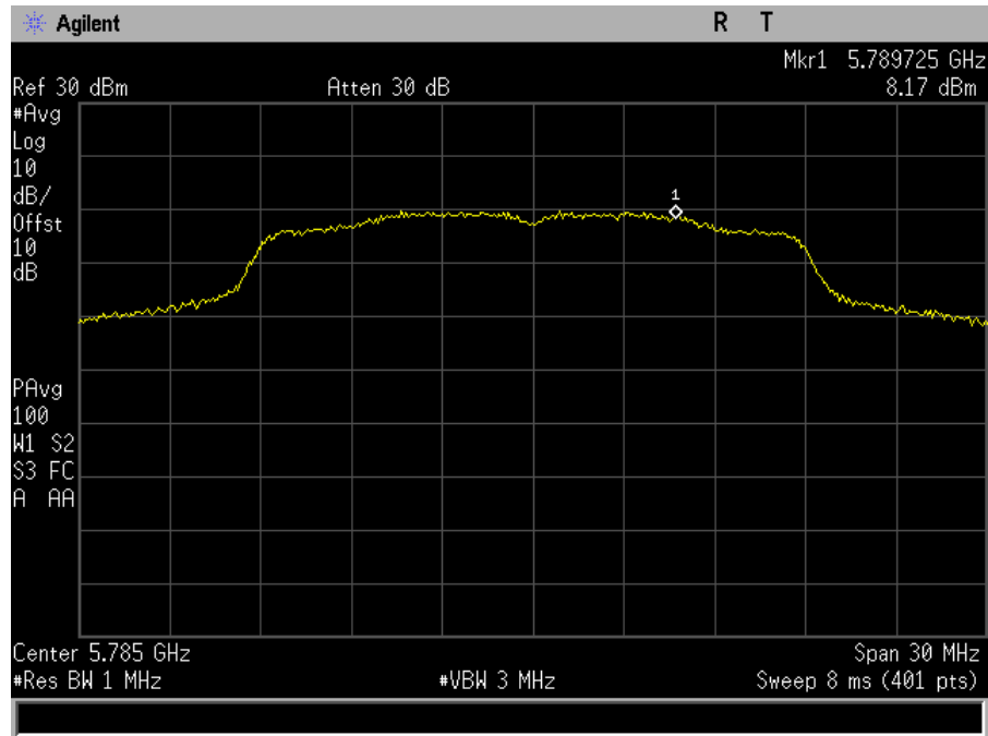
Plot 105. Power Spectral Density, MIMO, Bandwidth 20M, Ch. 5785M, a mode, port a
