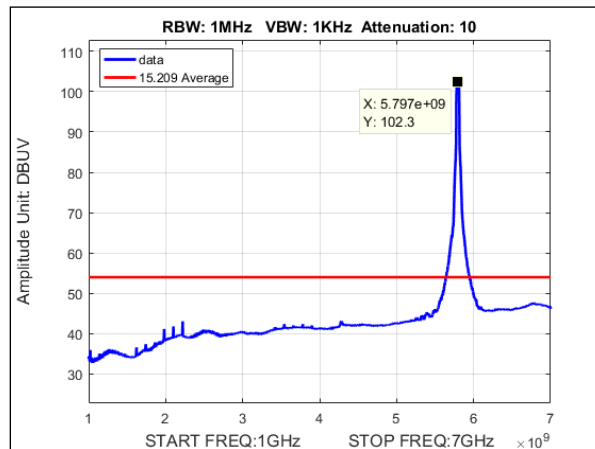
Plot 153. Undesirable Emissions, Average Radiated Spurious Emissions, MIMO, Bandwidth 40MHz, Ch. 5795, n mode, 1-7GHz
