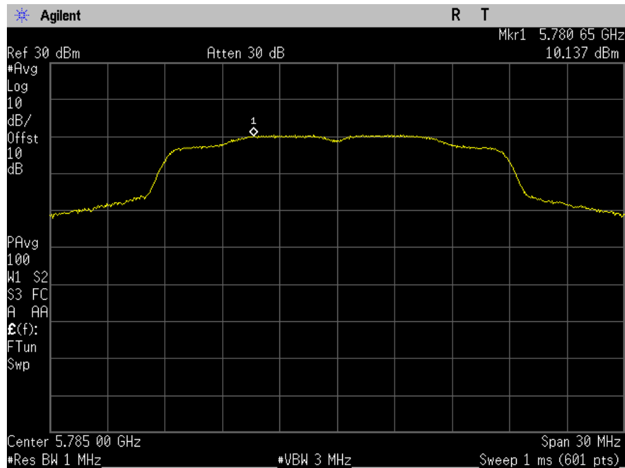
Plot 106. Power Spectral Density, MIMO, Bandwidth 20M, Ch. 5785M, a mode, port b
