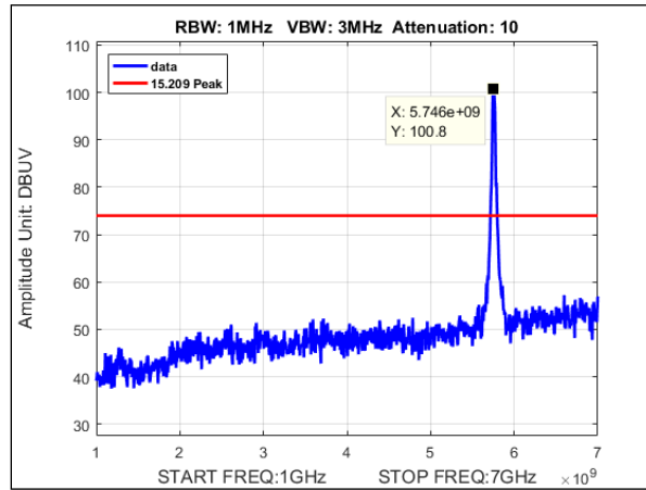
Plot 167. Undesirable Emissions, Peak Radiated Spurious Emissions, MIMO, Bandwidth 40M, Ch. 5755, n mode, 1-7GHz
