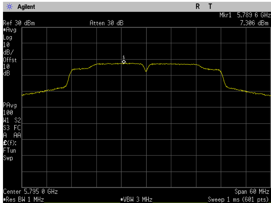
Plot 96. Power Spectral Density, SISO, Bandwidth 40M, Ch. 5795M, n mode, port b
