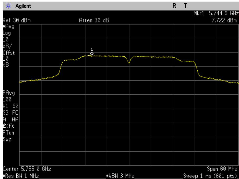
Plot 120. Power Spectral Density, MIMO, Bandwidth 40M, Ch. 5755M, n mode, port b
