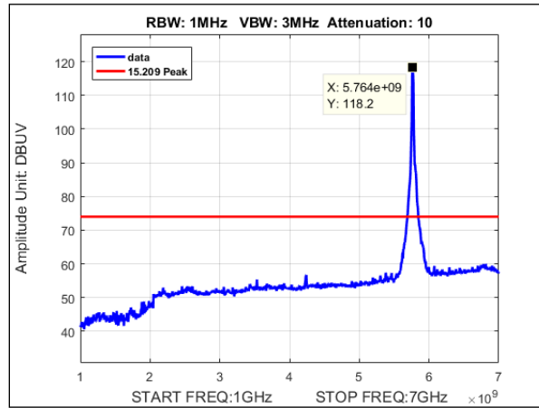
Plot 158. Undesirable Emissions, Peak Radiated Spurious Emissions, MIMO, Bandwidth 20M, Ch. 5765, ac mode, 1-7GHz
