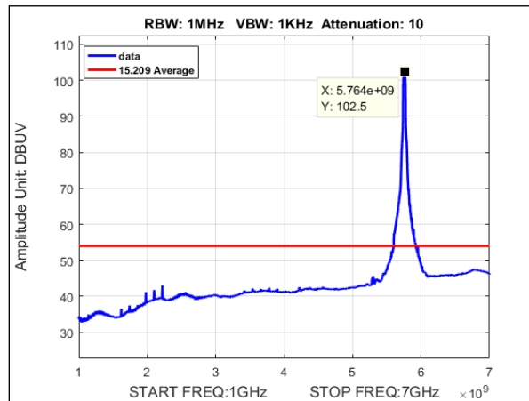
Plot 152. Undesirable Emissions, Average Radiated Spurious Emissions, MIMO, Bandwidth 40MHz, Ch. 5755, n mode, 1-7GHz
