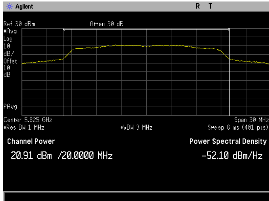
Plot 57. Maximum Conducted Output Power, MIMO, Bandwidth 20M, Ch. 5825M, ac mode, port a
