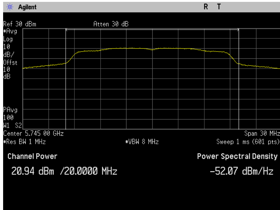
Plot 18. Maximum Conducted Output Power, SISO, Bandwidth 20M, Ch. 5745M, ac mode, port b
