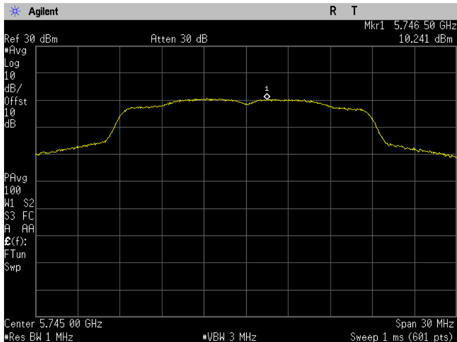
Plot 100. Power Spectral Density, MIMO, Bandwidth 20M, Ch. 5745M, a mode, port b
