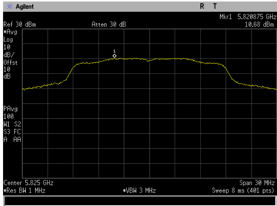
Plot 113. Power Spectral Density, MIMO, Bandwidth 20M, Ch. 5825M, ac mode, port a
