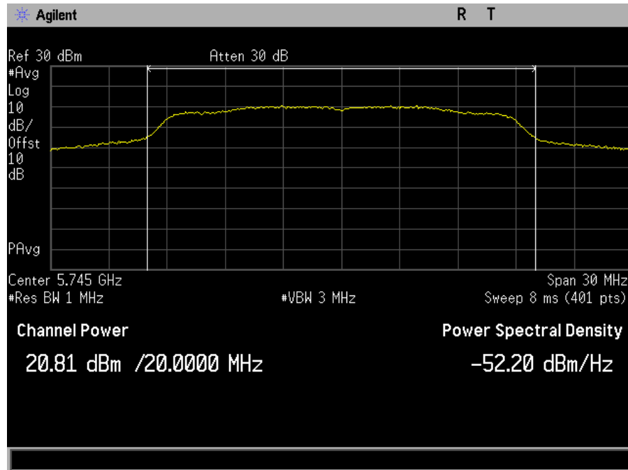
Plot 19. Maximum Conducted Output Power, SISO, Bandwidth 20M, Ch. 5745M, n mode, port a
