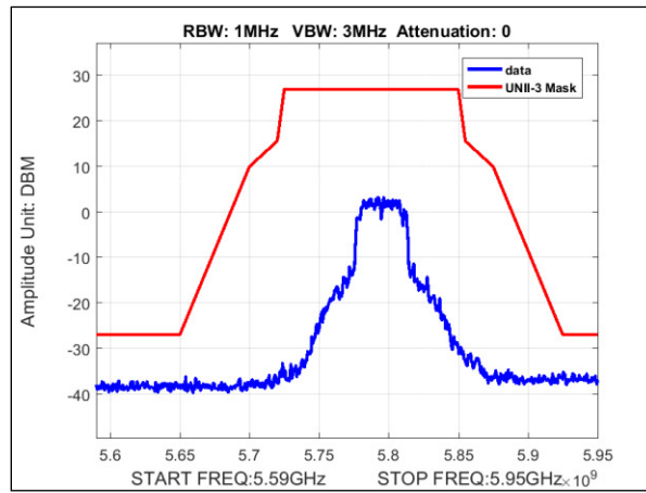
Plot 137. Undesirable Emissions, MIMO, Emissions Mask, Bandwidth 40M, Ch. 5795, n mode
