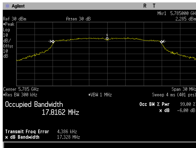
Plot 6. Occupied Bandwidth, 6dB, Bandwidth 20M, Ch. 5785M, n mode
