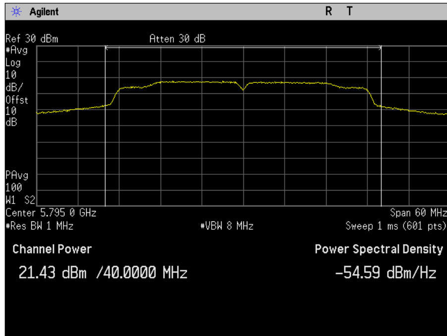
Plot 37. Maximum Conducted Output Power, SISO, Bandwidth 40M, Ch. 5795M, ac mode, port b
