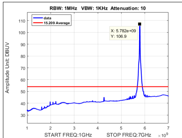
Plot 140. Undesirable Emissions, Average Radiated Spurious Emissions, MIMO, Bandwidth 20MHz, Ch. 5785, ac mode, 1-7GHz
