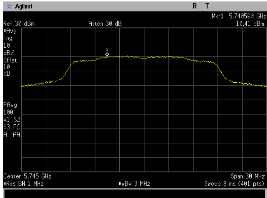
Plot 73. Power Spectral Density, SISO, Bandwidth 20M, Ch. 5745M, ac mode, port a
