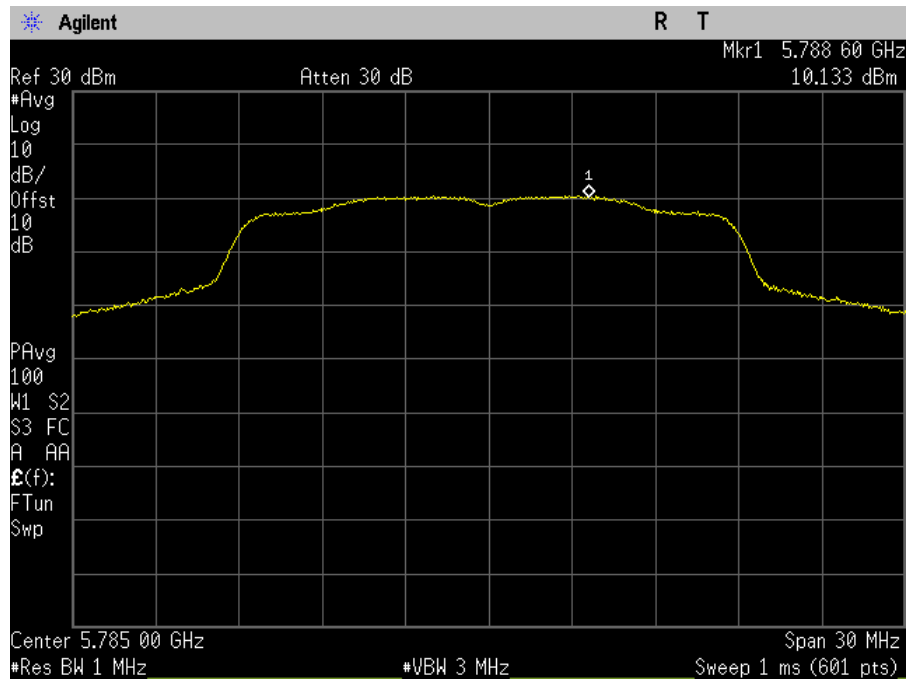
Plot 78. Power Spectral Density, SISO, Bandwidth 20M, Ch. 5785M, a mode, port b
