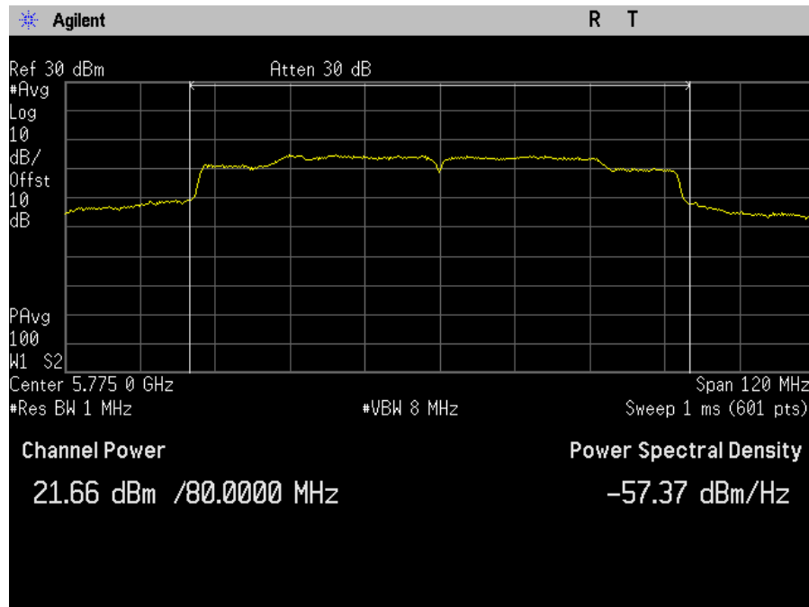
Plot 70. Maximum Conducted Output Power, MIMO, Bandwidth 80M, Ch. 5775M, ac mode, port b
