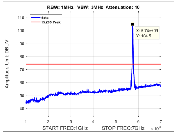
Plot 154. Undesirable Emissions, Peak Radiated Spurious Emissions, MIMO, Bandwidth 20M, Ch. 5745, a mode, 1-7GHz
