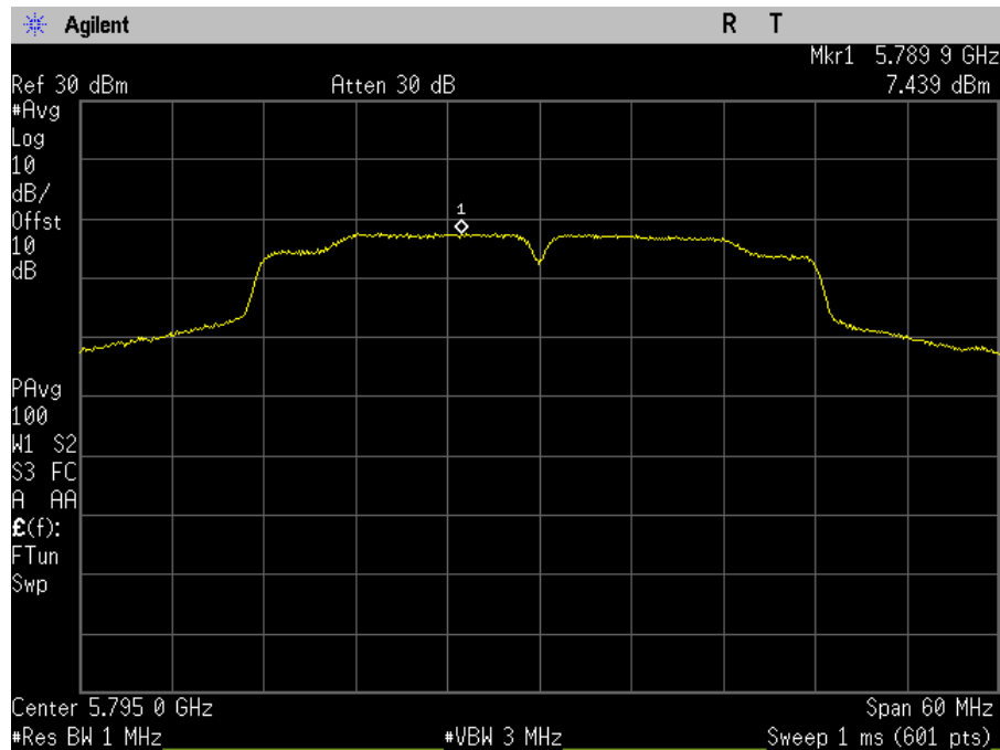
Plot 94. Power Spectral Density, SISO, Bandwidth 40M, Ch. 5795M, ac mode, port b
