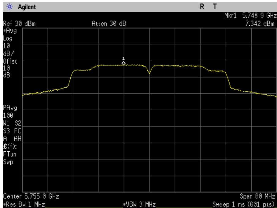
Plot 90. Power Spectral Density, SISO, Bandwidth 40M, Ch. 5755M, ac mode, port b
