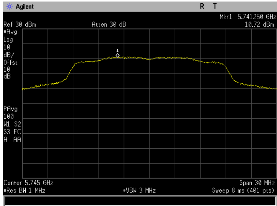
Plot 103. Power Spectral Density, MIMO, Bandwidth 20M, Ch. 5745M, n mode, port a
