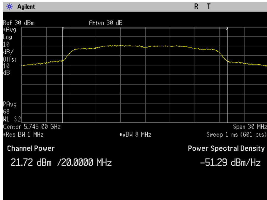
Plot 46. Maximum Conducted Output Power, MIMO, Bandwidth 20M, Ch. 5745M, ac mode, port b
