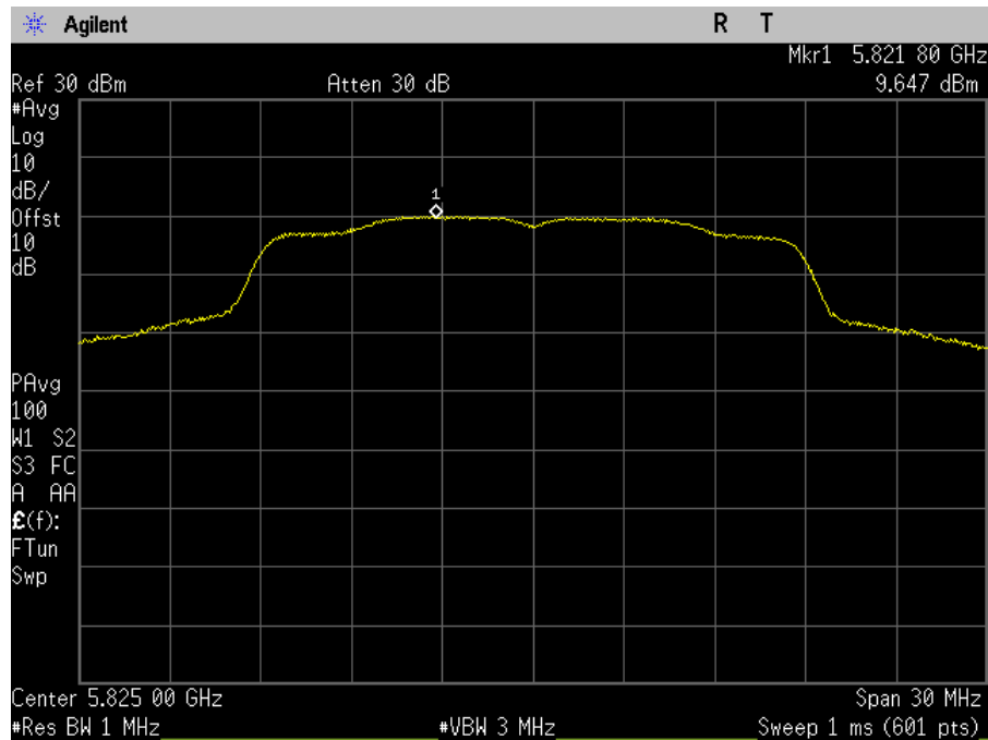
Plot 86. Power Spectral Density, SISO, Bandwidth 20M, Ch. 5825M, ac mode, port b
