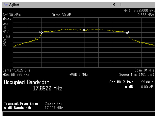
Plot 9. Occupied Bandwidth, 6dB, Bandwidth 20M, Ch. 5825M, n mode
