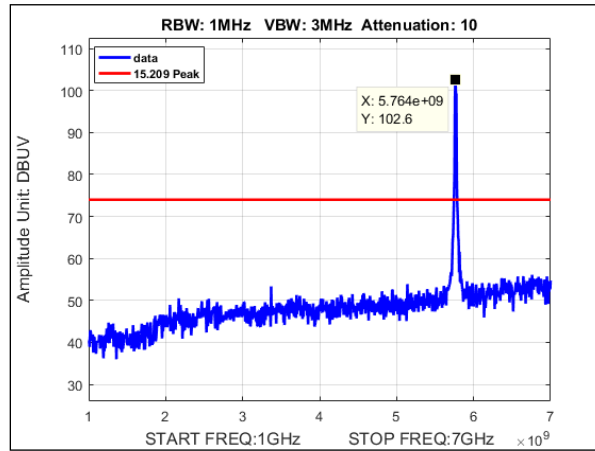
Plot 155. Undesirable Emissions, Peak Radiated Spurious Emissions, MIMO, Bandwidth 20M, Ch. 5765, a mode, 1-7GHz
