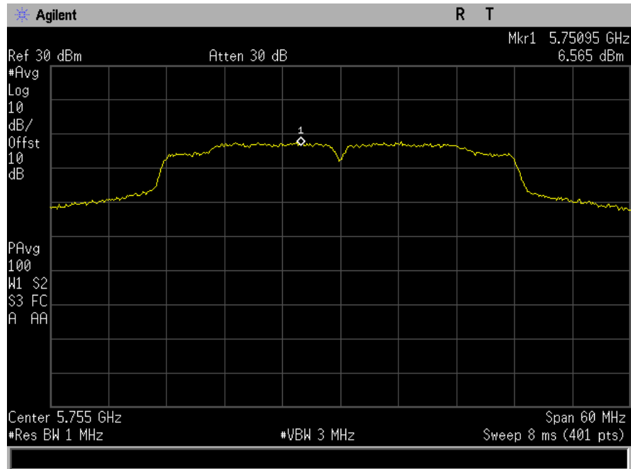
Plot 119. Power Spectral Density, MIMO, Bandwidth 40M, Ch. 5755M, n mode, port a
