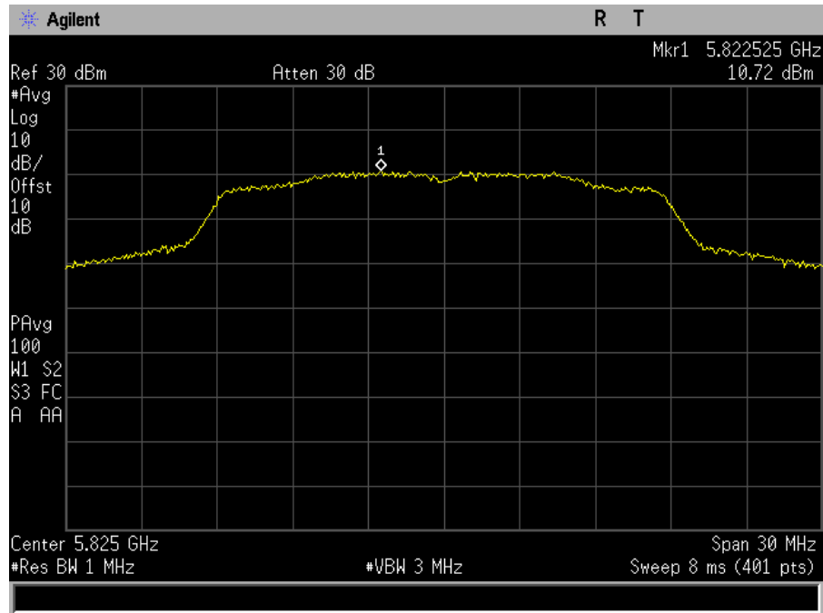
Plot 111. Power Spectral Density, MIMO, Bandwidth 20M, Ch. 5825M, a mode, port a
