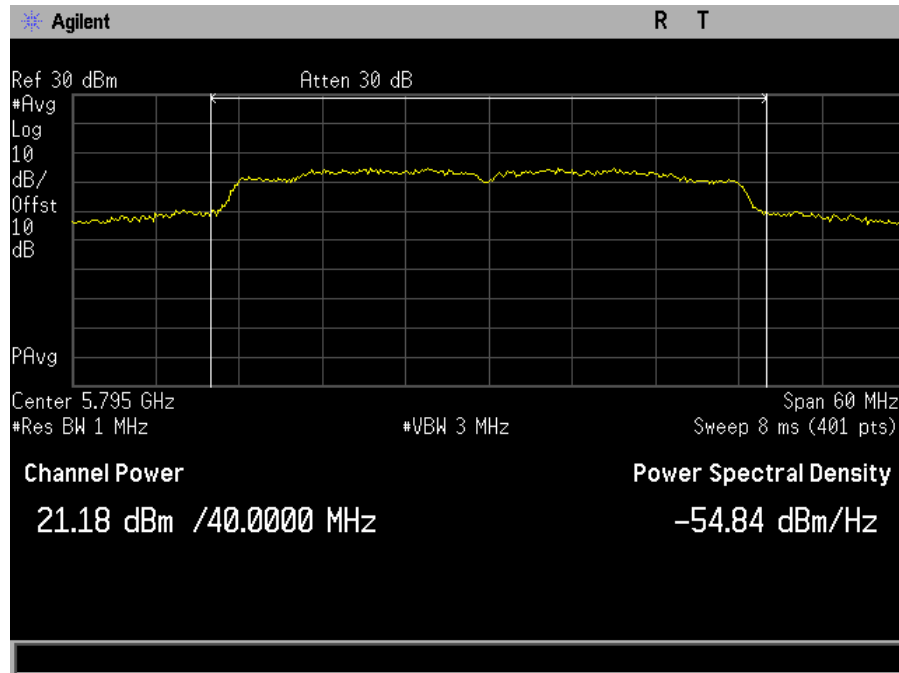
Plot 65. Maximum Conducted Output Power, MIMO, Bandwidth 40M, Ch. 5795M, ac mode, port a
