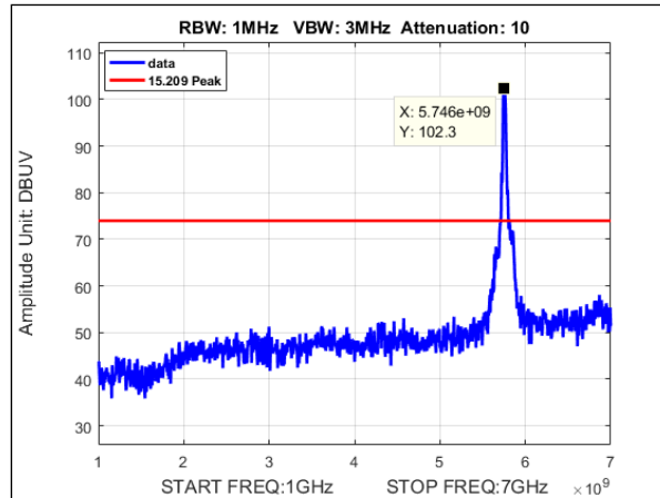
Plot 160. Undesirable Emissions, Peak Radiated Spurious Emissions, MIMO, Bandwidth 40M, Ch. 5755, ac mode, 1-7GHz
