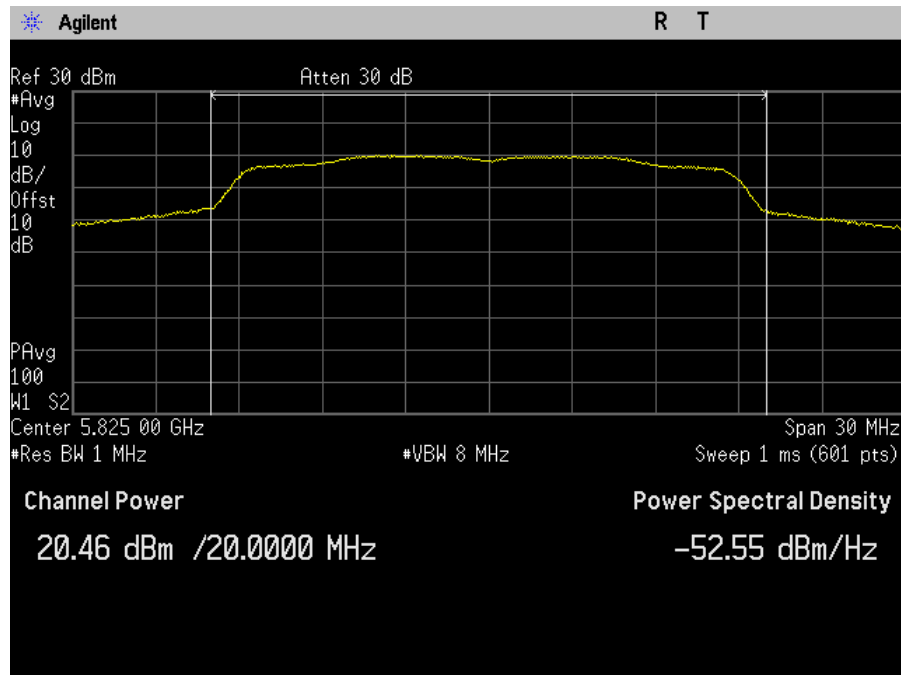
Plot 32. Maximum Conducted Output Power, SISO, Bandwidth 20M, Ch. 5825M, ac mode, port b
