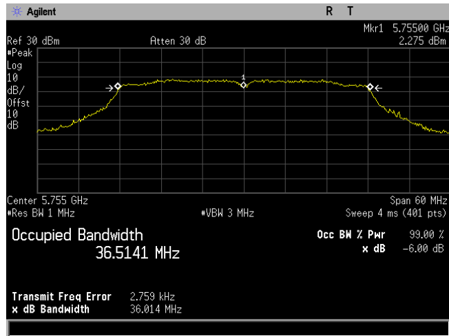
Plot 10. Occupied Bandwidth, 6dB, Bandwidth 40M, Ch. 5755M, ac mode
