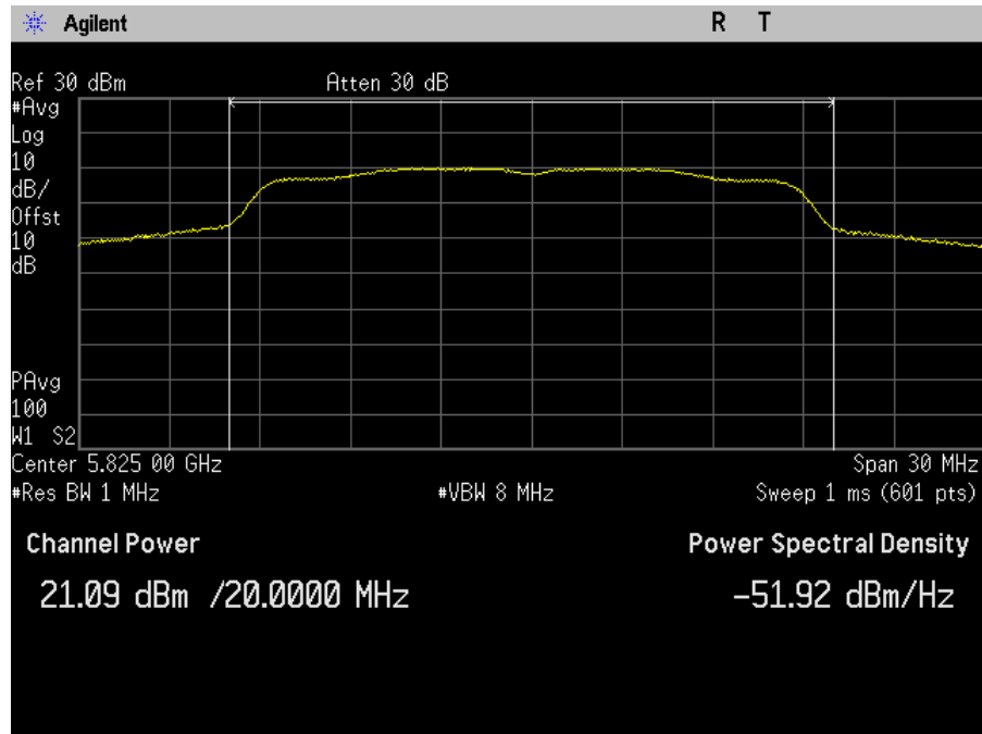
Plot 29. Maximum Conducted Output Power, SISO, Bandwidth 20M, Ch. 5825M, n mode, port b
