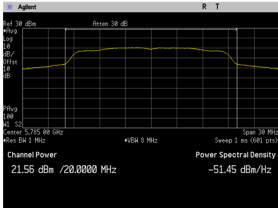
Plot 54. Maximum Conducted Output Power, MIMO, Bandwidth 20M, Ch. 5785M, n mode, port b
