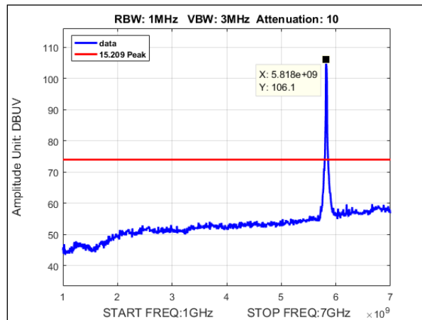
Plot 156. Undesirable Emissions, Peak Radiated Spurious Emissions, MIMO, Bandwidth 20M, Ch. 5825, a mode, 1-7GHz
