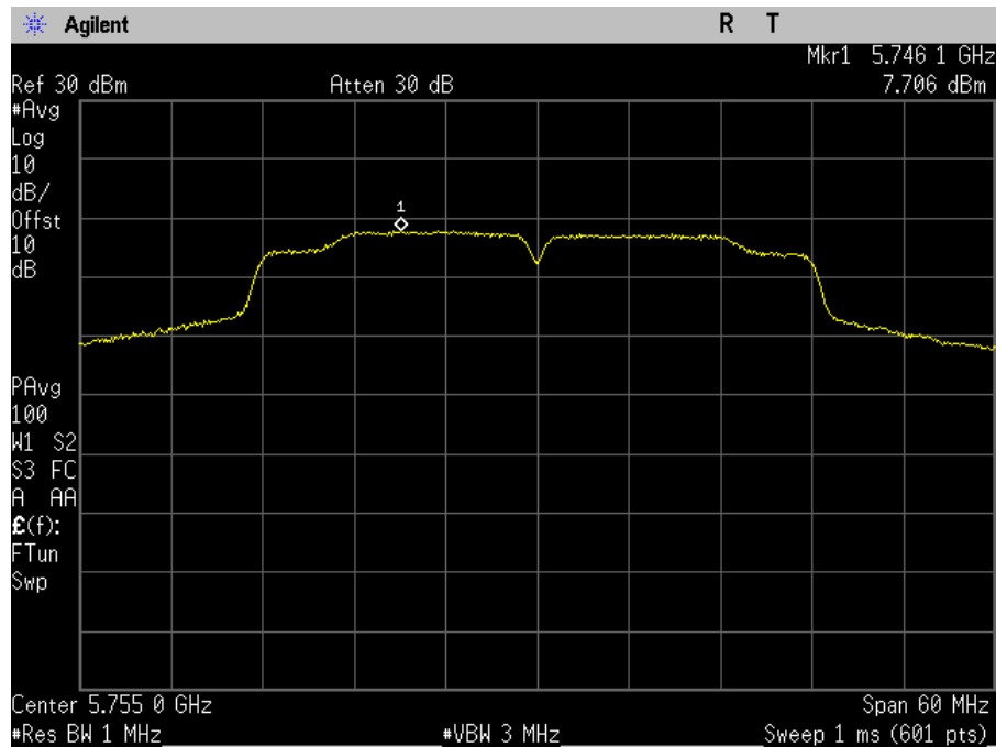
Plot 118. Power Spectral Density, MIMO, Bandwidth 40M, Ch. 5755M, ac mode, port b
