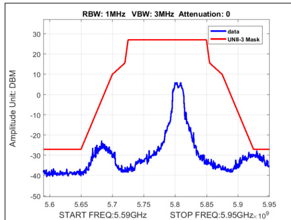
Plot 134. Undesirable Emissions, MIMO, Emissions Mask, Bandwidth 20M, Ch. 5805, ac mode
