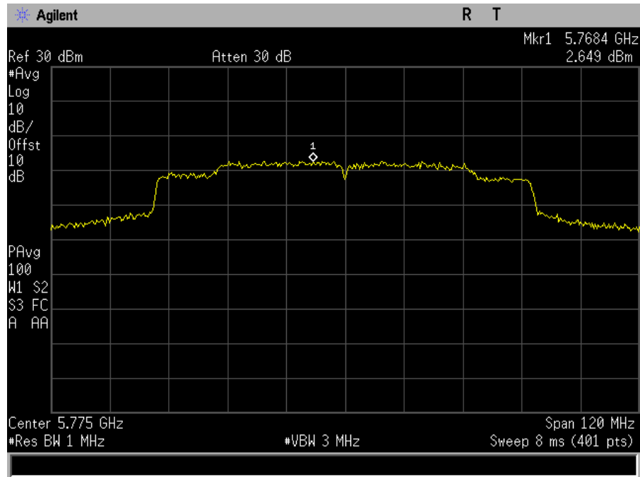
Plot 97. Power Spectral Density, SISO, Bandwidth 80M, Ch. 5775M, ac mode, port a
