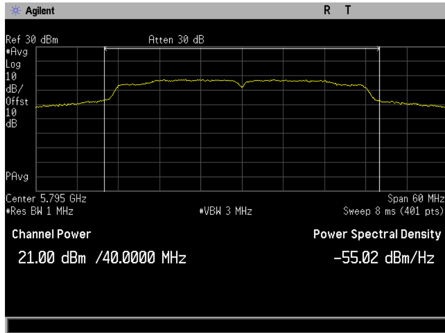
Plot 39. Maximum Conducted Output Power, SISO, Bandwidth 40M, Ch. 5795M, n mode, port a
