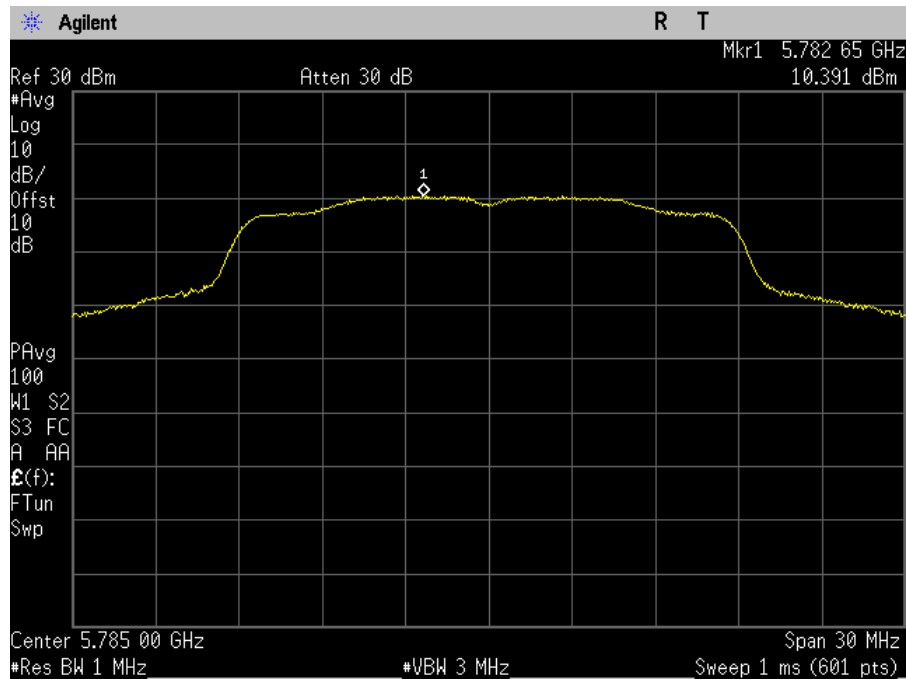
Plot 108. Power Spectral Density, MIMO, Bandwidth 20M, Ch. 5785M, ac mode, port b
