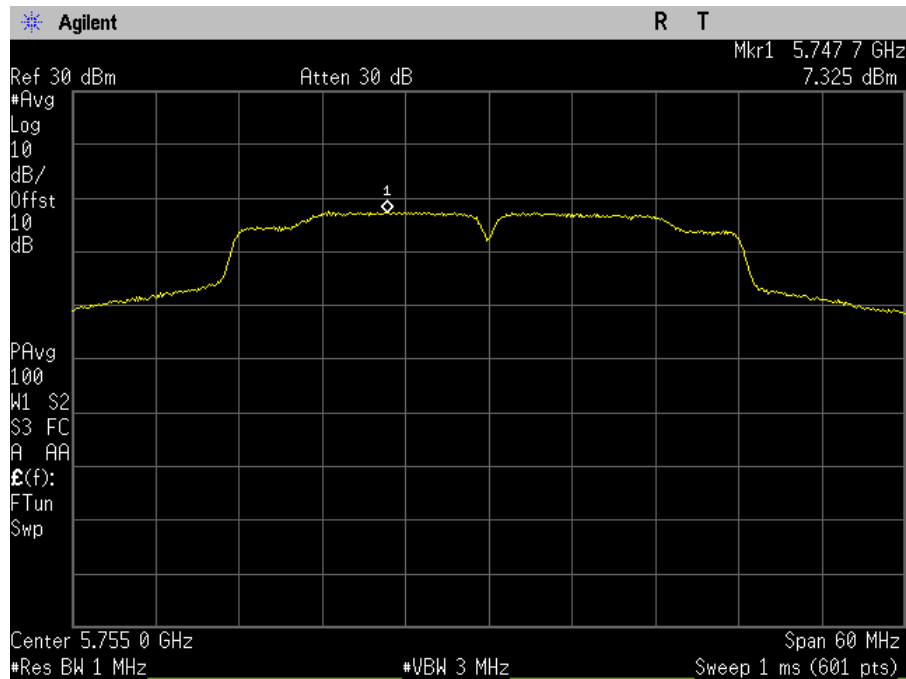
Plot 92. Power Spectral Density, SISO, Bandwidth 40M, Ch. 5755M, n mode, port b
