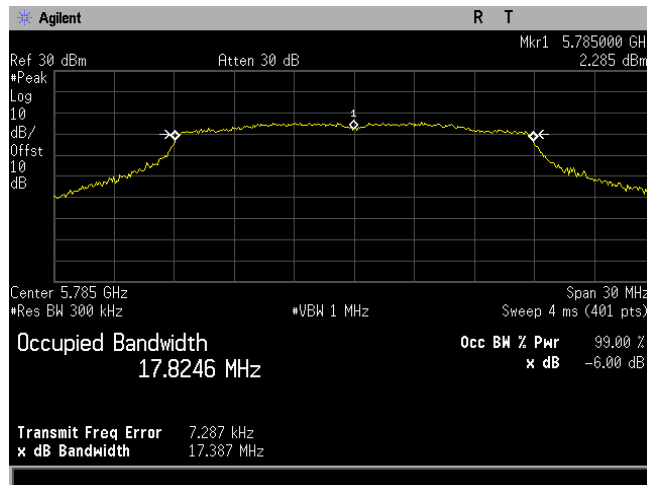
Plot 5. Occupied Bandwidth, 6dB, Bandwidth 20M, Ch. 5785M, ac mode
