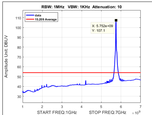
Plot 149. Undesirable Emissions, Average Radiated Spurious Emissions, MIMO, Bandwidth 20MHz, Ch. 5745, n mode, 1-7GHz
