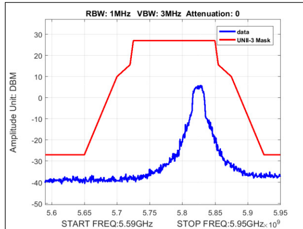
Plot 129. Undesirable Emissions, MIMO, Emissions Mask, Bandwidth 20M, Ch. 5825, a mode
