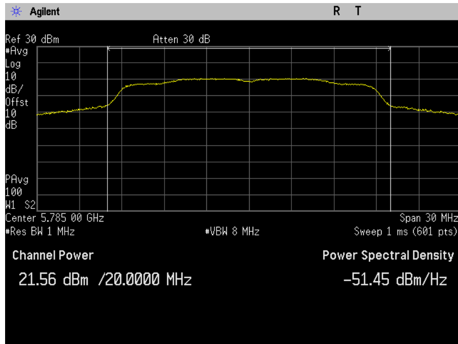
Plot 24. Maximum Conducted Output Power, SISO, Bandwidth 20M, Ch. 5785M, ac mode, port b
