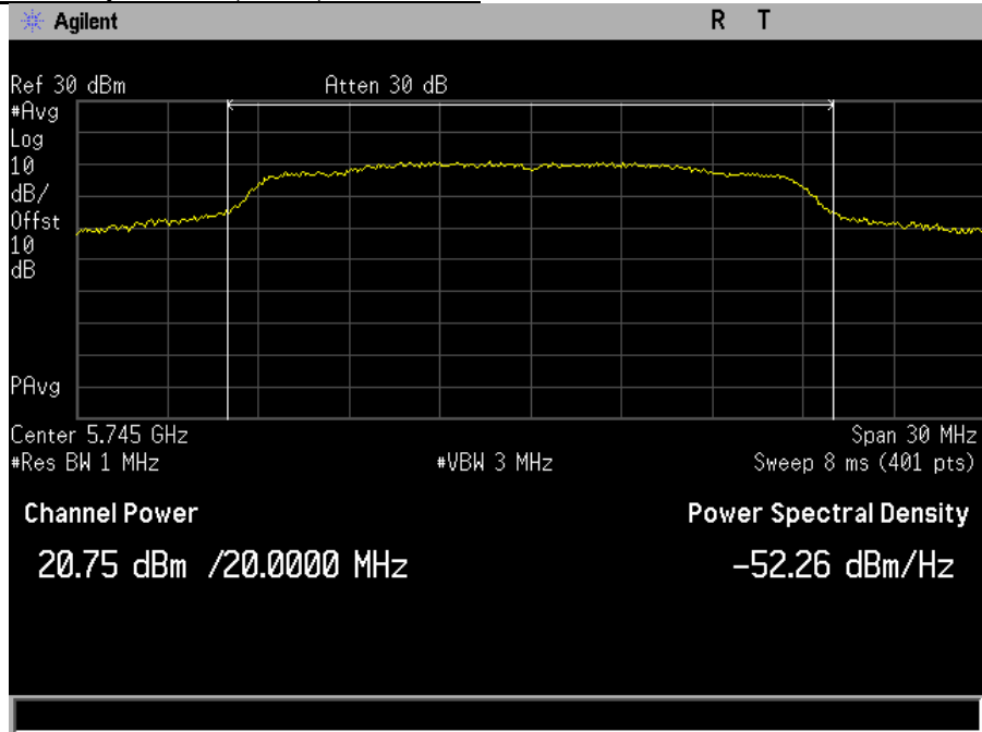
Plot 15. Maximum Conducted Output Power, SISO, Bandwidth 20M, Ch. 5745M, a mode, port a
