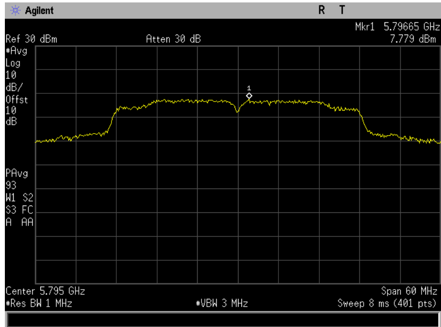
Plot 121. Power Spectral Density, MIMO, Bandwidth 40M, Ch. 5795M, ac mode, port a
