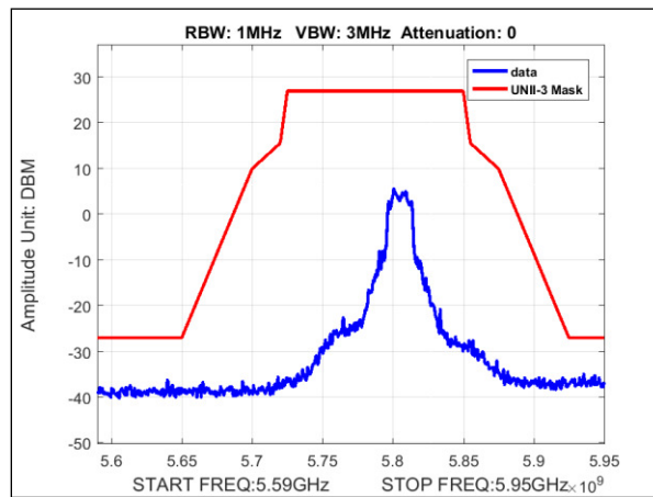
Plot 138. Undesirable Emissions, MIMO, Emissions Mask, Bandwidth 20M, Ch. 5805, n mode
