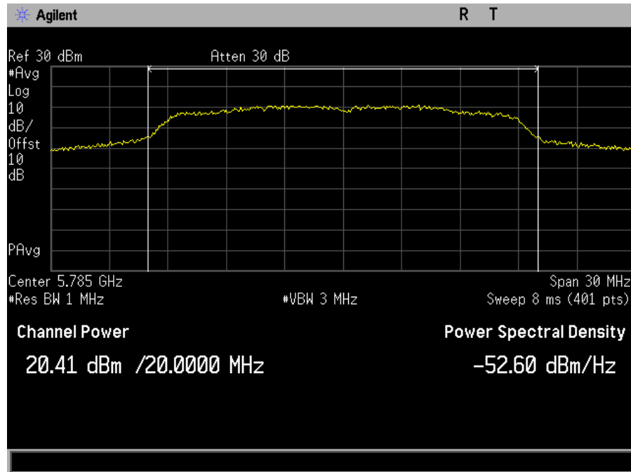
Plot 53. Maximum Conducted Output Power, MIMO, Bandwidth 20M, Ch. 5785M, n mode, port a
