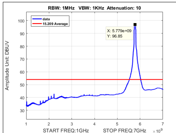
Plot 144. Undesirable Emissions, Average Radiated Spurious Emissions, MIMO, Bandwidth 80MHz, Ch. 5775M, ac mode, 1-7GHz
