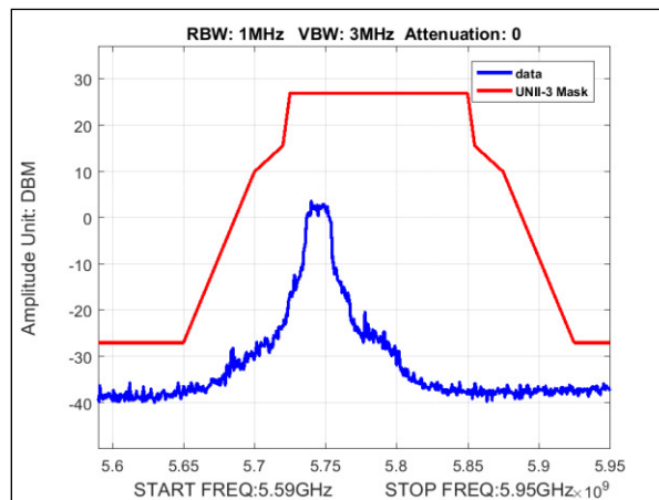
Plot 130. Undesirable Emissions, MIMO, Emissions Mask, Bandwidth 20M, Ch. 5745, ac mode
