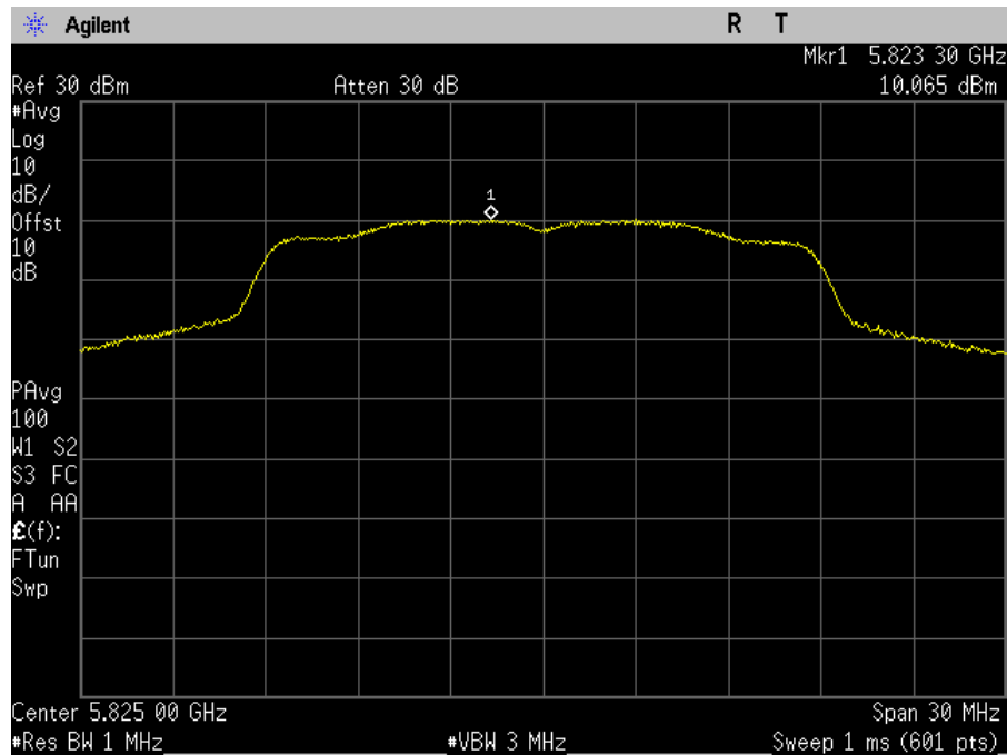
Plot 116. Power Spectral Density, MIMO, Bandwidth 20M, Ch. 5825M, n mode, port b
