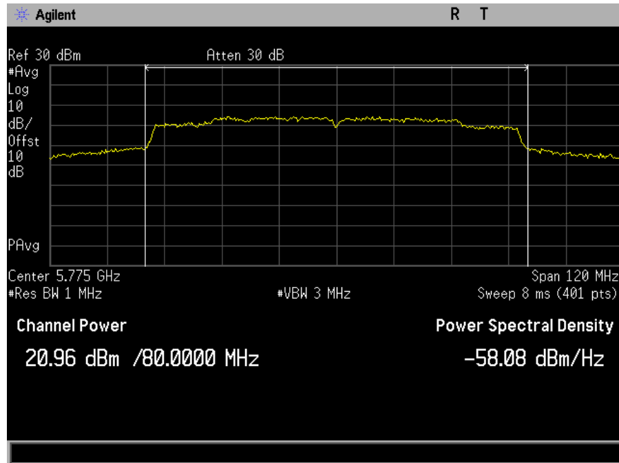
Plot 69. Maximum Conducted Output Power, MIMO, Bandwidth 80M, Ch. 5775M, ac mode, port a
