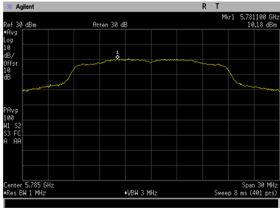
Plot 79. Power Spectral Density, SISO, Bandwidth 20M, Ch. 5785M, ac mode, port a
