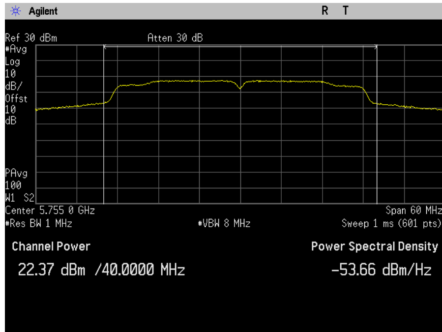
Plot 34. Maximum Conducted Output Power, SISO, Bandwidth 40M, Ch. 5755M, ac mode, port b
