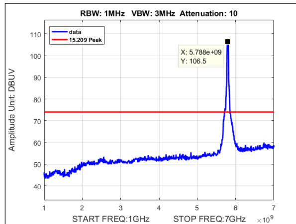
Plot 161. Undesirable Emissions, Peak Radiated Spurious Emissions, MIMO, Bandwidth 40M, Ch. 5795, ac mode, 1-7GHz
