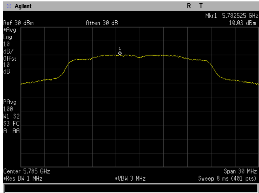
Plot 77. Power Spectral Density, SISO, Bandwidth 20M, Ch. 5785M, a mode, port a
