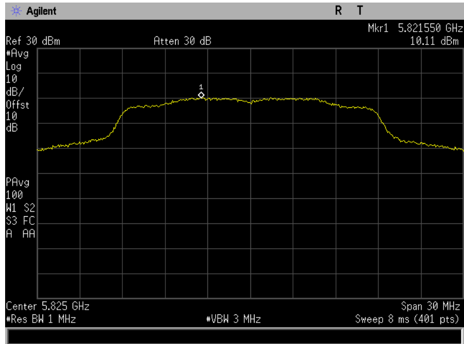
Plot 85. Power Spectral Density, SISO, Bandwidth 20M, Ch. 5825M, ac mode, port a
