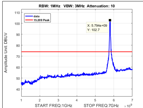
Plot 168. Undesirable Emissions, Peak Radiated Spurious Emissions, MIMO, Bandwidth 40M, Ch. 5795, n mode, 1-7GHz
