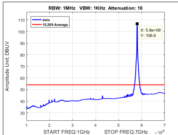
Plot 151. Undesirable Emissions, Average Radiated Spurious Emissions, MIMO, Bandwidth 20MHz, Ch. 5805, n mode, 1-7GHz
