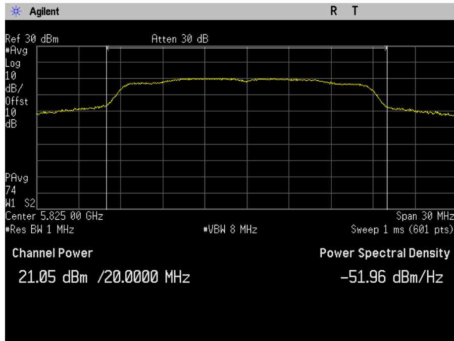
Plot 58. Maximum Conducted Output Power, MIMO, Bandwidth 20M, Ch. 5825M, ac mode, port b
