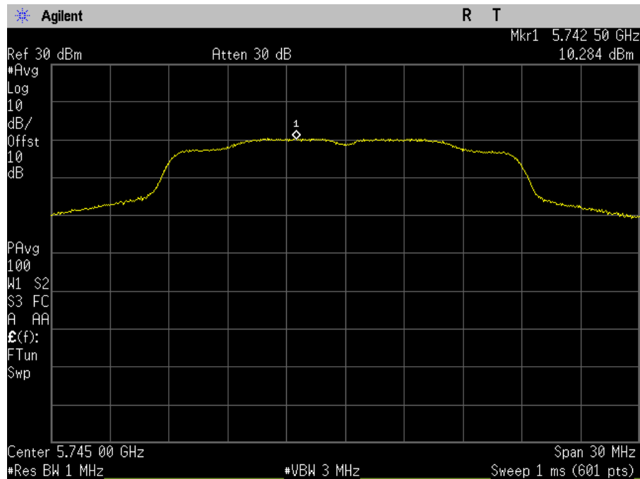
Plot 74. Power Spectral Density, SISO, Bandwidth 20M, Ch. 5745M, ac mode, port b
