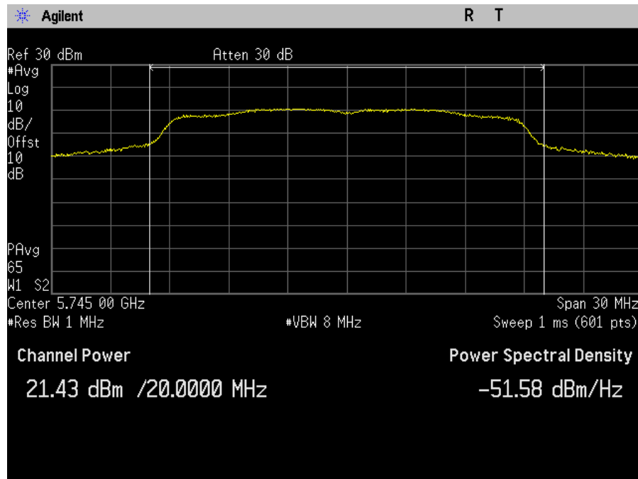
Plot 48. Maximum Conducted Output Power, MIMO, Bandwidth 20M, Ch. 5745M, n mode, port b
