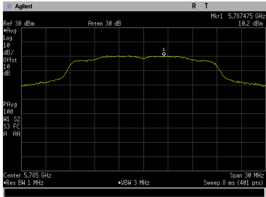
Plot 109. Power Spectral Density, MIMO, Bandwidth 20M, Ch. 5785M, n mode, port a
