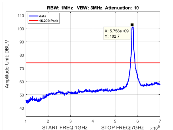
Plot 162. Undesirable Emissions, Peak Radiated Spurious Emissions, MIMO, Bandwidth 80M, Ch. 5775, ac mode, 1-7GHz
