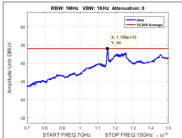
Plot 145. Undesirable Emissions, Average Radiated Spurious Emissions, MIMO, Bandwidth 80MHz, Ch. 5775, ac mode, 7-15GHz
