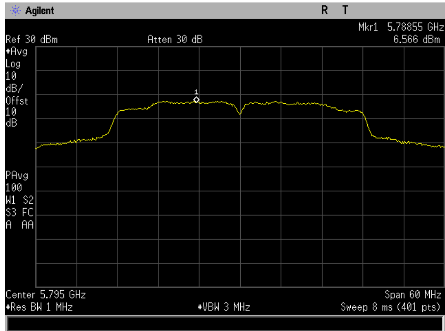
Plot 93. Power Spectral Density, SISO, Bandwidth 40M, Ch. 5795M, ac mode, port a
