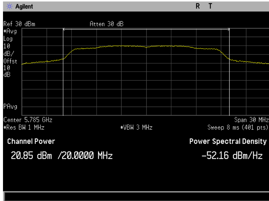
Plot 23. Maximum Conducted Output Power, SISO, Bandwidth 20M, Ch. 5785M, ac mode, port a
