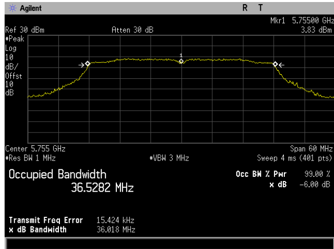
Plot 11. Occupied Bandwidth, 6dB, Bandwidth 40M, Ch. 5755M, n mode
