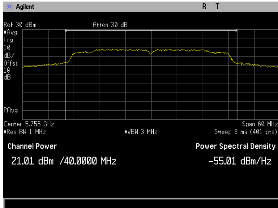
Plot 61. Maximum Conducted Output Power, MIMO, Bandwidth 40M, Ch. 5755M, ac mode, port a
