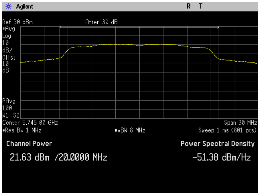
Plot 16. Maximum Conducted Output Power, SISO, Bandwidth 20M, Ch. 5745M, a mode, port b
