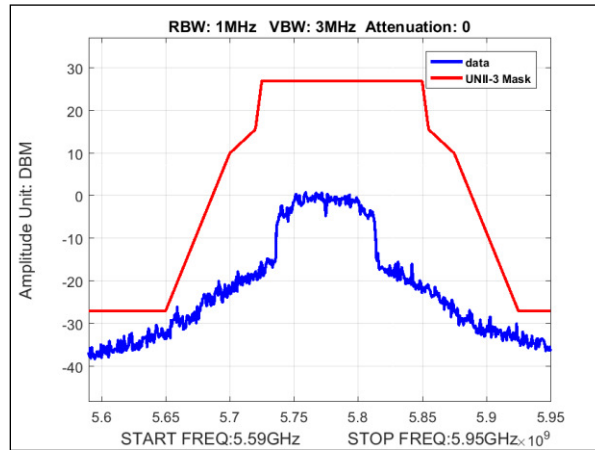
Plot 132. Undesirable Emissions, MIMO, Emissions Mask, Bandwidth 80M, Ch. 5775, ac mode
