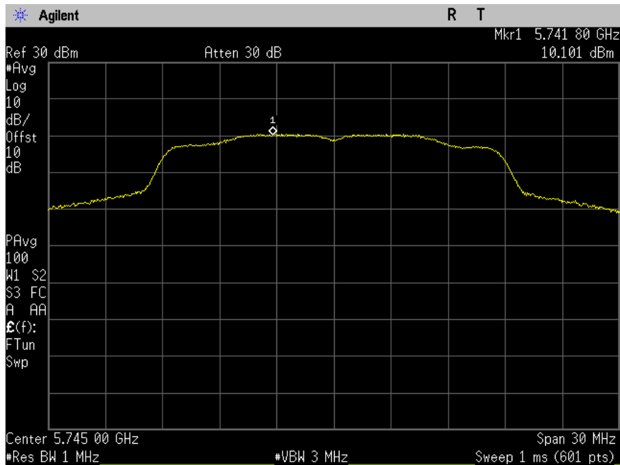
Plot 72. Power Spectral Density, SISO, Bandwidth 20M, Ch. 5745M, a mode, port b
