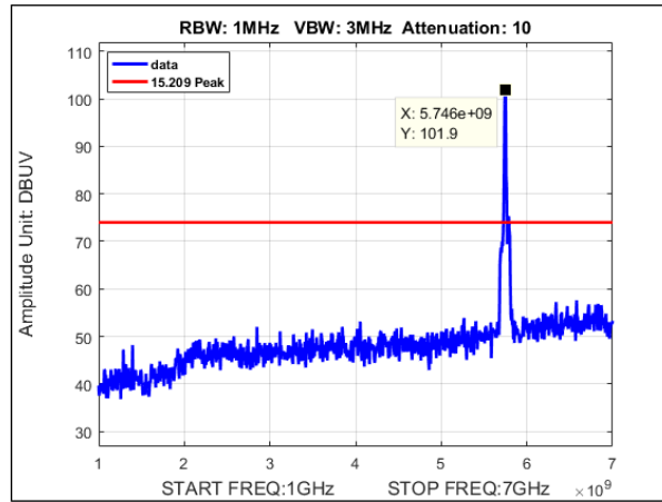
Plot 164. Undesirable Emissions, Peak Radiated Spurious Emissions, MIMO, Bandwidth 20M, Ch. 5745, n mode, 1-7GHz
