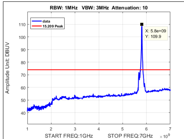
Plot 159. Undesirable Emissions, Peak Radiated Spurious Emissions, MIMO, Bandwidth 20M, Ch. 5805, ac mode, 1-7GHz
