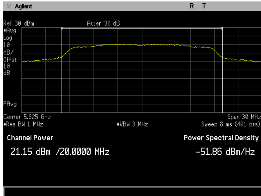
Plot 55. Maximum Conducted Output Power, MIMO, Bandwidth 20M, Ch. 5825M, a mode, port a
