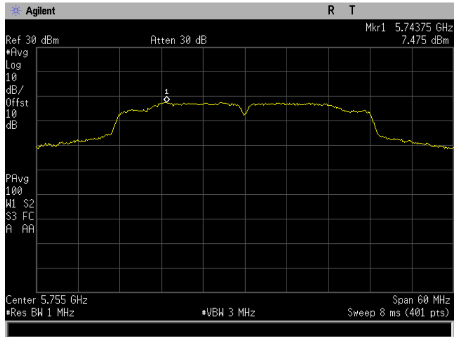
Plot 89. Power Spectral Density, SISO, Bandwidth 40M, Ch. 5755M, ac mode, port a
