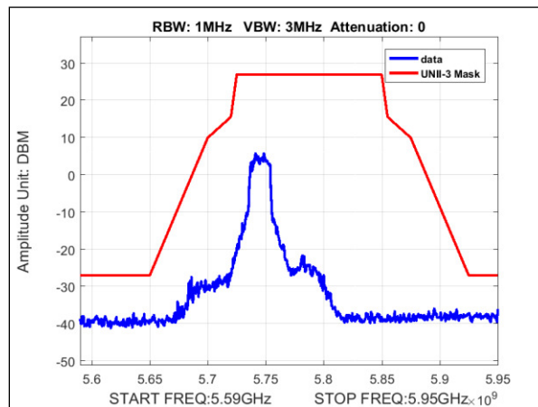
Plot 135. Undesirable Emissions, MIMO, Emissions Mask, Bandwidth 20M, Ch. 5745, n mode
