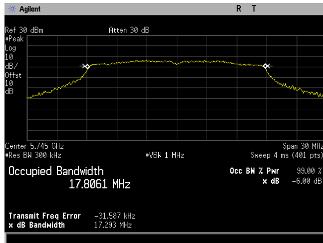
Plot 2. Occupied Bandwidth, 6dB, Bandwidth 20M, Ch. 5745M, ac mode
