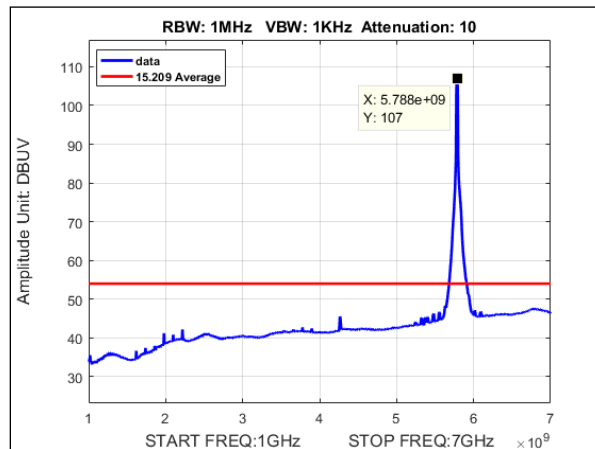
Plot 150. Undesirable Emissions, Average Radiated Spurious Emissions, MIMO, Bandwidth 20MHz, Ch. 5785, n mode, 1-7GHz
