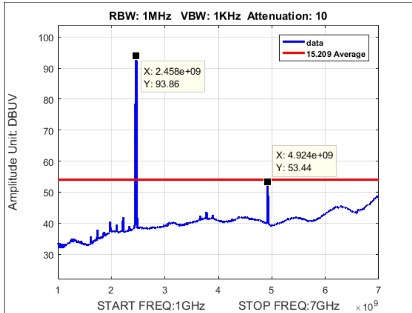
Plot 111. Radiated Emissions, SISO, Average Radiated Spurious Emissions, 20M, High Channel, b mode, 2462 at 13.25 dBm, 17-GHz
