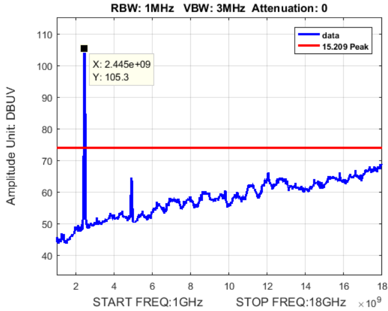
Plot 147. Peak Radiated Spurious Emissions, MIMO, HT8, 40M, High Channel, 2452, 1-18 GHz
