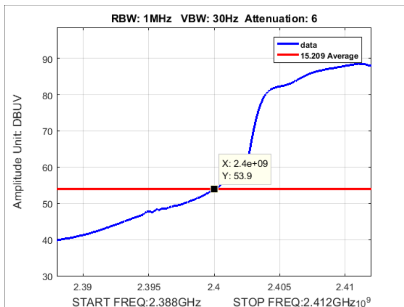
Plot 169. Average Radiated Band Edge, SISO, g mode, port b, Low Channel, 2412M at 17.25 dBm
