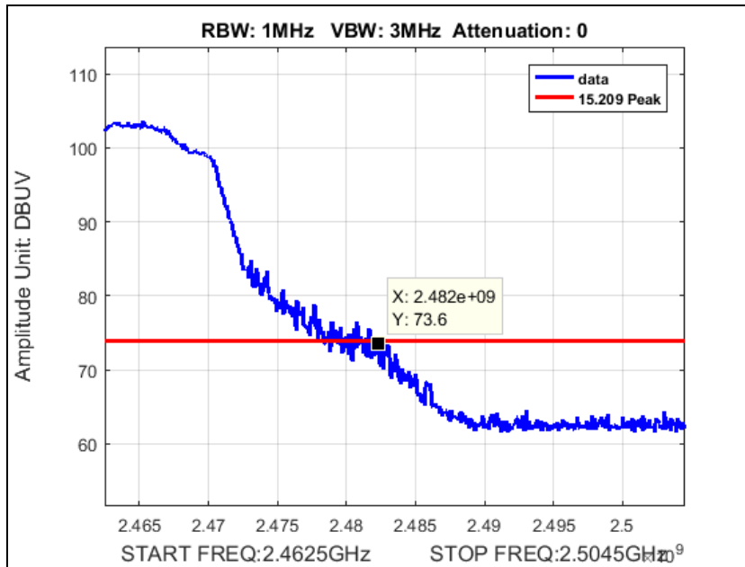
Plot 178. Peak Radiated Band Edge, SISO, N20, port b, High Channel, 2462M at 19.25 dBm
