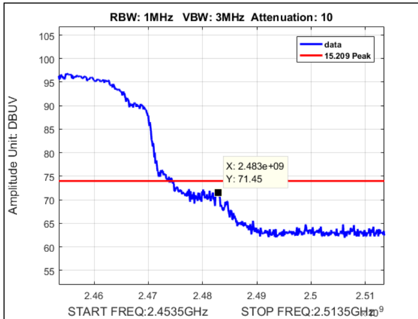
Plot 180. Peak Radiated Band Edge, SISO, N40, port b, High Channel, 2452M at 19 dBm
