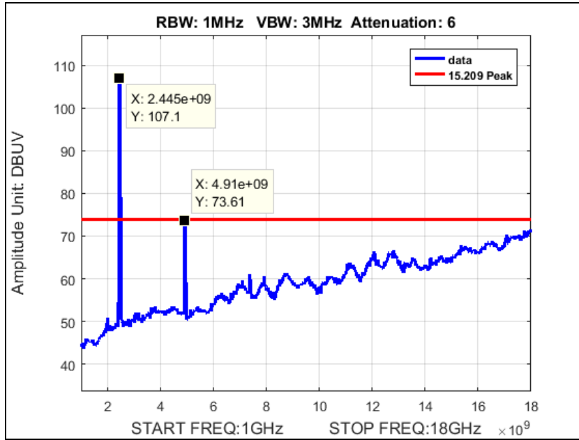
Plot 123. Peak Radiated Spurious Emissions, 20M, b mode, High Channel, 2462 at 22 dBm, 1-18 GHz
