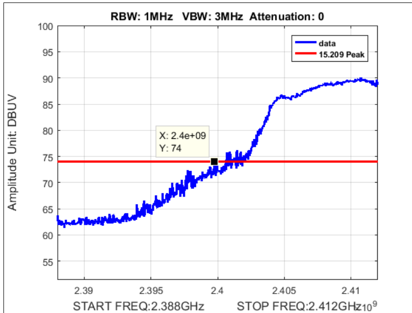
Plot 161. Peak Radiated Band Edge, SISO, g mode, port a, Low Channel, 2412M at 18 dBm
