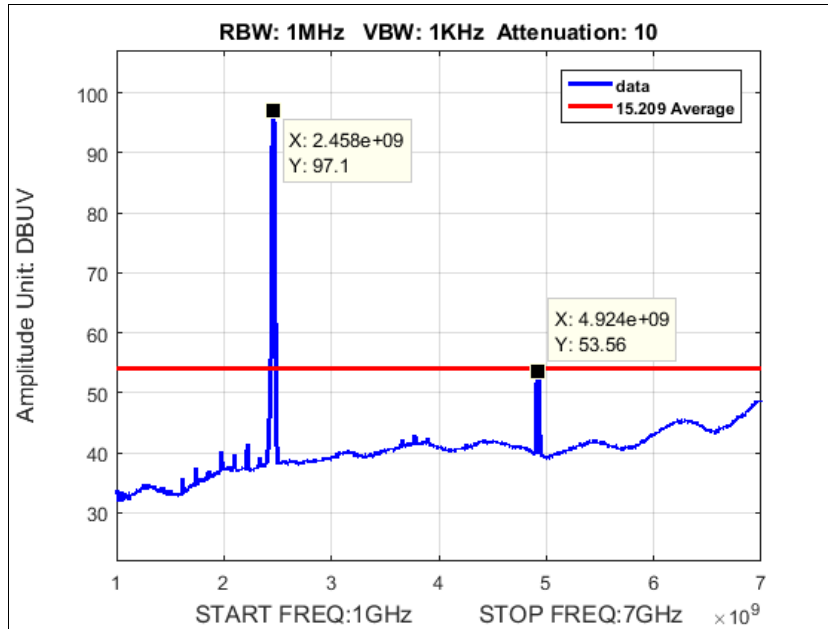
Plot 135. Average Radiated Spurious Emissions, MIMO, HT8, 20M, High Channel, 2462 at 17 dBm, 1-7 GHz
