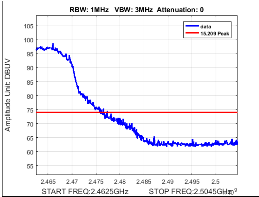
Plot 160. Peak Radiated Band Edge, SISO, g mode, port a, High Channel, 2462M at 24 dBm
