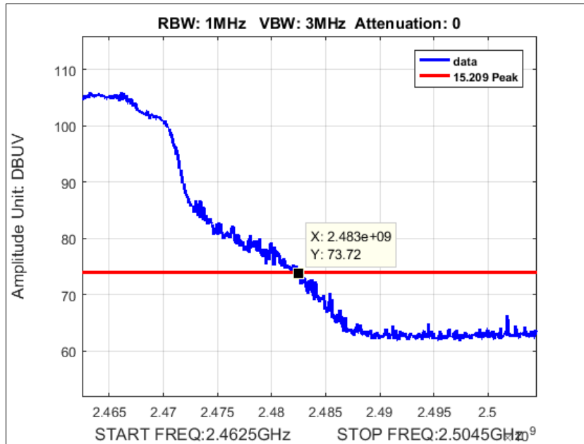
Plot 186. Peak Radiated Band Edge, MIMO, HT8, 20M, High Channel, 2462M at 19 dBm
