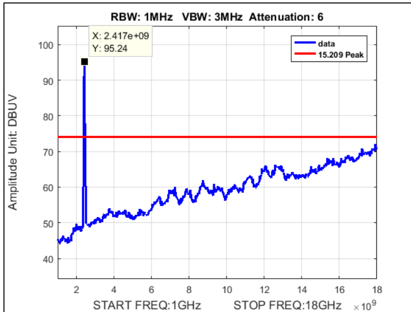
Plot 130. Peak Radiated Spurious Emissions, N20, 20M, Low Channel, 2412, 1-18 GHz
