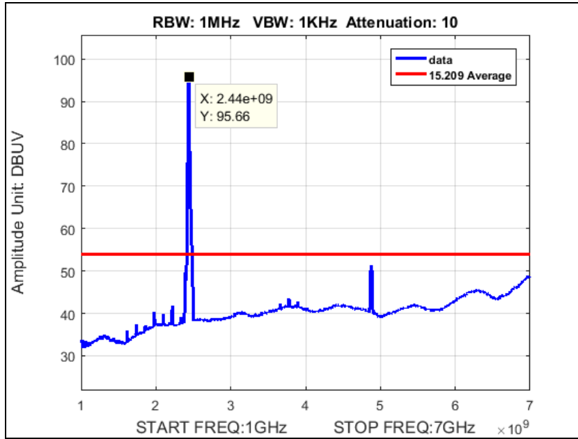
Plot 119. Average Radiated Spurious Emissions, N20, 20M, Mid Channel, 2437, 1-7 GHz
