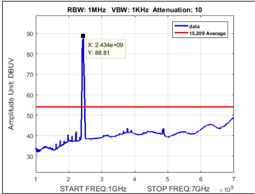
Plot 121. Average Radiated Spurious Emissions, N40, 40M, Low Channel, 2422, 1-7 GHz
