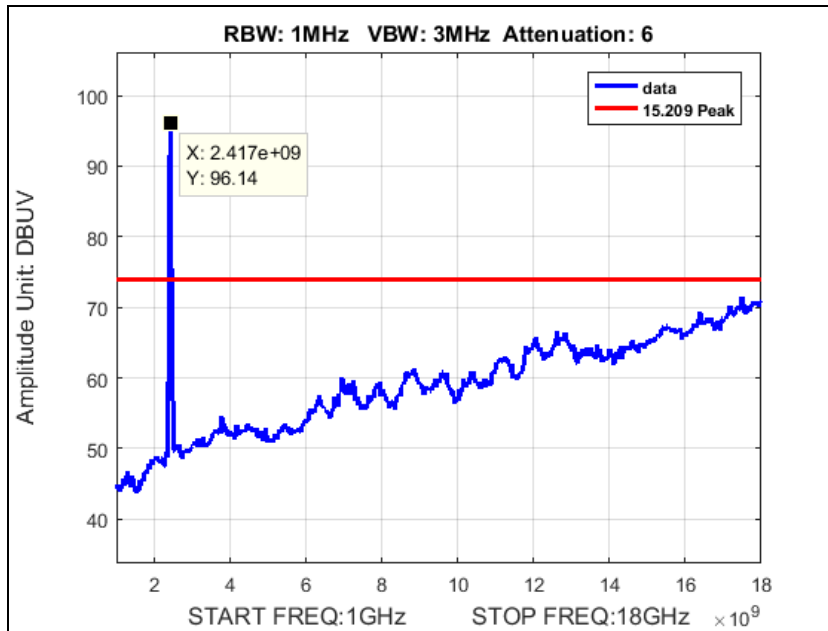
Plot 127. Peak Radiated Spurious Emissions, 20M, g mode, Low Channel, 2412, 1-18 GHz
