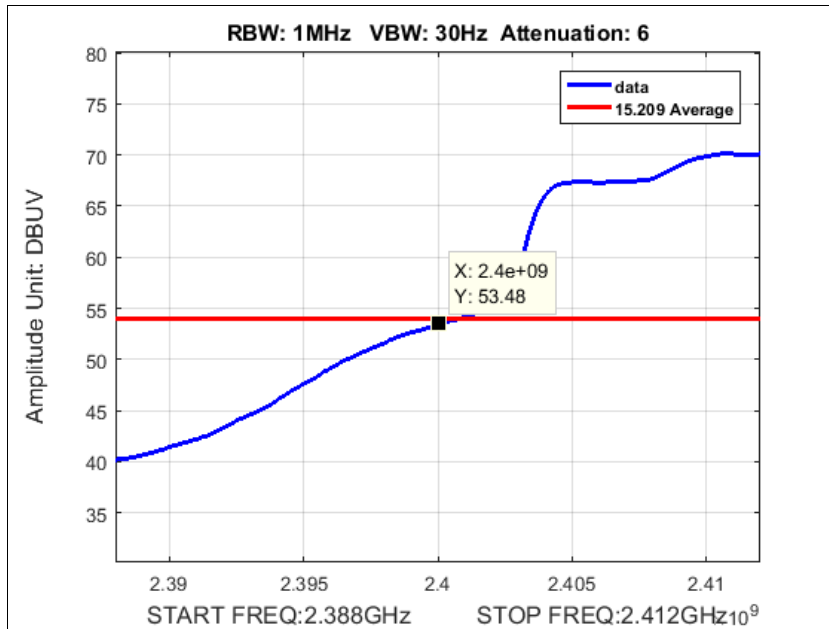
Plot 157. Average Radiated Band Edge, SISO, N40, port a, Low Channel, 2422M at 18.25 dBm
