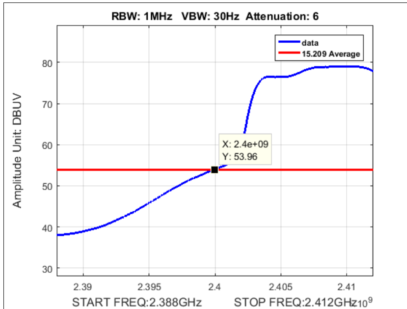
Plot 155. Average Radiated Band Edge, SISO, N20, port a, Low Channel, 2412M at 17 dBm
