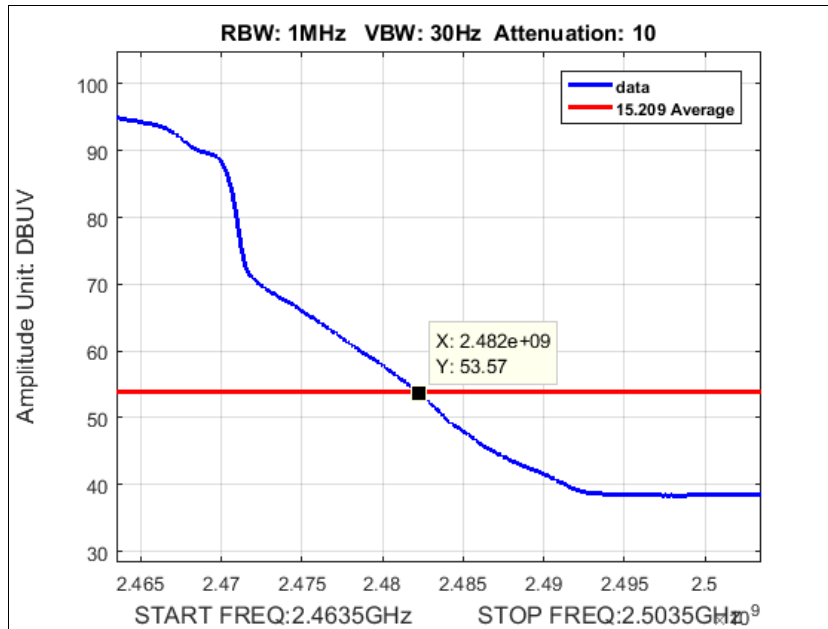
Plot 168. Average Radiated Band Edge, SISO, g mode, port b, High Channel, 2462M at 19 dBm
