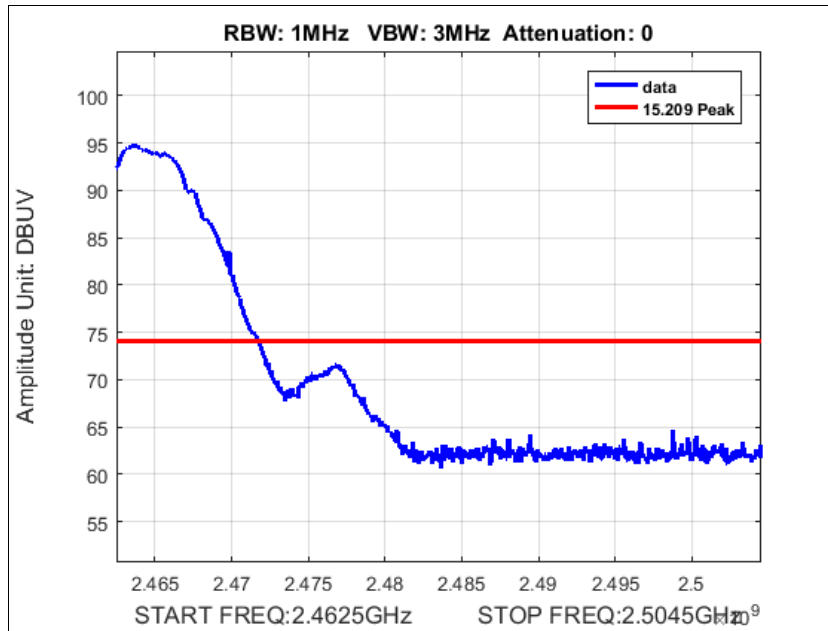
Plot 158. Peak Radiated Band Edge, SISO, b mode, port a, High Channel, 2462M at 24 dBm
