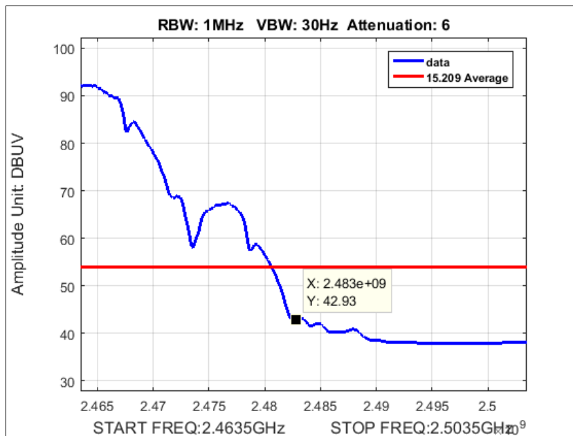
Plot 150. Average Radiated Spurious Band Edge, SISO, b mode, port a, High Channel, 2462M at 24 dBm
