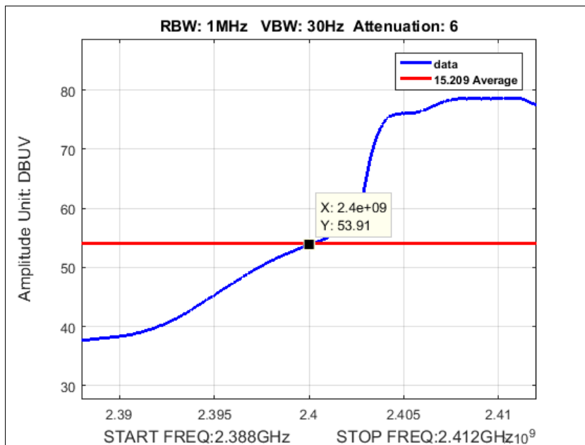
Plot 153. Average Radiated Band Edge, SISO, g mode, port a, Low Channel, 2412M at 17 dBm
