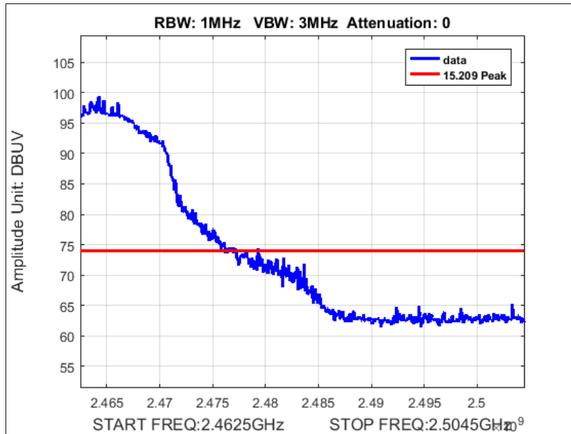
Plot 162. Peak Radiated Band Edge, SISO, N20, port a, High Channel, 2462M at 24 dBm
