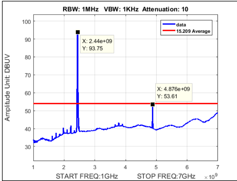
Plot 113. Radiated Emissions, Average Radiated Spurious Emissions, SISO, 20M, Mid Channel, 2437 at 17.25 dBm, 1-7 GHz
