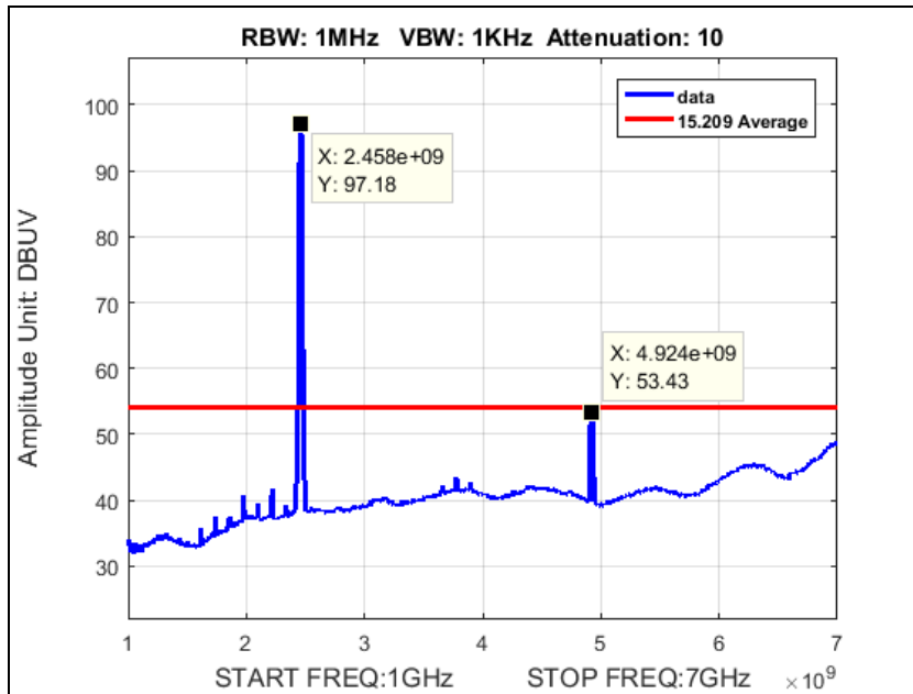
Plot 117. Radiated Emissions, Average Radiated Spurious Emissions, N20, 20M, High Channel, 2462 at 19 dBm 1-7 GHz
