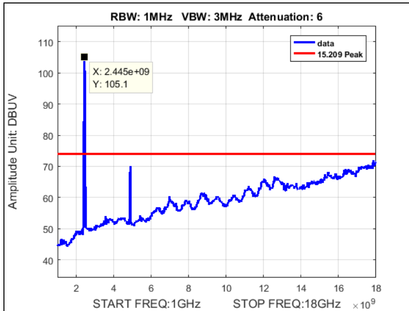
Plot 125. Peak Radiated Spurious Emissions, 20M, b mode, Mid Channel, 2437, 1-18 GHz
