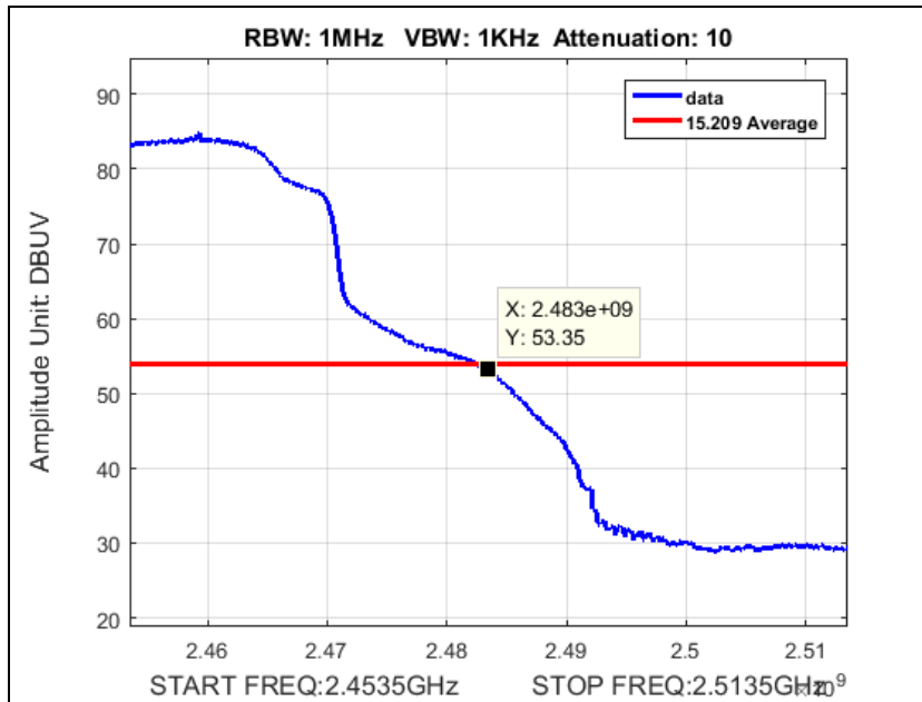
Plot 184. Average Radiated Band Edge, MIMO, HT8, 40M, High Channel, 2452M at 19 dBm
