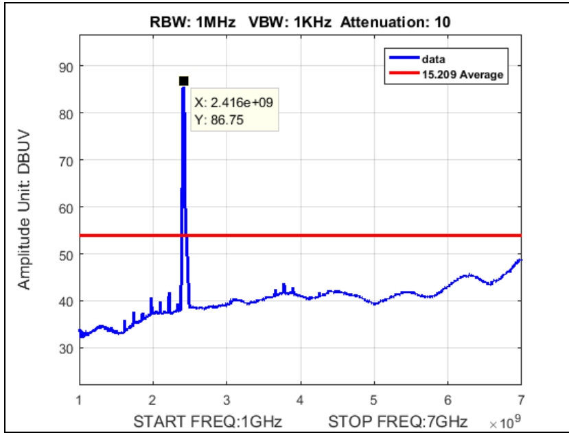
Plot 115. Radiated Emissions, Average Radiated Spurious Emissions, 20M, g mode, Low Channel, 2412, 1-7 GHz
