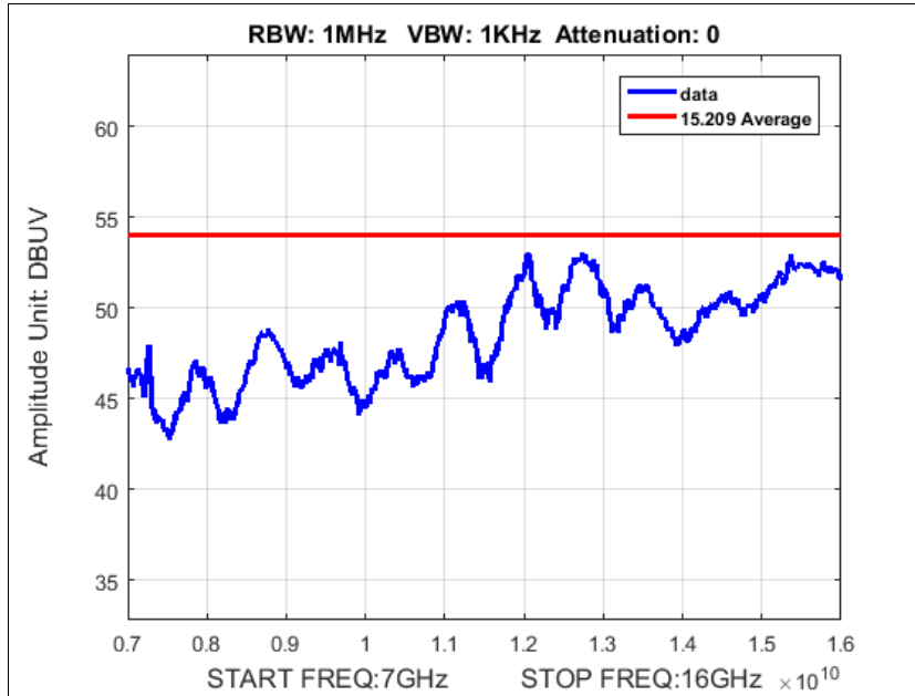
Plot 141. Average Radiated Spurious Emissions, MIMO, HT8, 40M, Low Channel, 2422, 7-16 GHz
