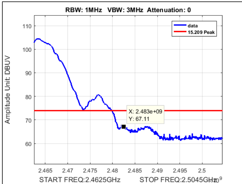
Plot 174. Peak Radiated Band Edge, SISO, b mode, port b, High Channel, 2462 at 24 dBm
