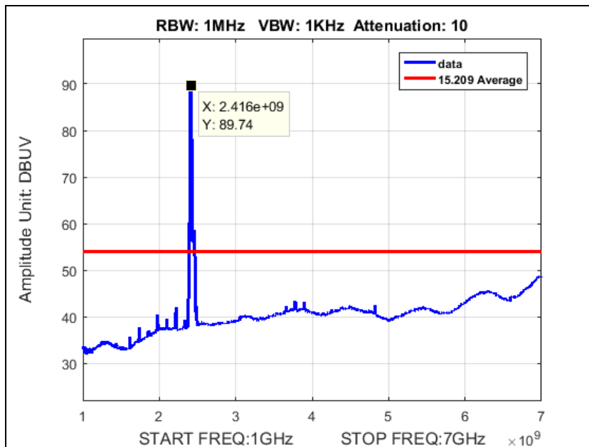
Plot 112. Radiated Emissions, SISO, Average Radiated Spurious Emissions, 20M, low channel, b mode, 2412, 1-7GHz
