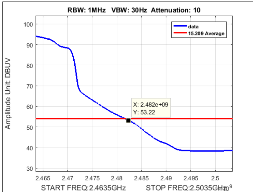
Plot 170. Average Radiated Band Edge, SISO, N20, port b, High Channel, 2462M at 18.25 dBm
