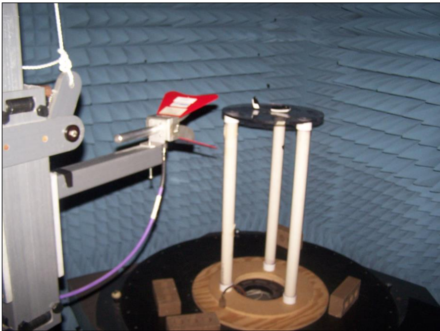
Radiated Spurious Emissions, Test Setup, Above 1 GHz
