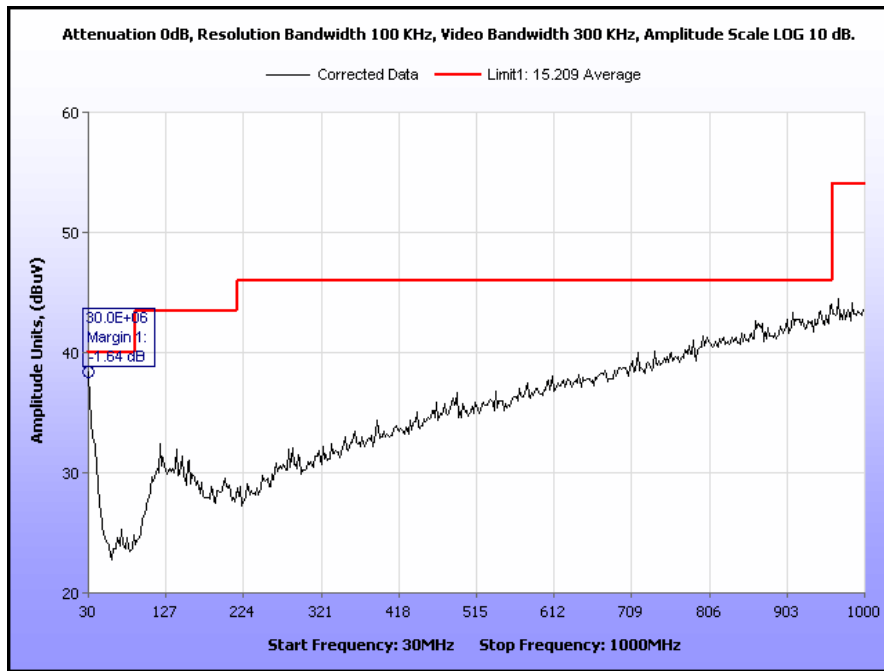
Plot 16. Radiated Spurious Emissions, Low Channel, 30 MHz – 1 GHz
