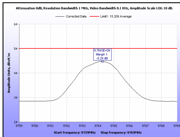
Plot 20. Radiated Spurious Emissions, Mid Channel, 1 GHz – 18 GHz, 9.764 GHz
