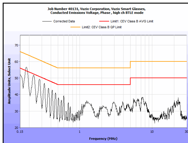
Plot 3. Conducted Emissions, 15.207(a), Phase Line, High Channel
