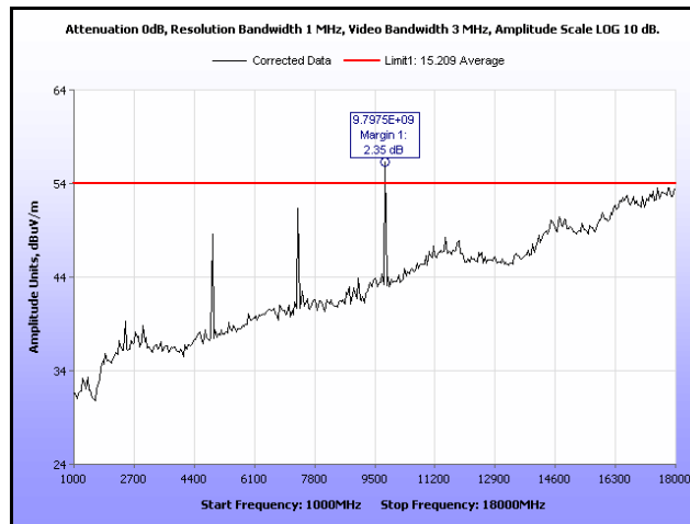
Plot 19. Radiated Spurious Emissions, Mid Channel, 1 GHz – 18 GHz
