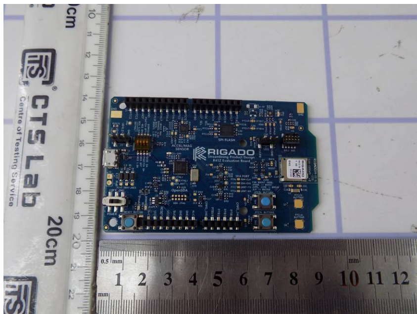
Jig view 1
