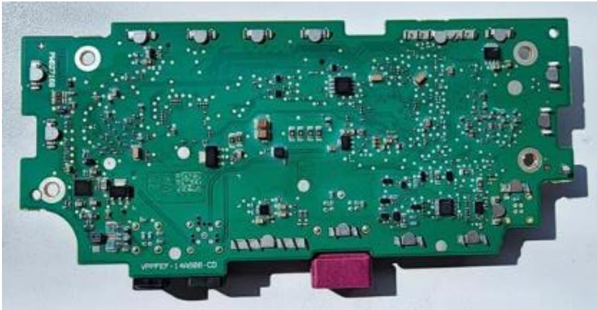
MEZ – Bottom view
