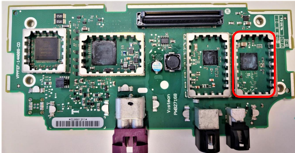
MEZ - Top View with RF Shield
