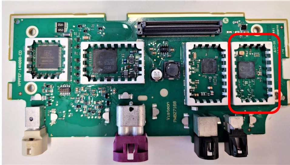
MEZ - Top View with RF Shield
