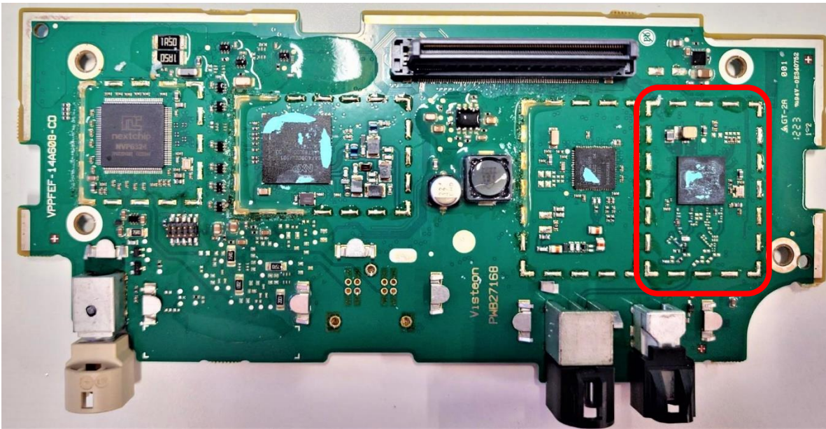
MEZ - Top View without RF Shield
