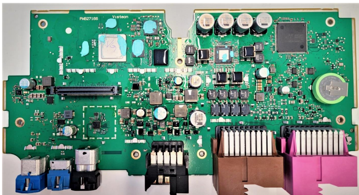
PWBA – Top View without RF Shield
