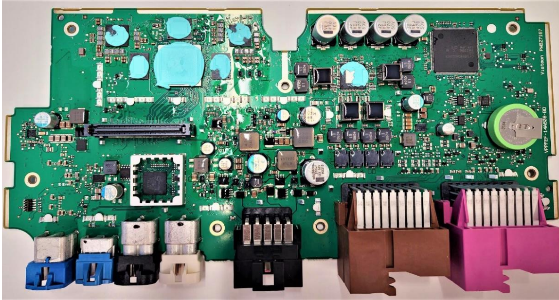
PWBA – Top View without RF Shield
