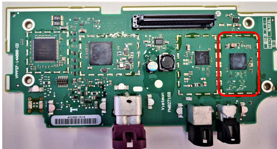
MEZ - Top View without RF shield
