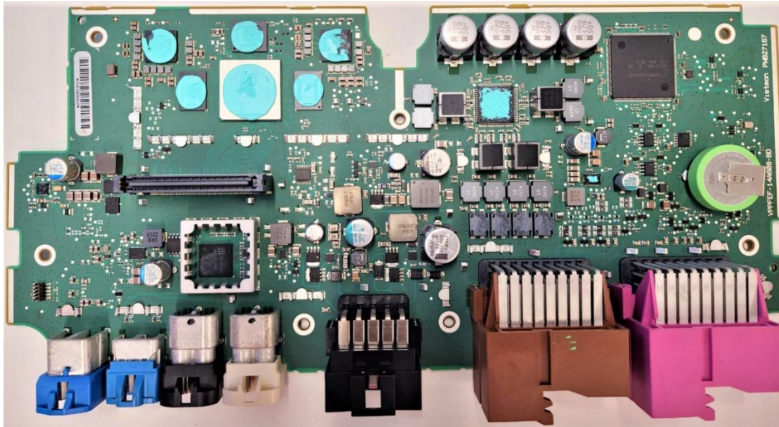
PWBA – Top View with RF Shield
