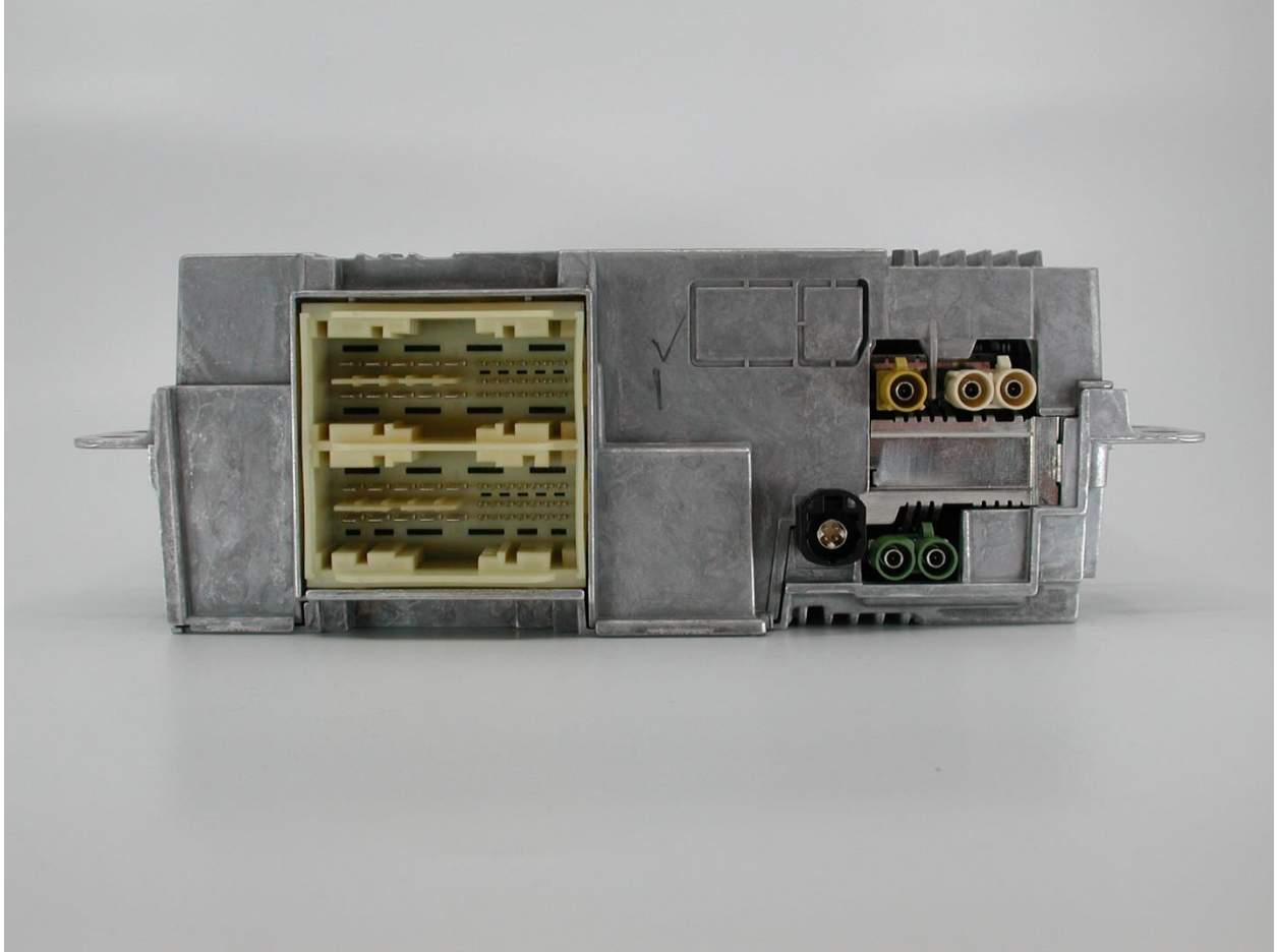
2. Front Elevation of MFA2 Housing
