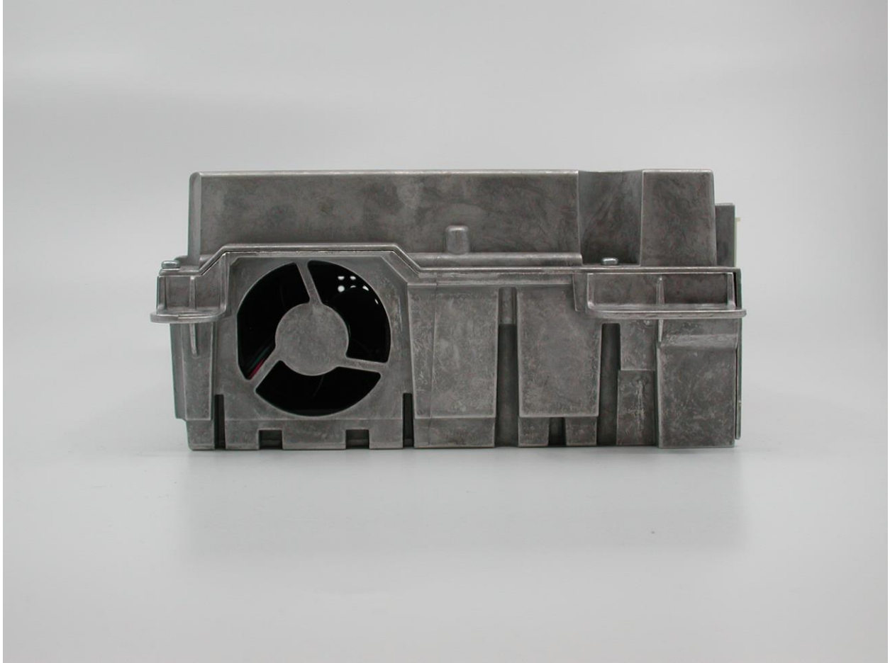
4. Left Elevation of MFA2 Housing
