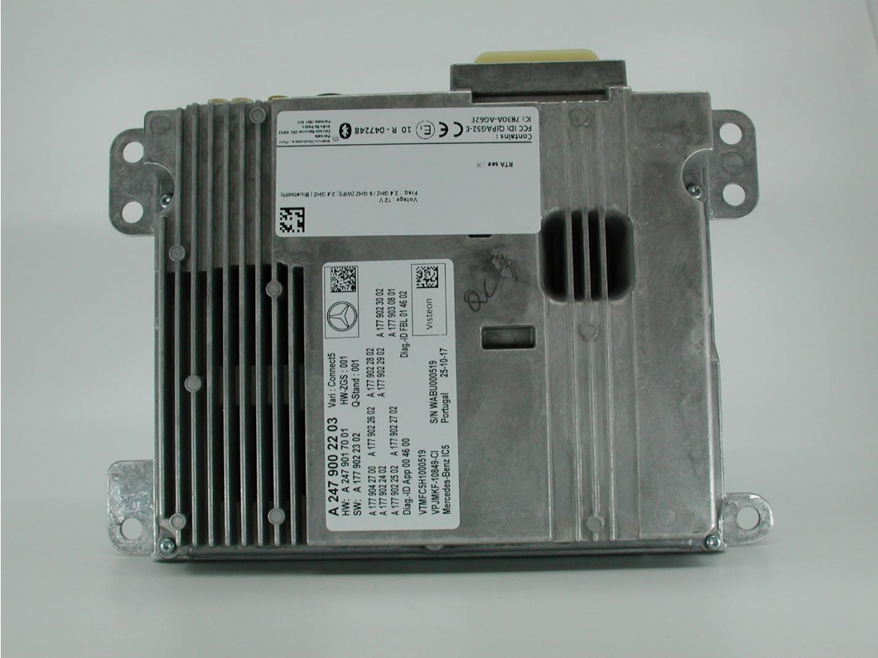
1. Top Elevation of MFA2 Housing
