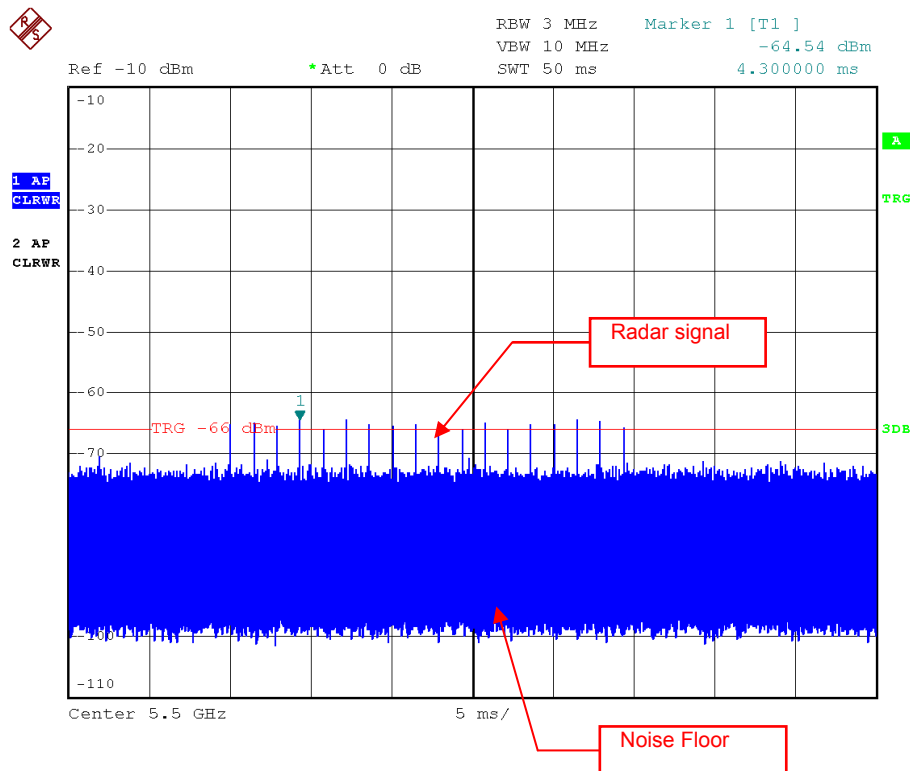
Radar Signal 1
