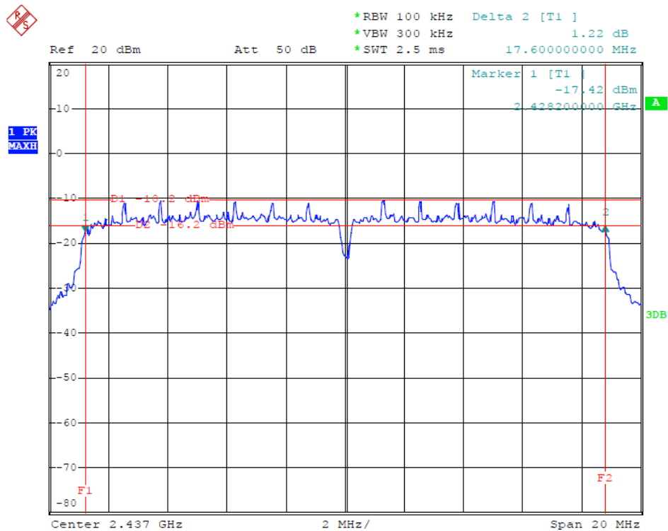
802.11n Channel Middle 2437MHz(20MHz)
