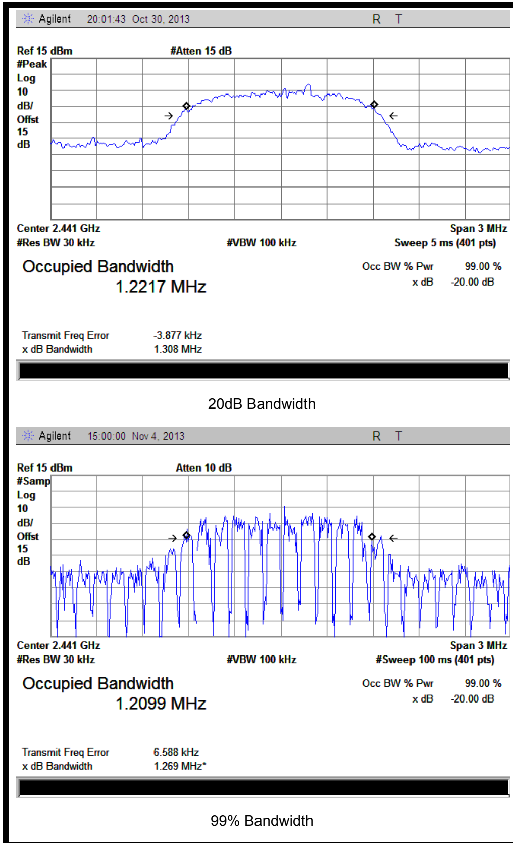
(Plot H: Channel = 2441 @ 8-DPSK)
