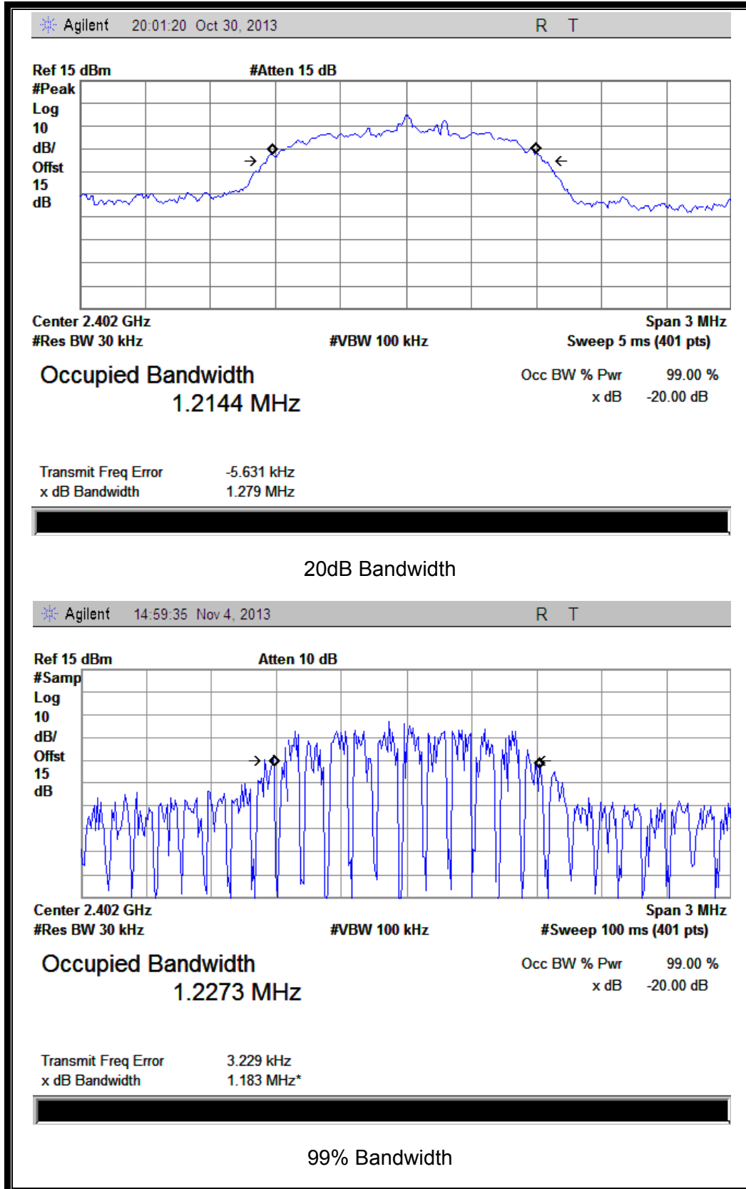
(Plot G: Channel = 2402 @ 8-DPSK)
