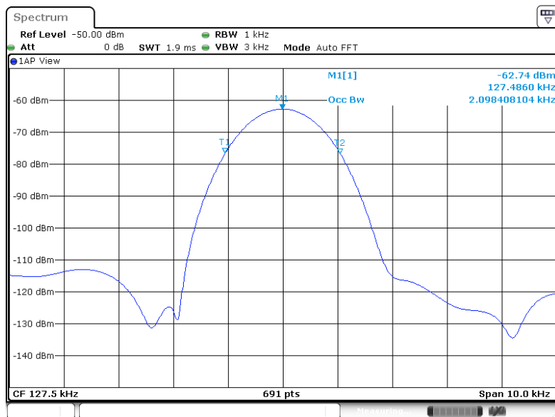
Emission Bandwidth Plot 99% Bandwidth (127.5 kHz)
