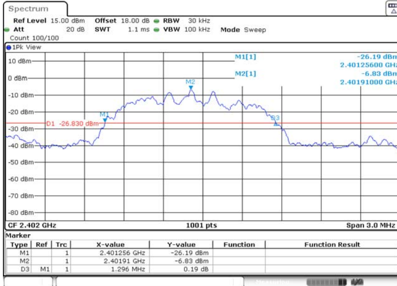
3DH5 Ant1_2402
