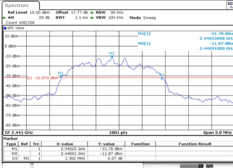
3DH5 Ant1_2441
