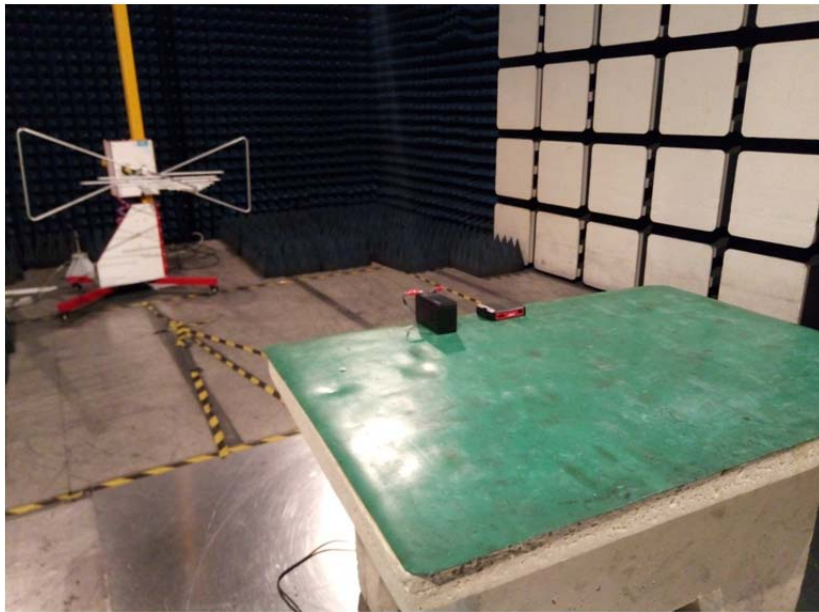
Test setup
