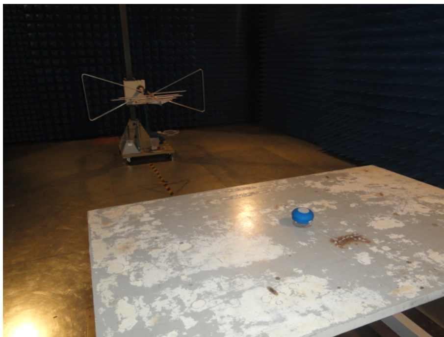
Emission Radiated test View
