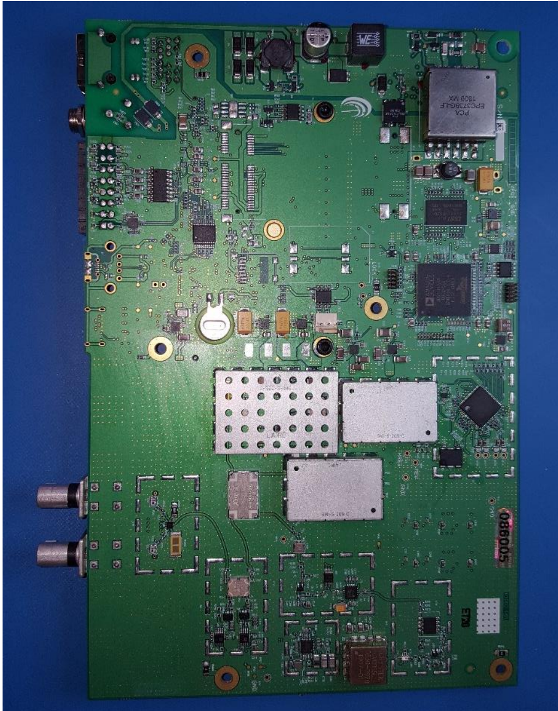
Figure 1: Top Side, Shield Can Lids Installed
