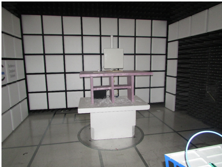
Figure 4: Radiated Emissions – Front – Above 1GHz
