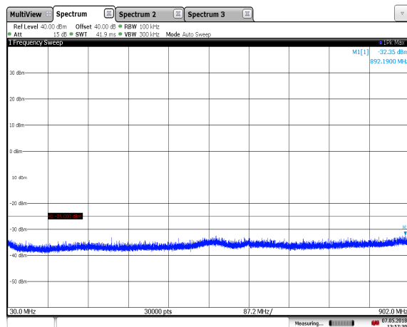
13:57:30 07.05.2018 Figure 7.3.2-21: 902.75 MHz – ISO-10374 - 30MHz to Edge
