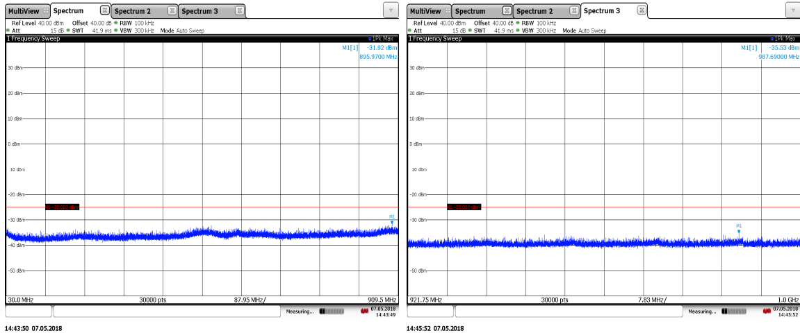
Figure 7.3.2-35: 916.25 MHz – PS111 - 30MHz to Edge
