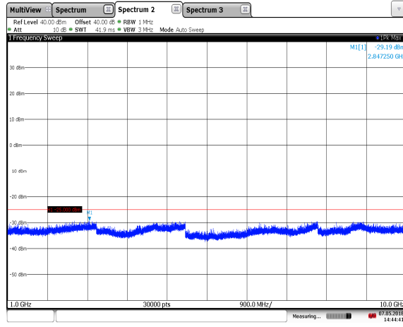
Figure 7.3.2-37: 916.25 MHz – PS111 - 1 GHz – 10GHz
