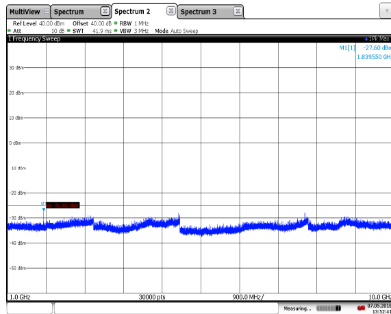
Figure 7.3.2-8: 919.25 MHz – C1G2 - 1 GHz – 10GHz
