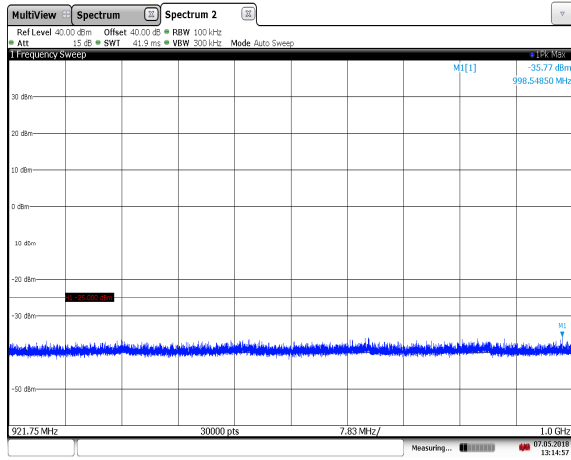
Figure 7.3.2-12: 911.75 MHz – ISOB – Edge to 1GHz
