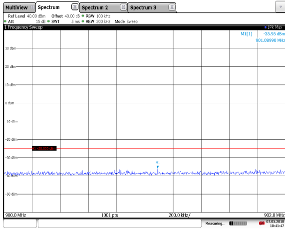
10:41:47 07.05.2018 Figure 7.3.2-17: 902.75 MHz – ISO10374 - Low Edge
