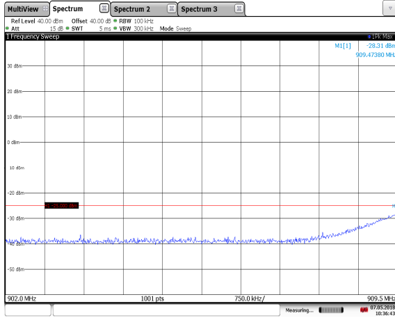
Figure 7.3.2-9: 911.75 MHz – ISOB - Low Edge
