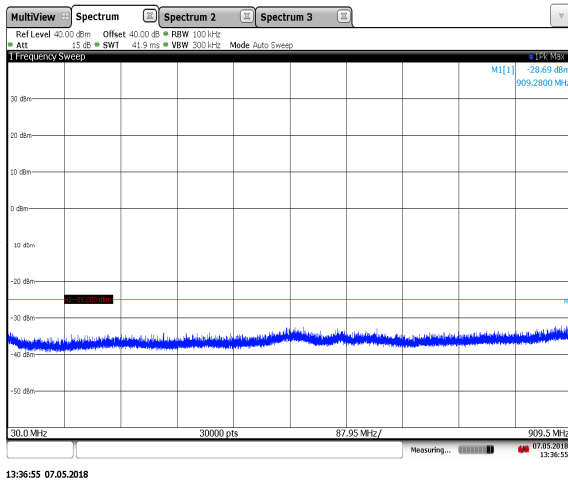
Figure 7.3.2-3: 911.75 MHz – C1G2 - 30MHz to Edge
