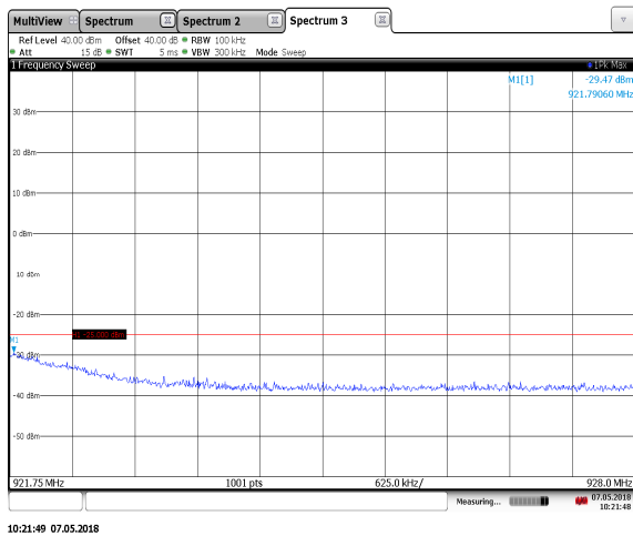
Figure 7.3.2-2: 919.25 MHz – C1G2 – High Edge
