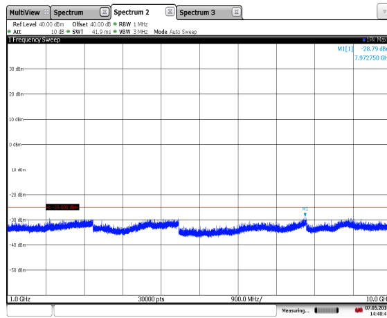
Figure 7.3.2-34: 913.75 MHz – PS111 - 1 GHz – 10GHz
