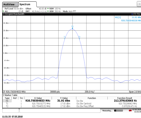
Figure 7.2.2-7: 920.75 MHz – IS0-10374
