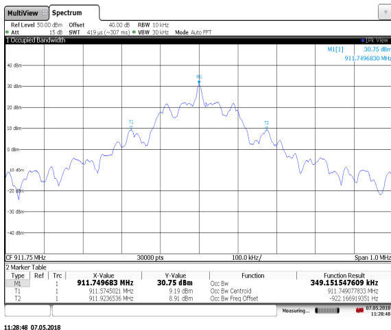
Figure 7.2.2-1: 911.75 MHz – C1G2
