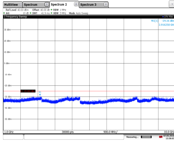
Figure 7.3.2-23: 902.75 MHz – ISO-10374 - 1 GHz – 10GHz
