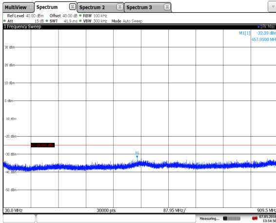
Figure 7.3.2-6: 919.25 MHz – C1G2 - 30MHz to Edge
