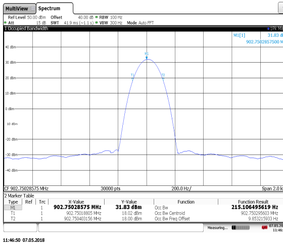
Figure 7.2.2-5: 902.75 MHz – IS0-10374
