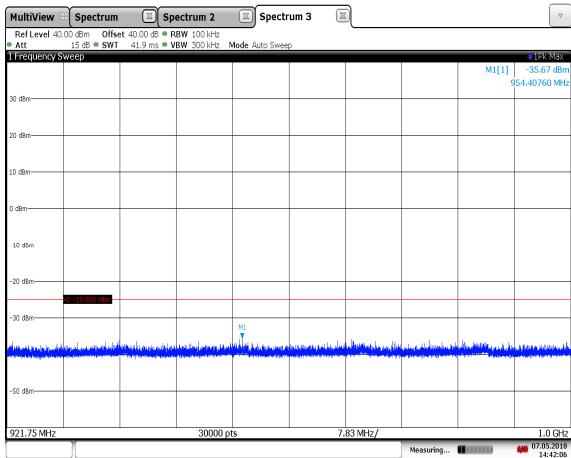
Figure 7.3.2-33: 913.75 MHz – PS111 – Edge to 1GHz
