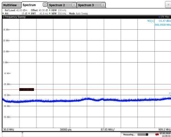
Figure 7.3.2-32: 913.75 MHz – PS111 - 30MHz to Edge
