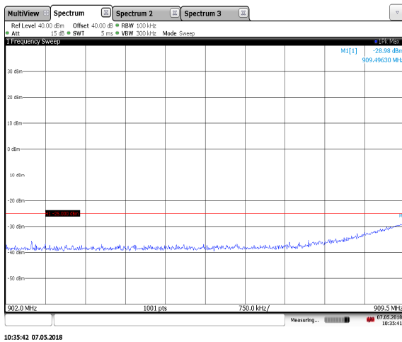
Figure 7.3.2-1: 911.75 MHz – C1G2 - Low Edge
