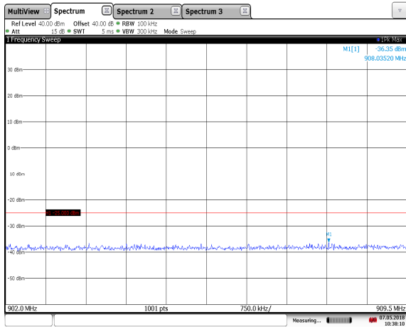
10:38:10 07.05.2018 Figure 7.3.2-19: 910.75 MHz – ISO10374 - Low Edge
