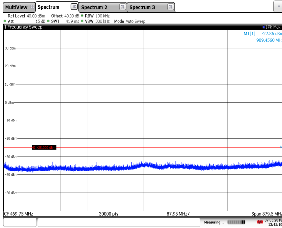
Figure 7.3.2-11: 911.75 MHz – ISOB - 30MHz to Edge
