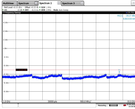
Figure 7.3.2-29: 920.75 MHz – ISO-10374 - 1 GHz – 10GHz
