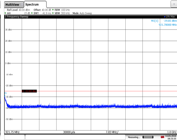
Figure 7.3.2-7: 919.25 MHz – C1G2 – Edge to 1GHz
