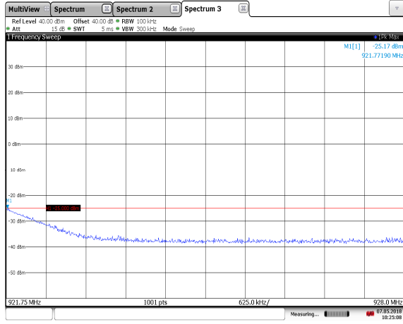
Figure 7.3.2-10: 919.75 MHz – ISOB – High Edge
