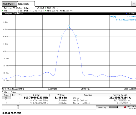
Figure 7.2.2-6: 910.75 MHz – IS0-10374
