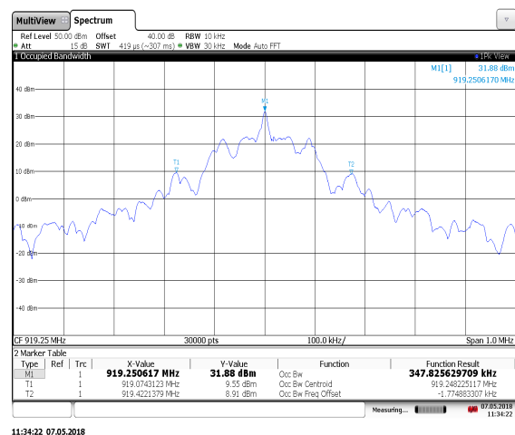
Figure 7.2.2-2: 919.25 MHz – C1G2
