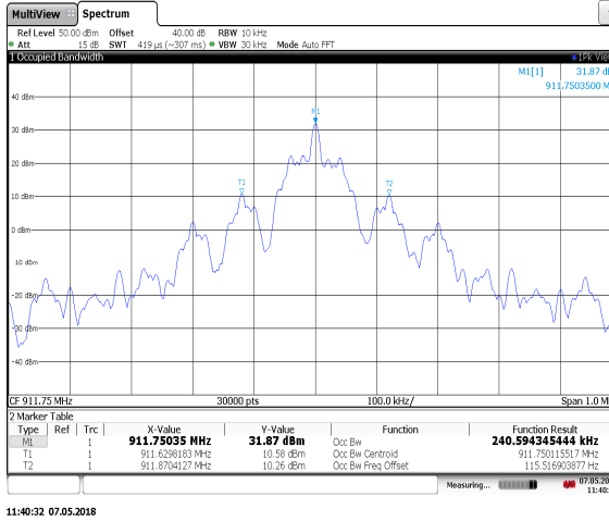
Figure 7.2.2-3: 911.75 MHz – IS0B
