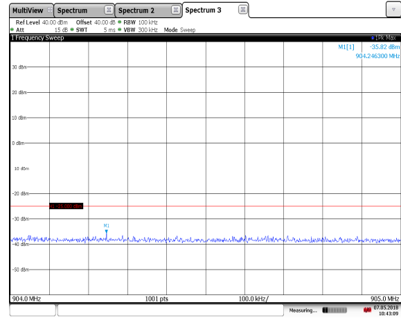
10:43:09 07.05.2018 Figure 7.3.2-18: 903.25 MHz – ISO10374 – High Edge
