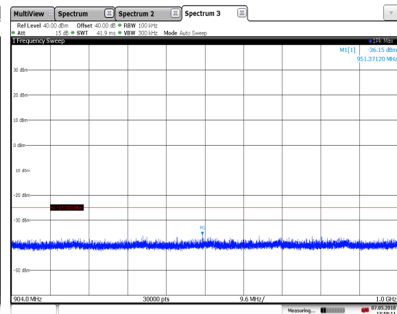
13:59:11 07.05.2018 Figure 7.3.2-22: 902.75 MHz – ISO-10374 – Edge to 1GHz
