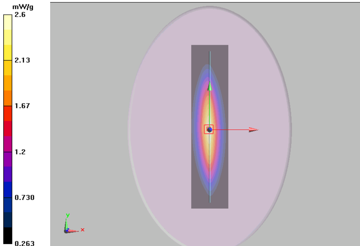
Figure 7 System Performance Check 835MHz 250mW
