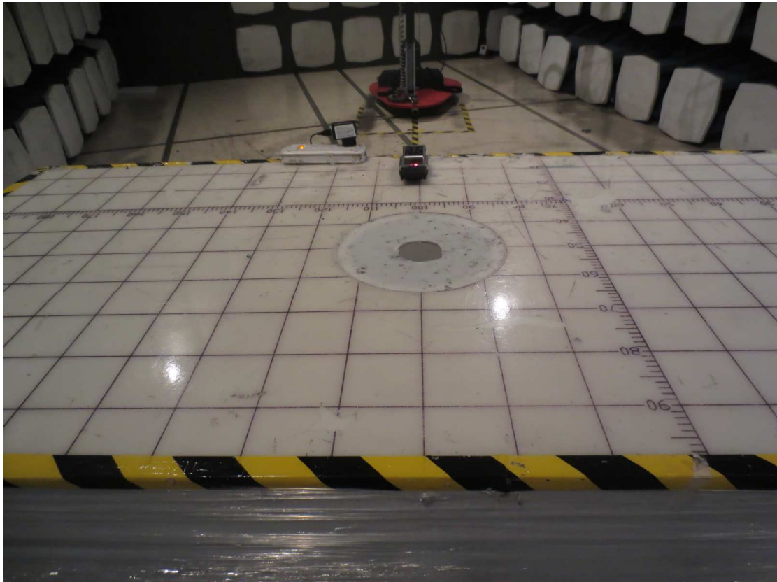
Test Setup Photo –Radiated Emission
