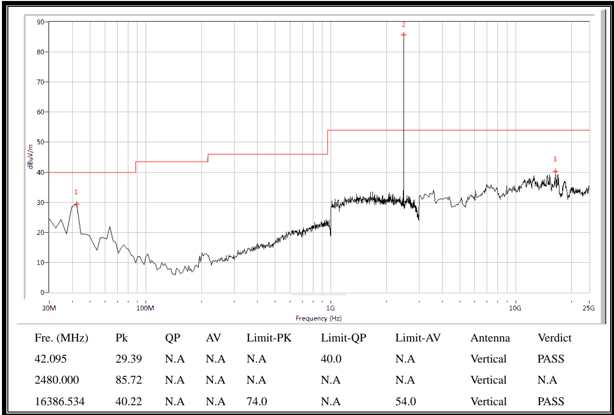
(Plot C.2: 30MHz to 25GHz, Antenna Vertical @ GFSK, channel 78)
