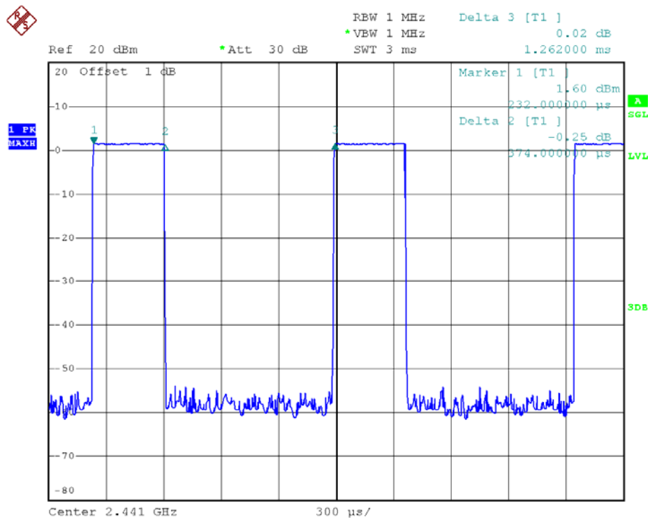
39 Channel @ DH1
