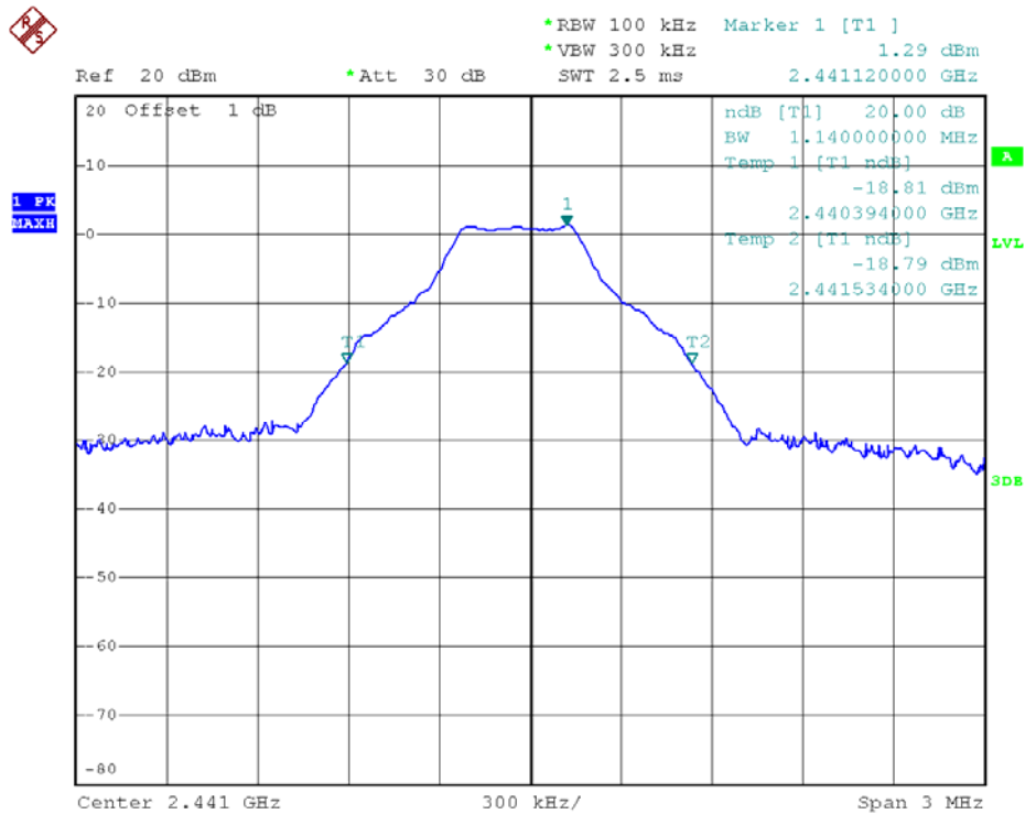
39 Channel @ GFSK
