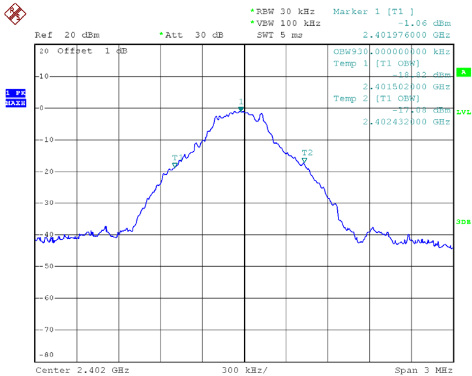
0 Channel @ GFSK
