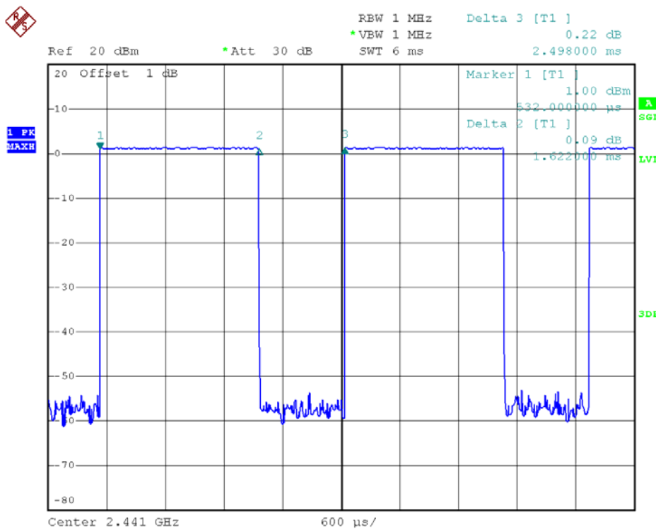
39 Channel @ DH3
