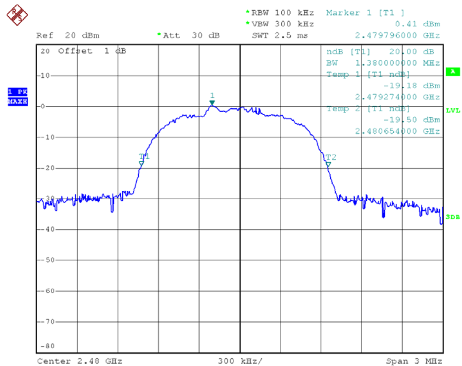
78 Channel @ 8-DPSK
