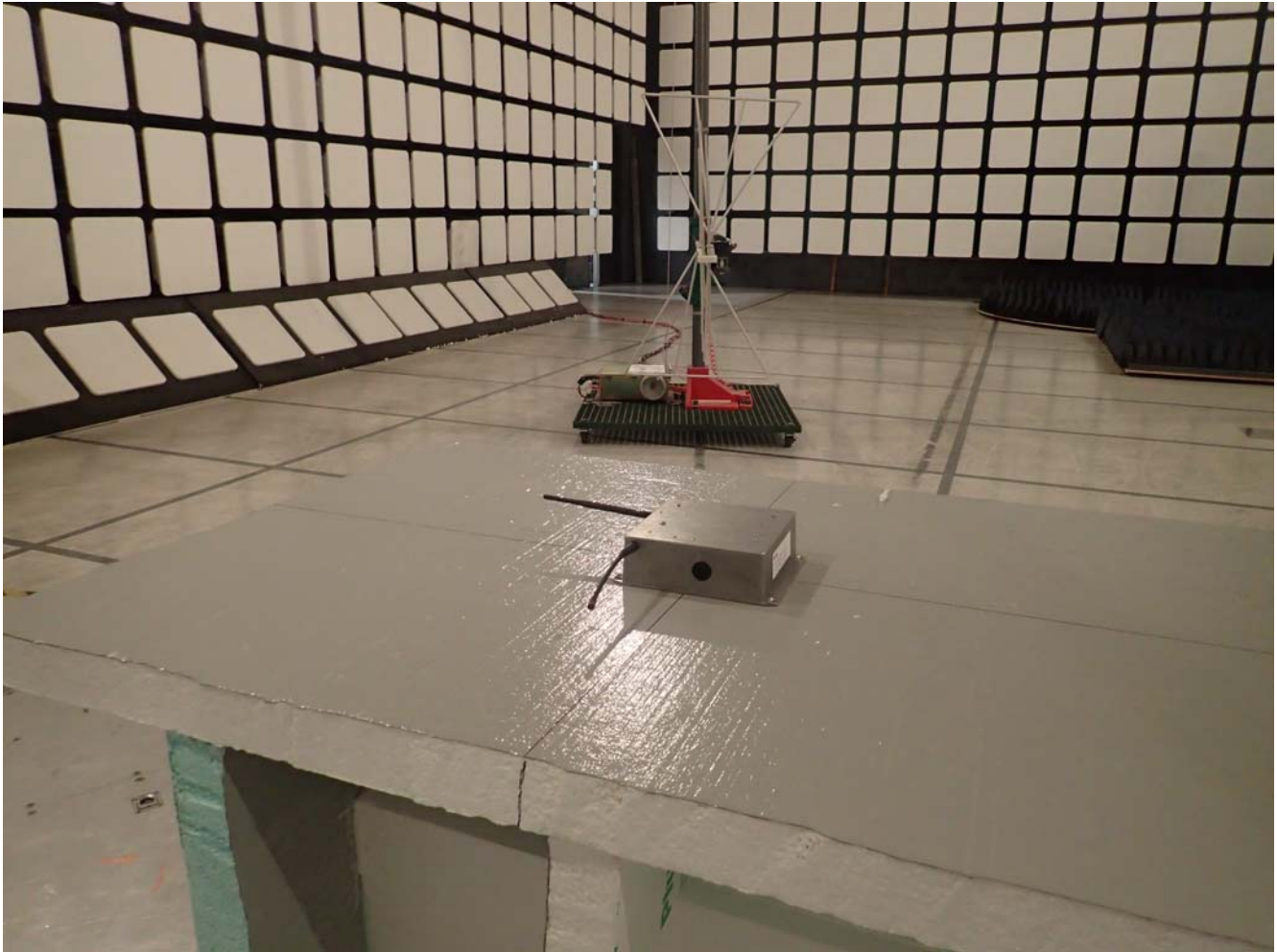
Radiated Emissions at 3m Distance EUT Orientation: Horizontal
