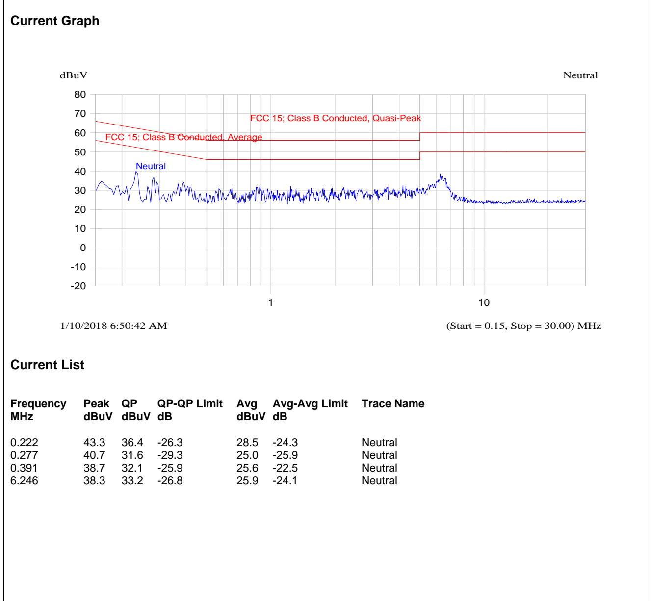
Plot 5.2.3.2. Power Line Conducted ions Line Voltage: AC 120 V; Line Tested: Neutral
