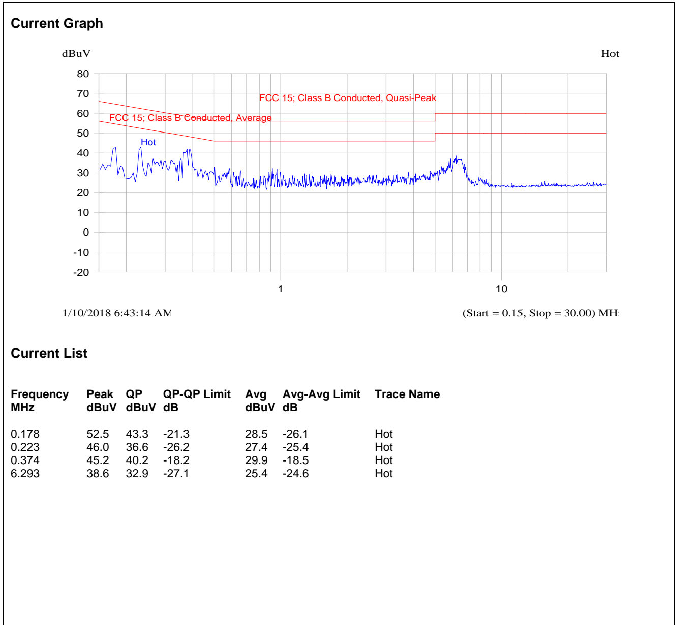
Plot 5.2.3.1. Power Line Conducted Emissions Line Voltage: AC 120 V; Line Tested: Hot
