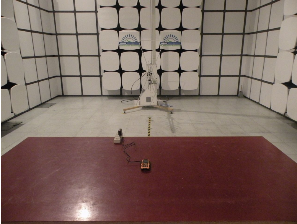
Photographs-Radiated Emission Test Setup in Chamber
