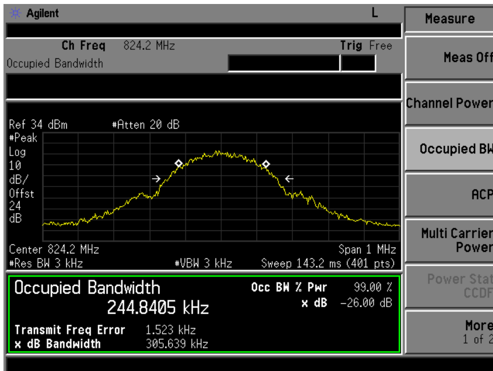
GSM 850 CH128
