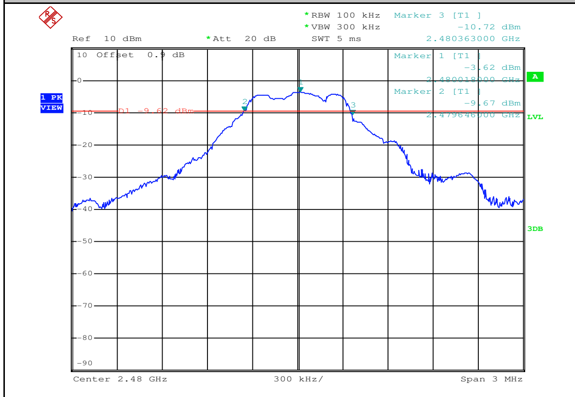
6dB Bandwidth_BLE_2480_Ant1
