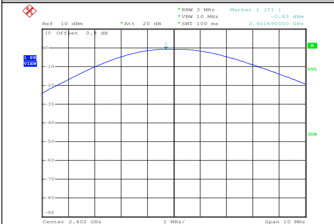
Maximum peak conducted output power_BLE_2402_Ant1
