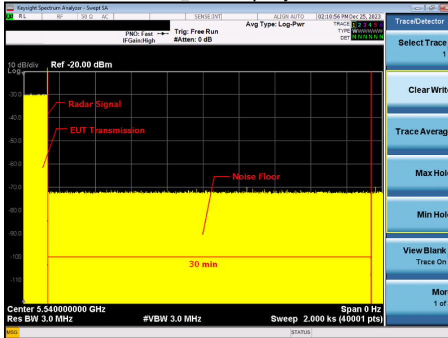
TX (IEEE 802.11a Mode) 5540MHz_Non-Occupancy Period
