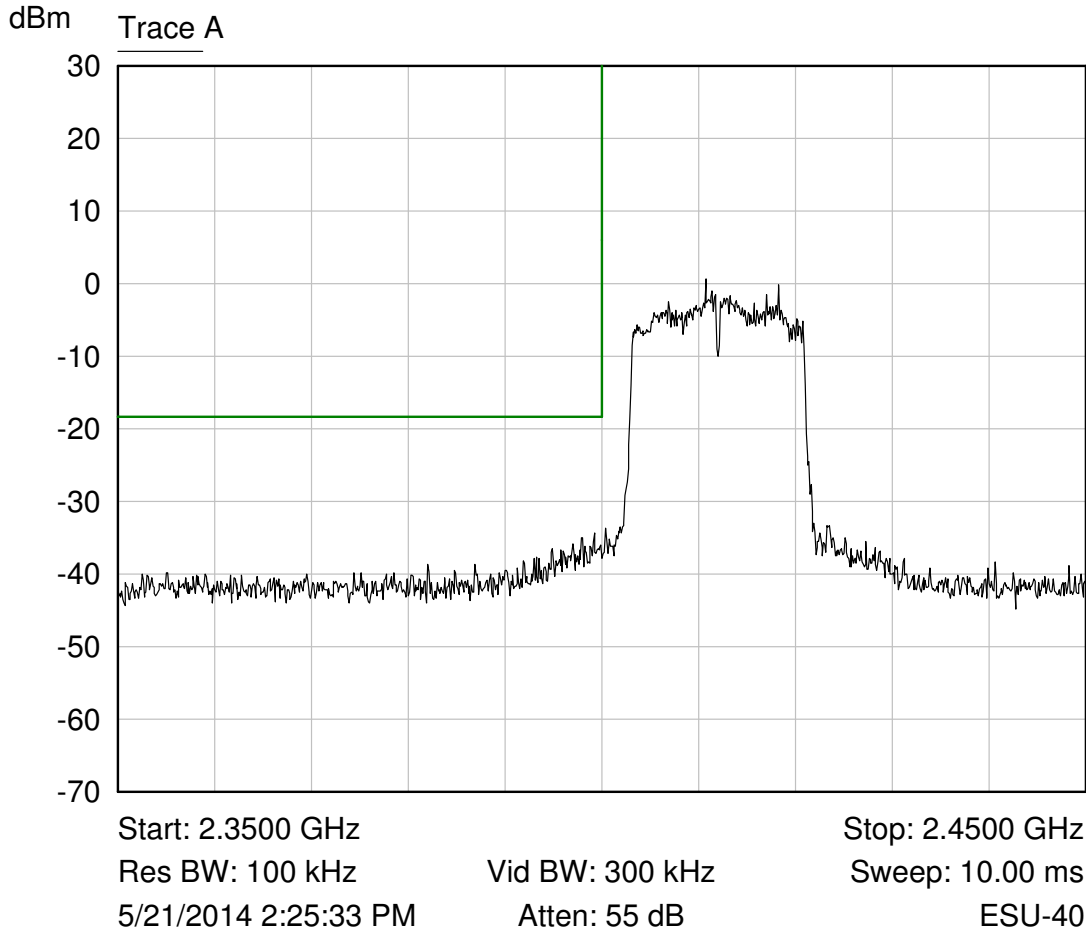
Trace A 802.11n +13 power setting
