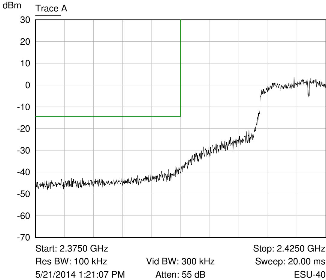
Trace A 802.11g +17 power setting
