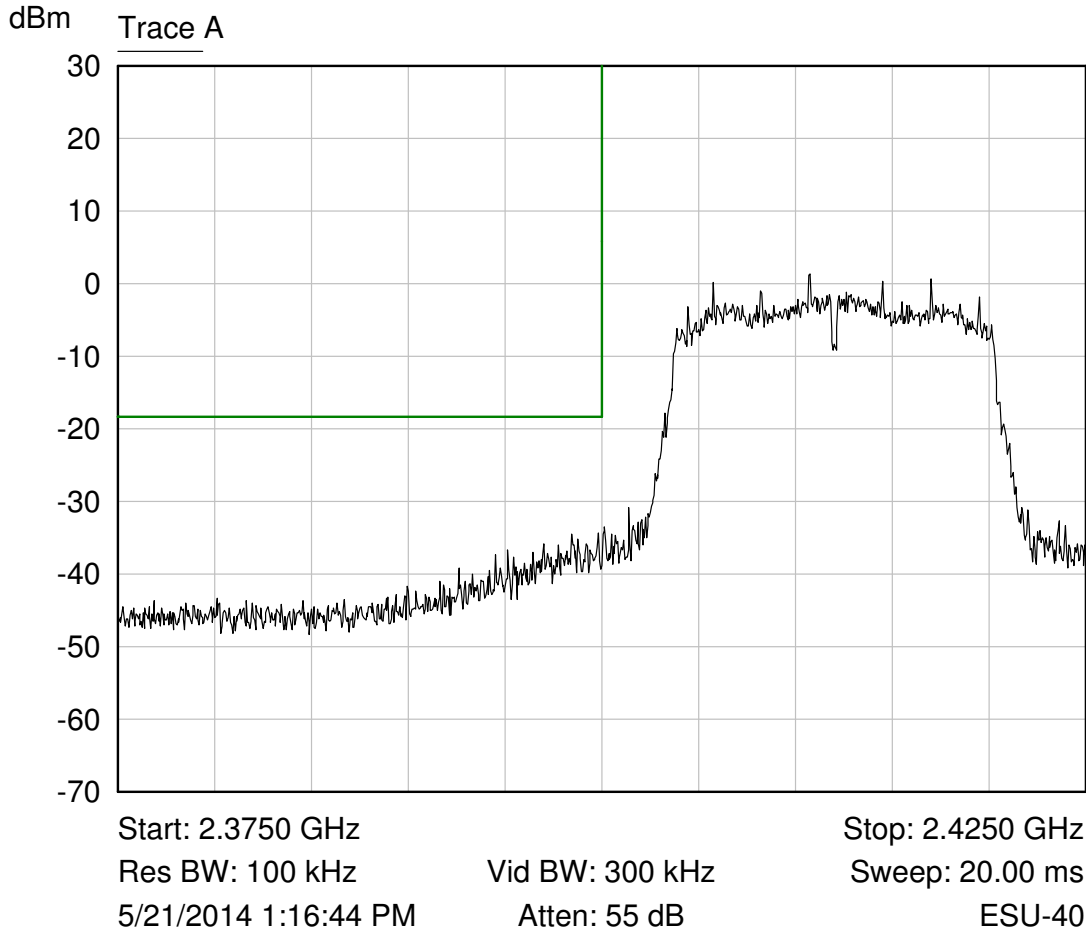
Trace A 802.11g +13 power setting
