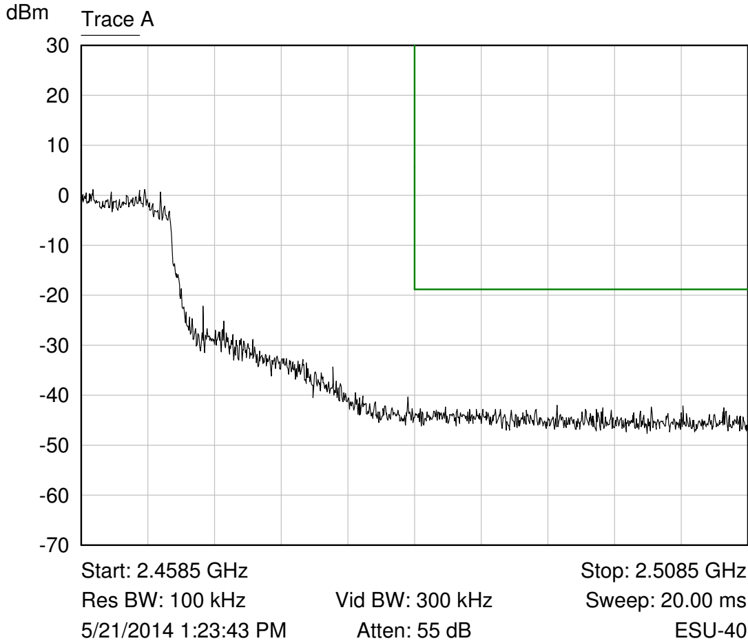
Trace A 802.11g +16 power setting
