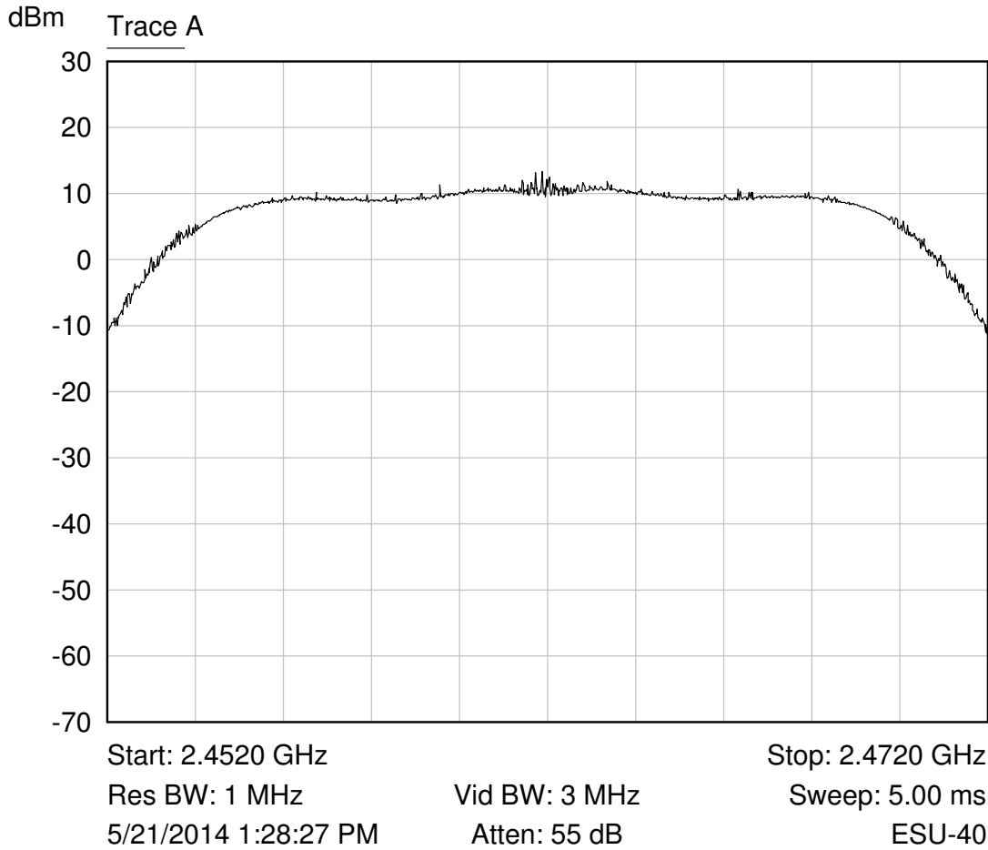
Trace A 802.11g +14 power setting
