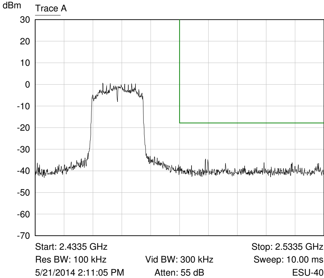
Trace A 802.11n +14 power setting
