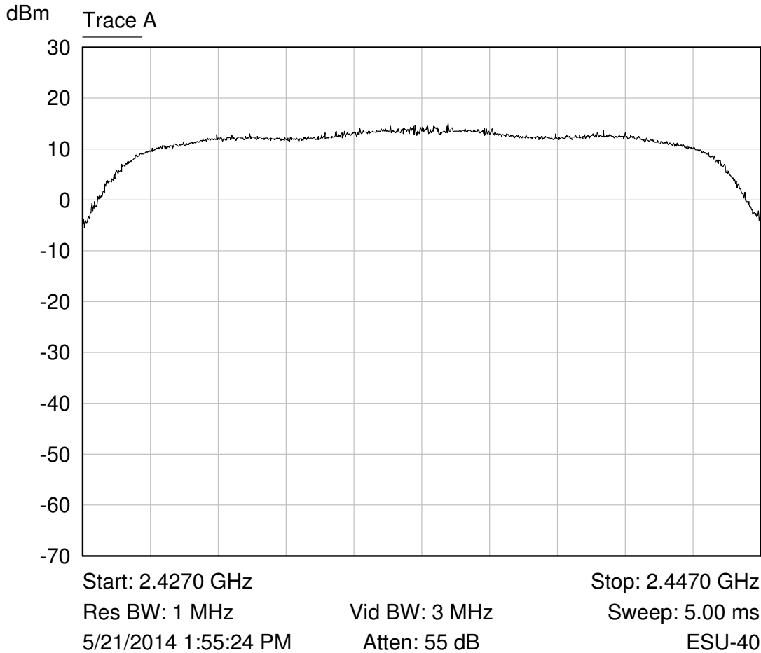
Trace A 802.11n +17 power setting
