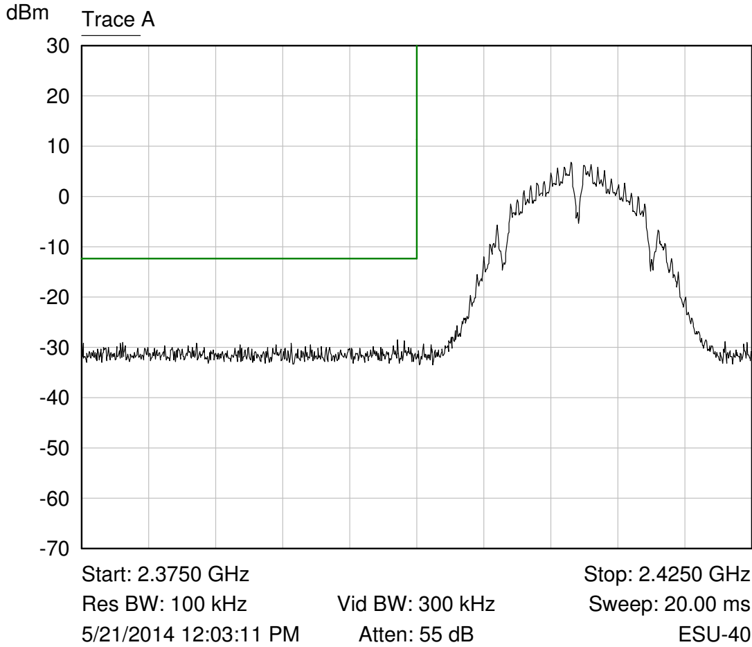
Trace A 802.11b +16 power setting
