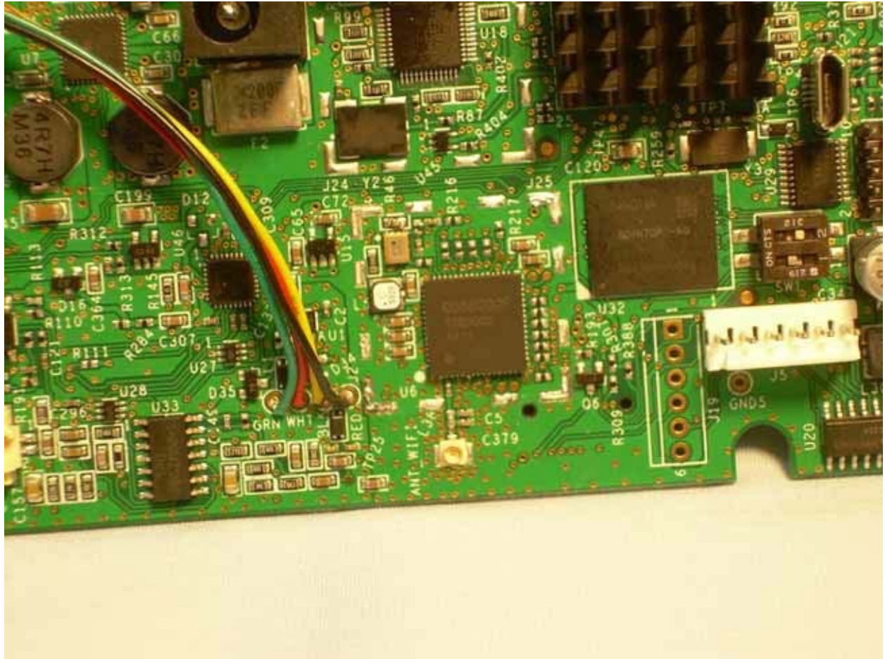
View of the Back Side of the Main PCB Circuitry with RF Shield Removed
