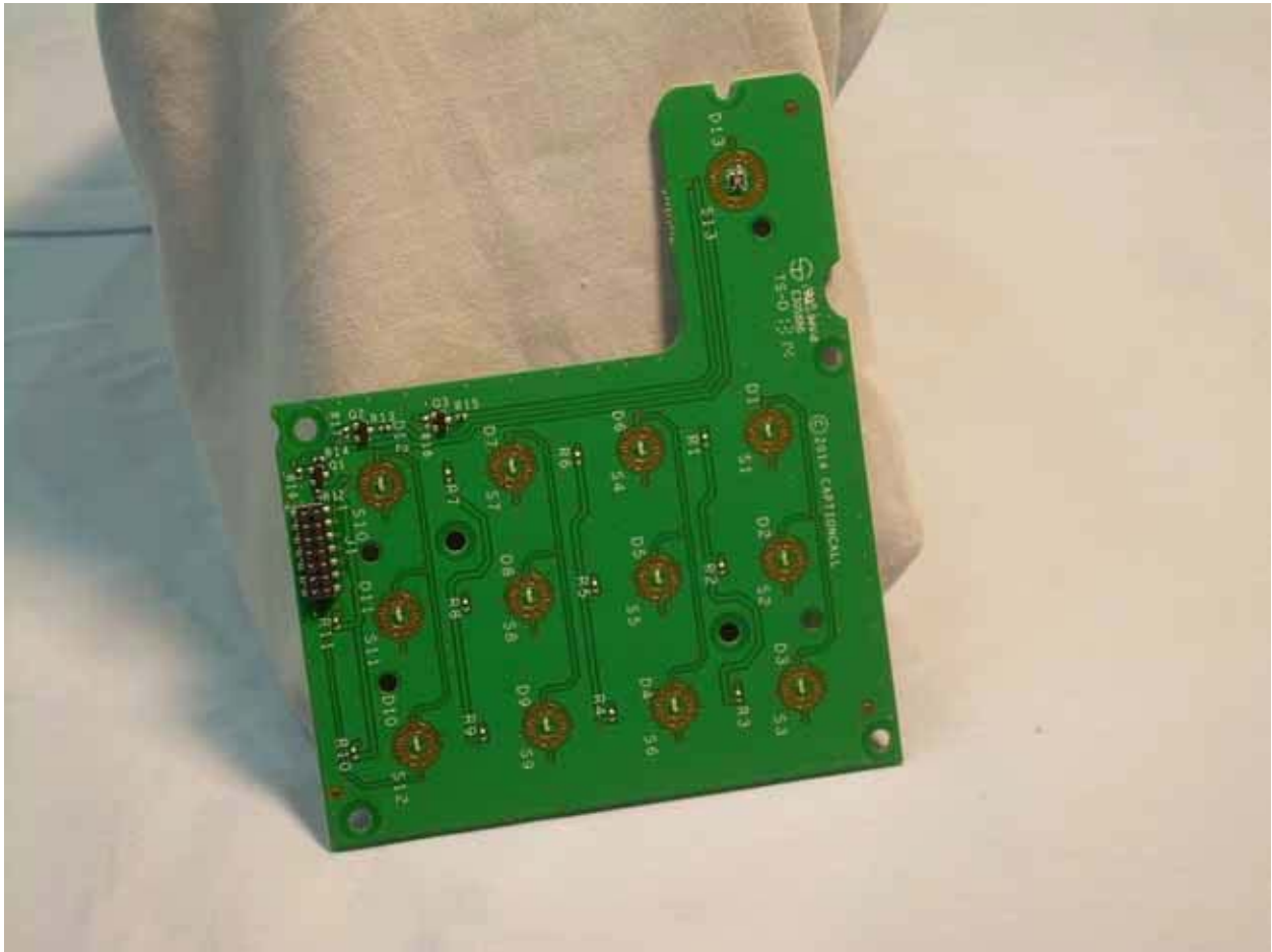
View of the Front Side of the Button Interface PCB
