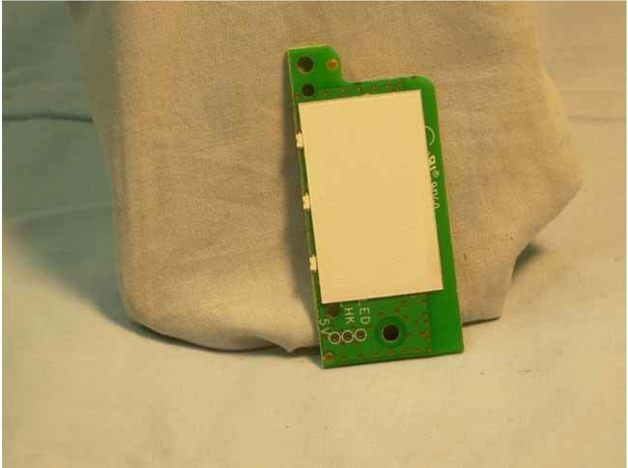
View of the Front Side of the Antenna PCB
