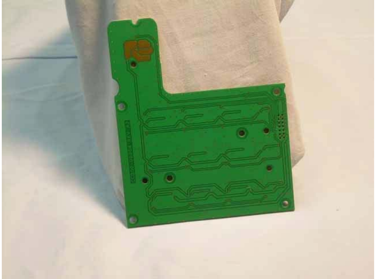
View of the Back Side of the Button Interface PCB
