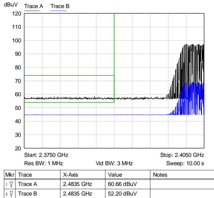
Graph 14: Lower Band Edge Plot While Hopping
