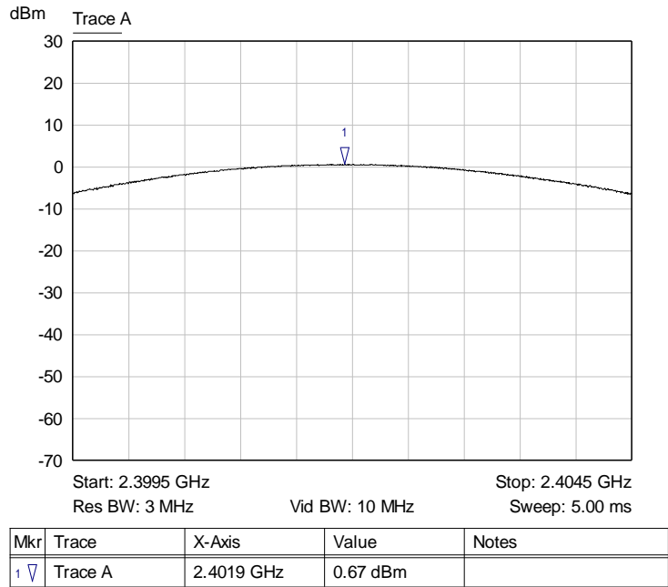
Graph 22: Transmitting at the Lowest Channel
