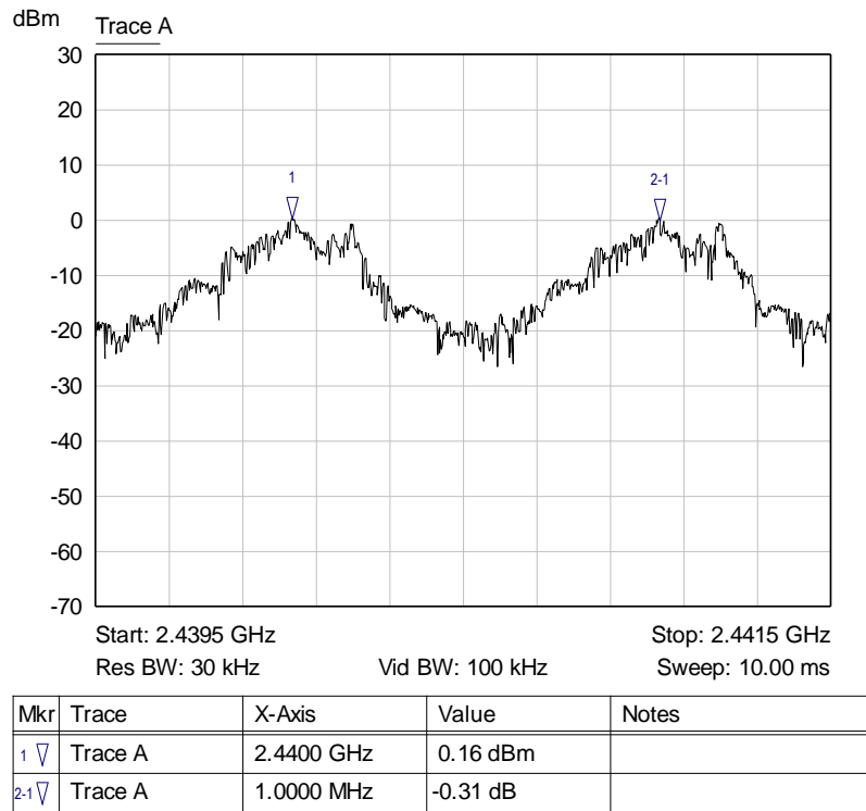
Graph 1: Channel Separation Plot
