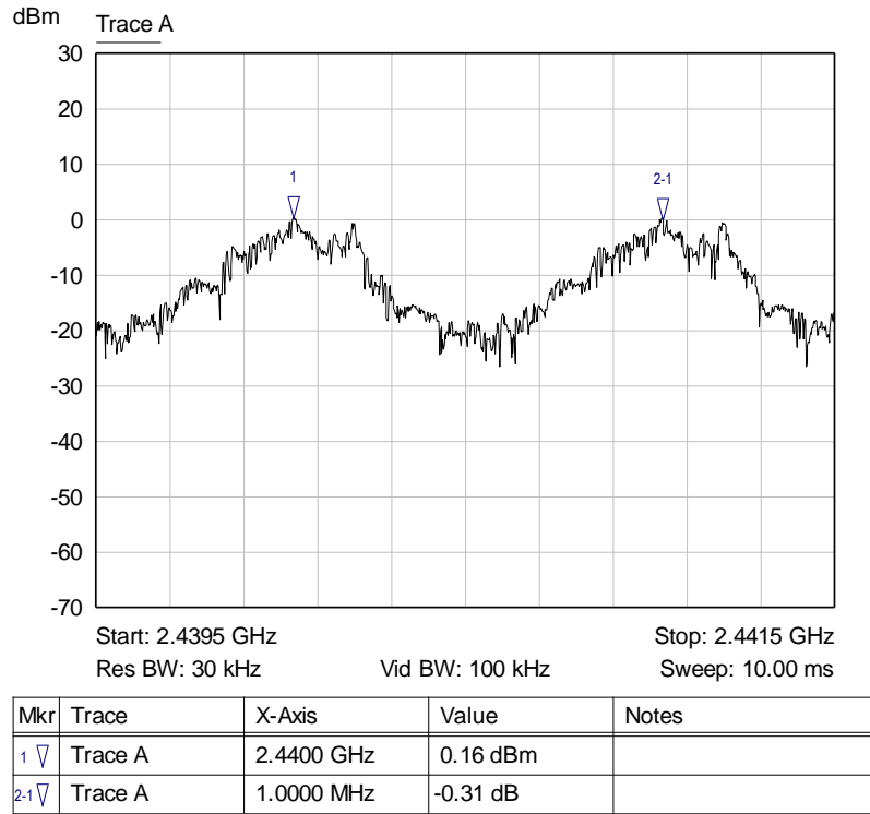
Graph 16: Channel Separation Plot
