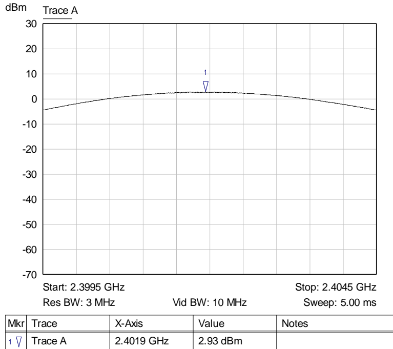
Graph 7: Transmitting at the Lowest Channel
