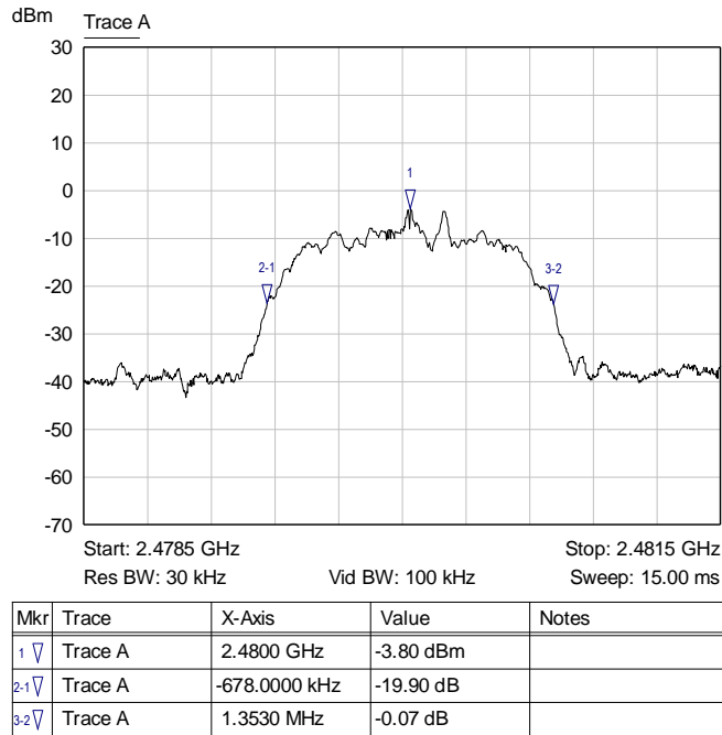
Graph 19: Highest Channel 20 dB Bandwidth
