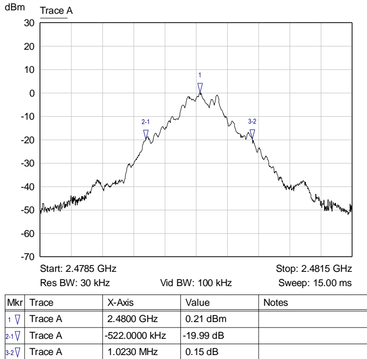
Graph 4: Highest Channel 20 dB Bandwidth
