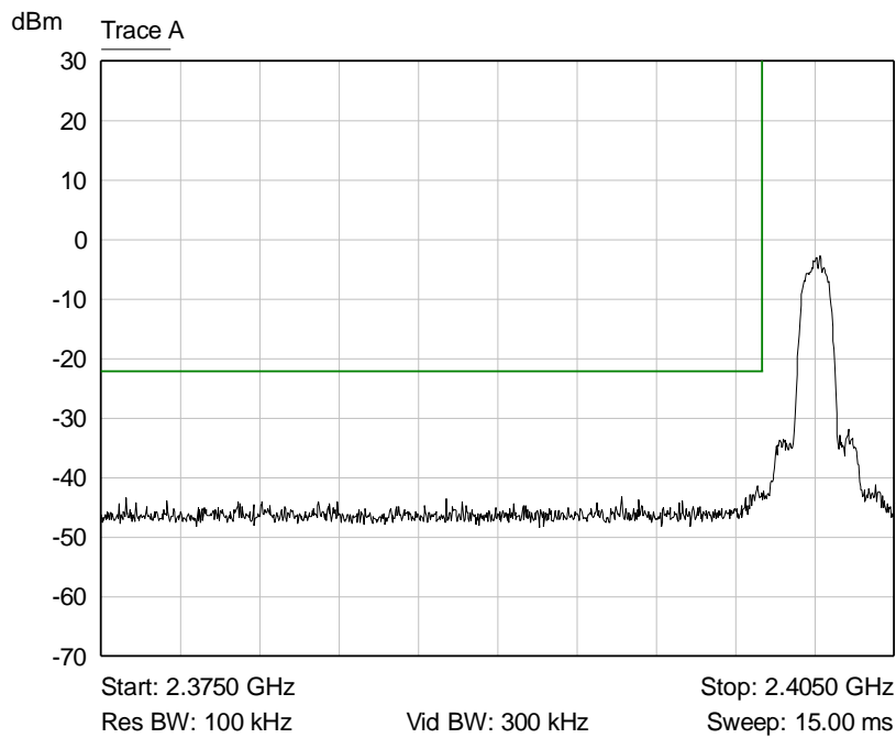
Graph 25: Lower Channel Plot
