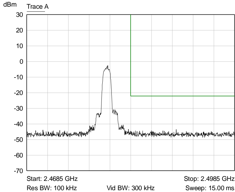
Graph 26: Upper Channel Plot
