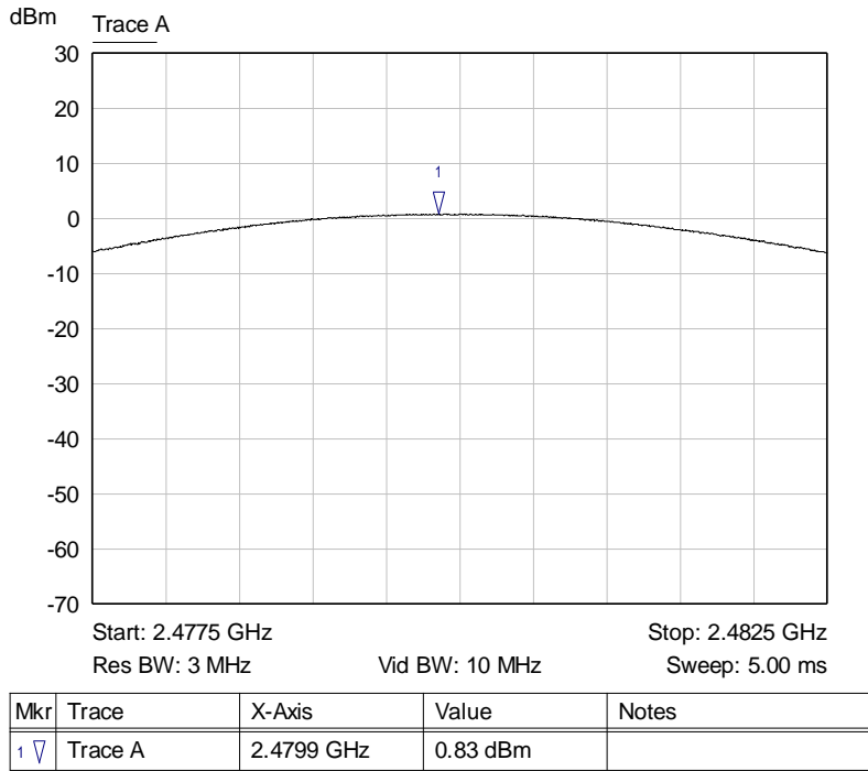
Graph 24: Transmitting at the Highest Channel
