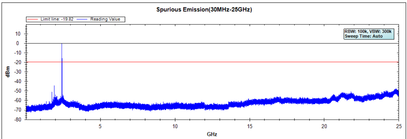
Channel 11 (2462MHz) 30MHz -25GHz
