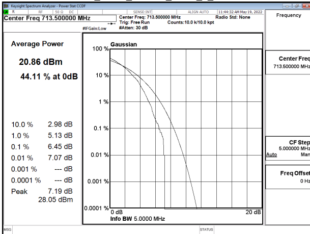
Band12_5MHz_64QAM_RB25_0_CH23155
