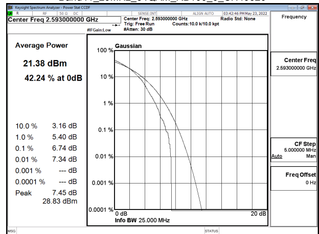
Band41_20MHz_64QAM_RB100_0_CH40620
