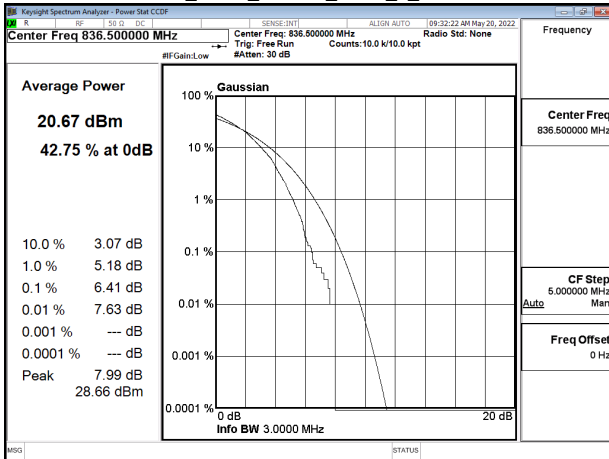
Band26_3MHz_64QAM_RB15_0_CH26915
