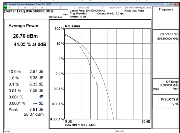
Band26_1.4MHz_64QAM_RB6_0_CH26915
