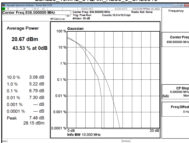
Band26_10MHz_64QAM_RB50_0_CH26915
