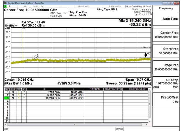
Band4_3MHz_QPSK_RB1_0_CH20385
