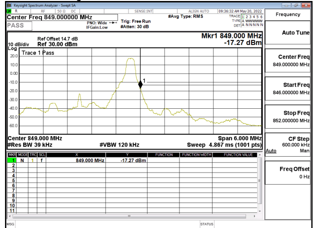
Band Edge_Band26_3MHz_QPSK_RB15_0_CH26805
