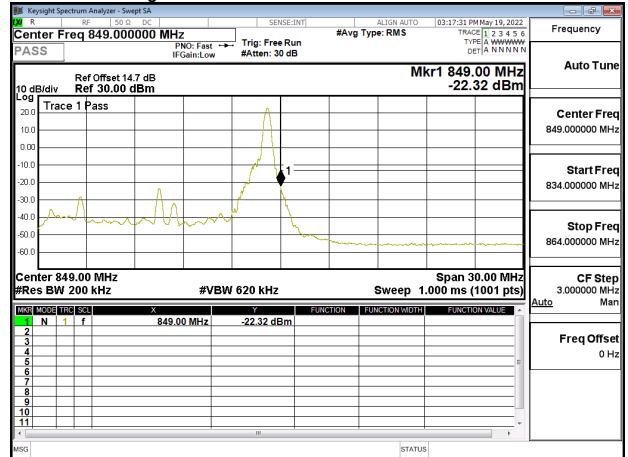
Band Edge_Band26_15MHz_QPSK_RB75_0_CH26865
