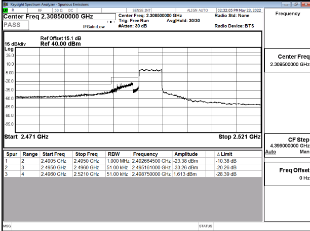
Emission Mask_Band41_5MHz_QPSK_RB25_0_CH39675
