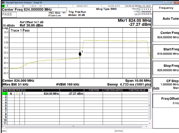
Band Edge_Band26_5MHz_QPSK_RB25_0_CH26815
