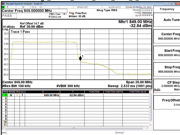
Band Edge_Band26_15MHz_QPSK_RB1_0_CH26865
