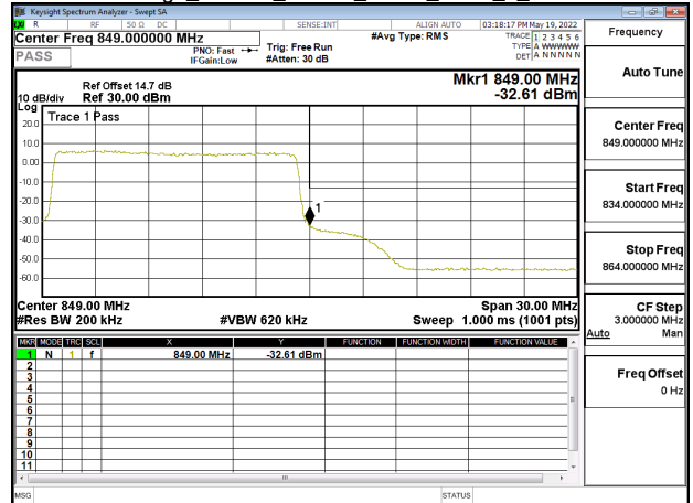
Band Edge_Band26_15MHz_QPSK_RB75_0_CH26965
