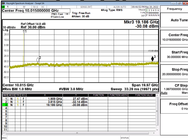
Band2_1.4MHz_QPSK_RB1_0_CH19193
