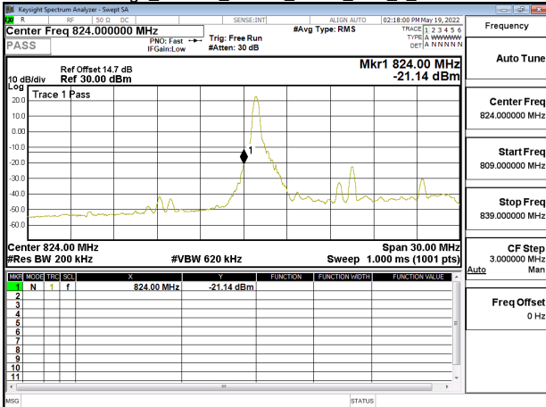
Band Edge_Band26_15MHz_QPSK_RB1_0_CH26865
