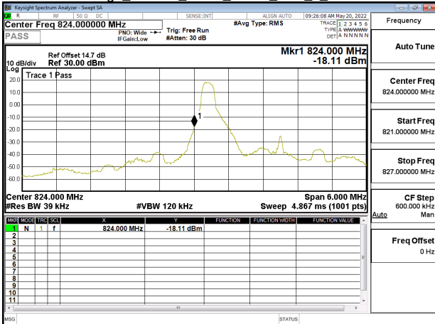
Band Edge_Band26_3MHz_QPSK_RB1_0_CH26805
