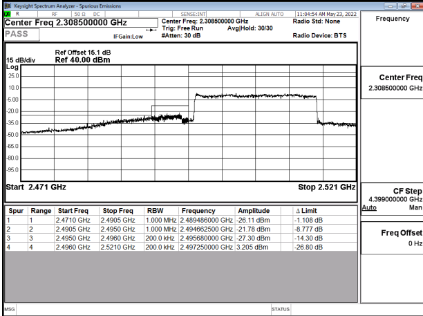
Emission Mask_Band41_20MHz_QPSK_RB100_0_CH39750
