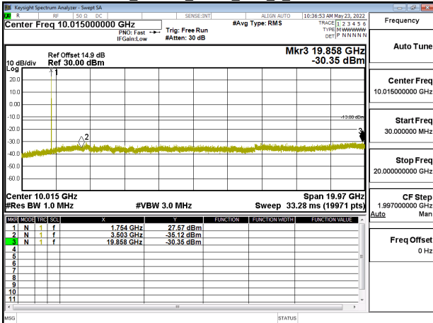
Band4_1.4MHz_QPSK_RB1_0_CH20393
