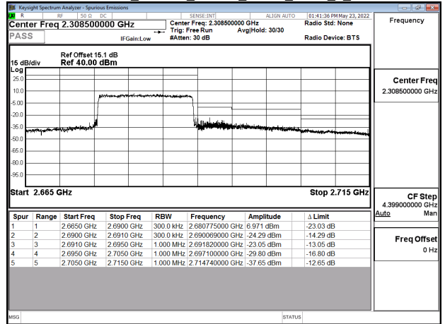
Emission Mask_Band41_15MHz_QPSK_RB75_0_CH41515
