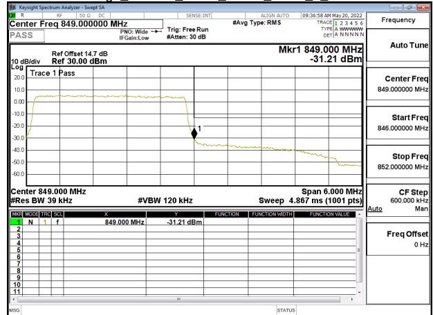
Band Edge_Band26_3MHz_QPSK_RB15_0_CH27025
