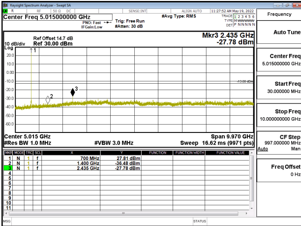
Band12_5MHz_QPSK_RB1_0_CH23095
