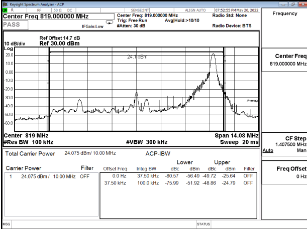
Emission Mask_Band26-Part90s_10MHz_QPSK_RB1_49_CH26740
