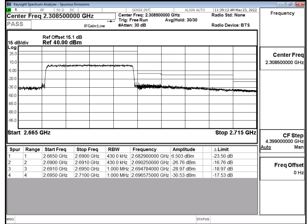
Emission Mask_Band41_20MHz_QPSK_RB100_0_CH41490
